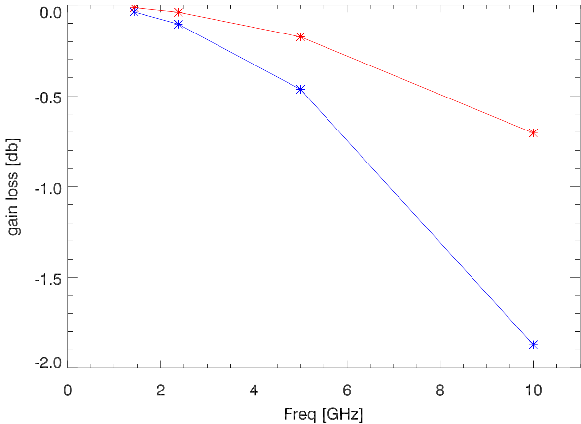
Gain loss Vs Freq (if radius 7.0cm short)
