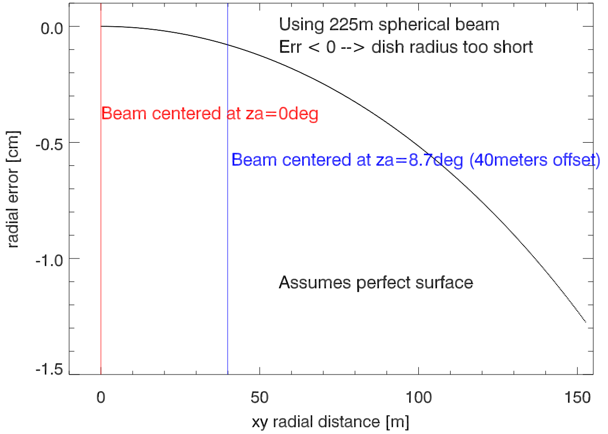
Radial error vs xy radius if dish radius 7.0cm short
