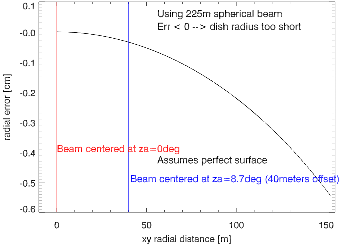
Radial error vs xy radius if dish radius 3.0cm short
