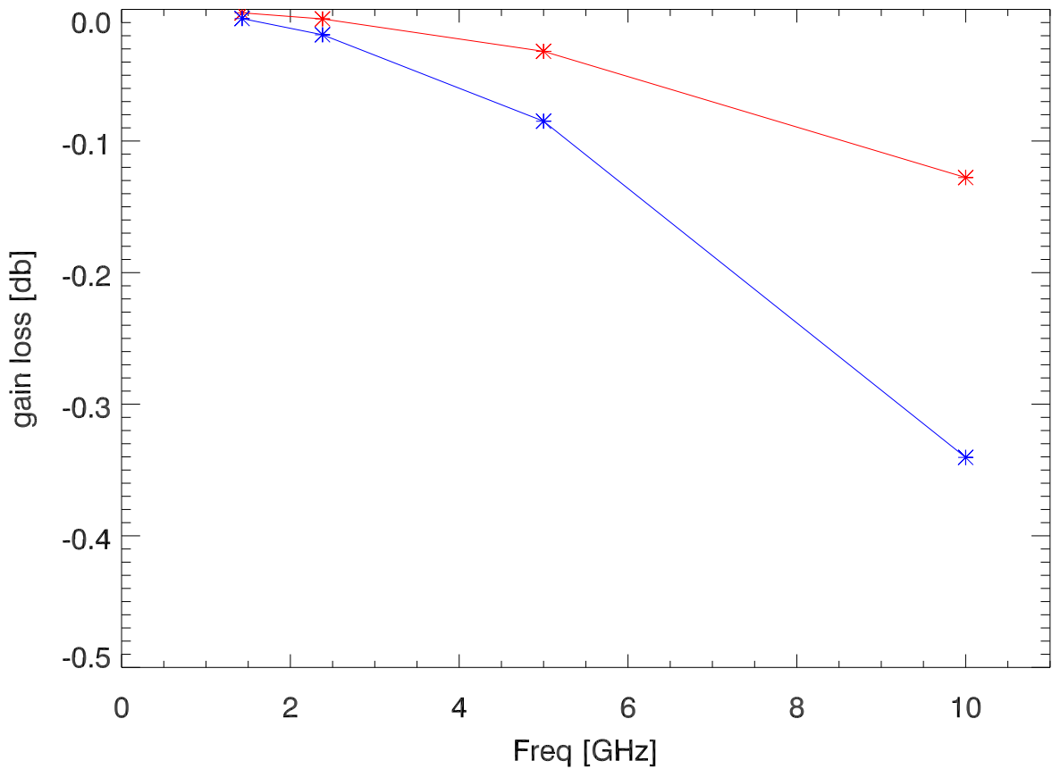
Gain loss Vs Freq (if radius 3.0cm short)
