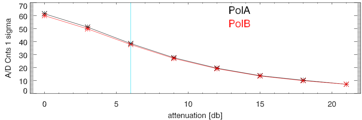
rms (in A/D cnts) vs attenuation
