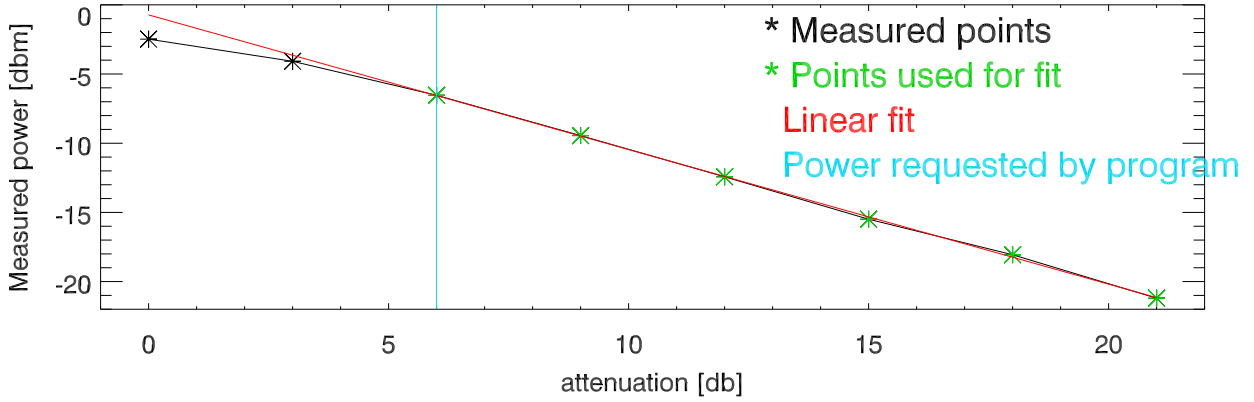
161027 jplDigRvr,Xband. cwcDRVC reported power vs attenuation. PoIA
