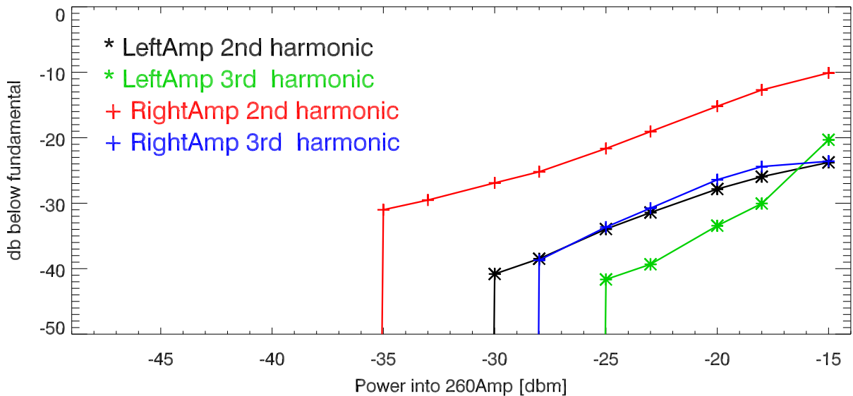
harmonic level below fundamental vs input power
