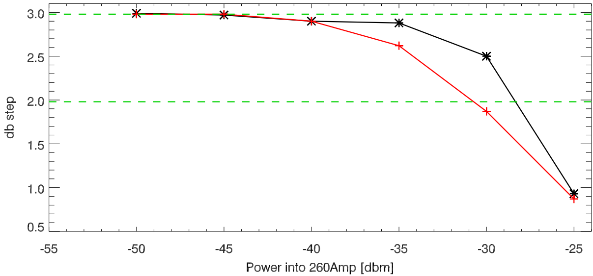
3db step of fundamental vs input power
