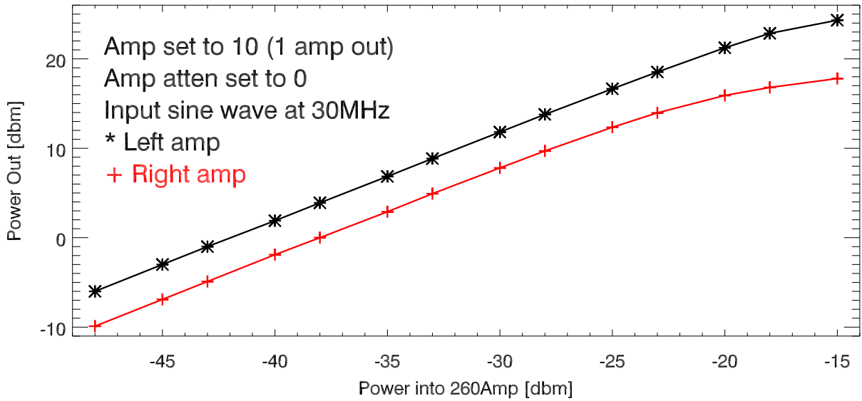
14feb20 test linearity rcvrRoom 260Mhz Amps
