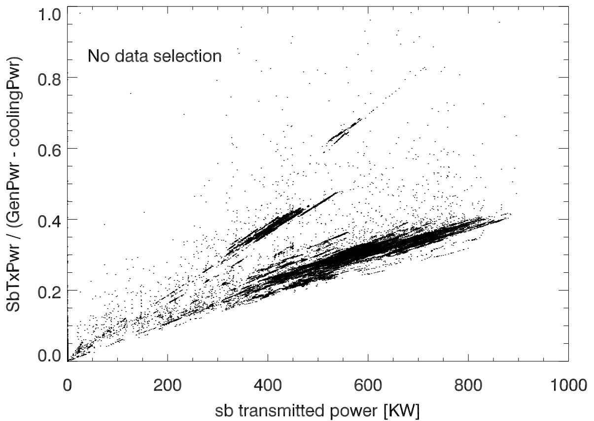
TxPower / (GenPower - coolingPower)
