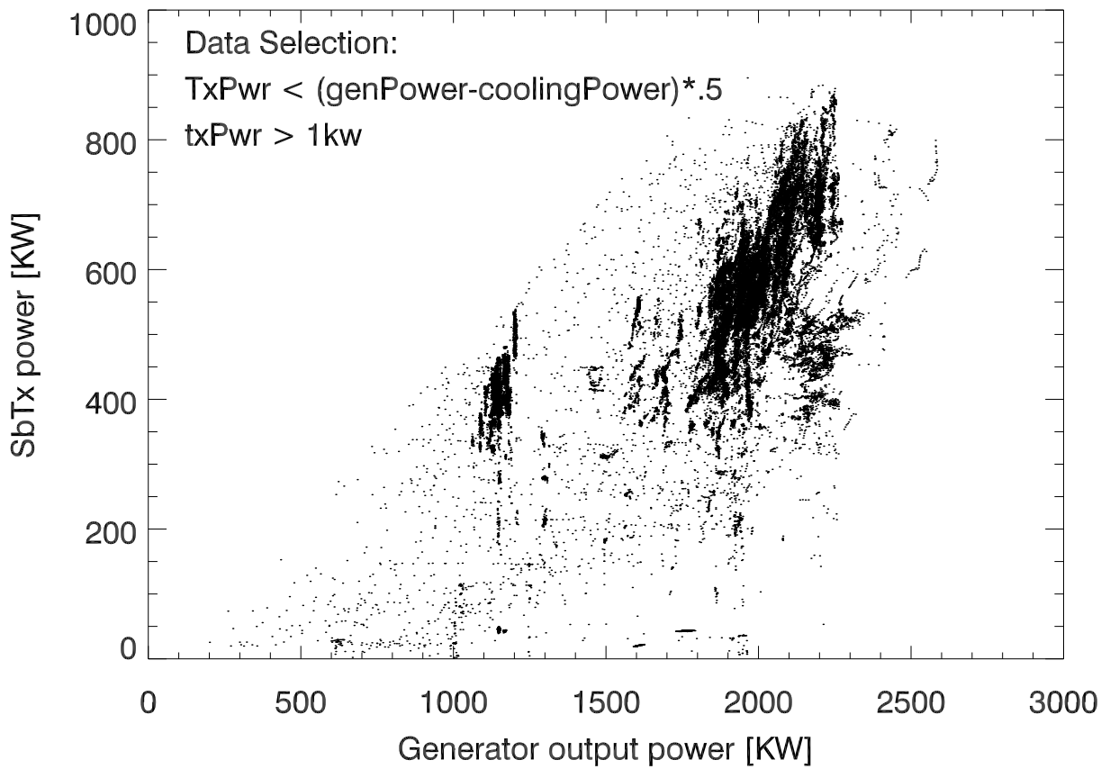
2017 sbTx power vs generator output power
