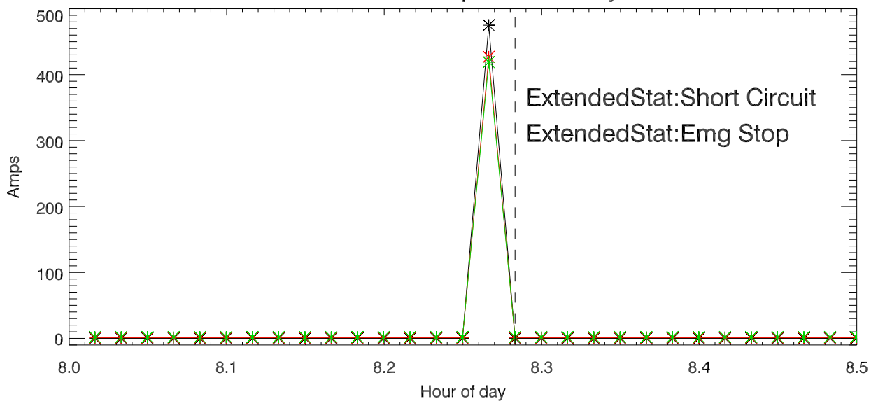
Gen4. Phase Amps vs hour of day
