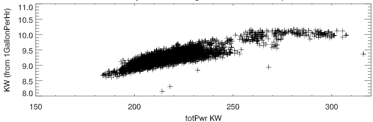
Efficiency: KW from 1 gallon/hour Vs total power
