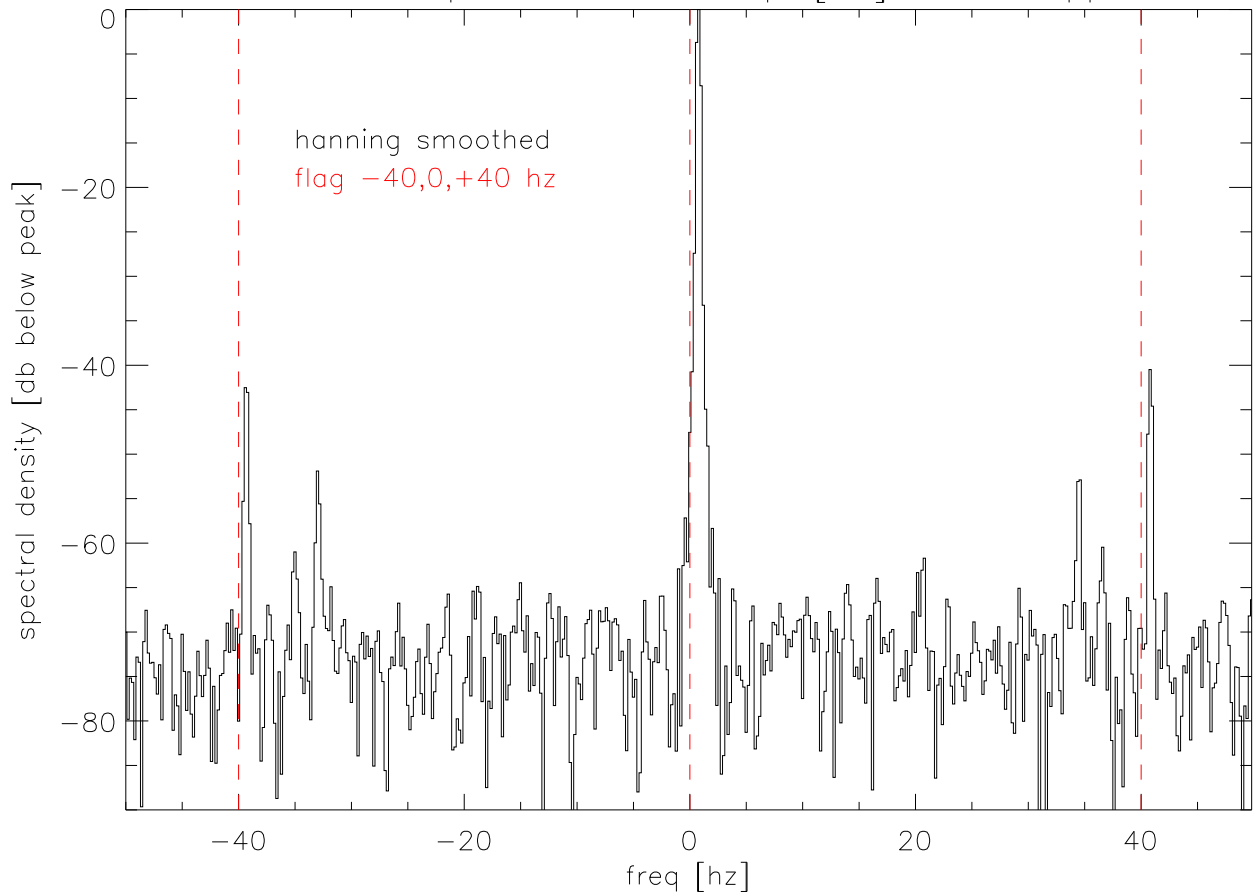
31mar06 Spectrum of txsample[86] for 500 ipp
