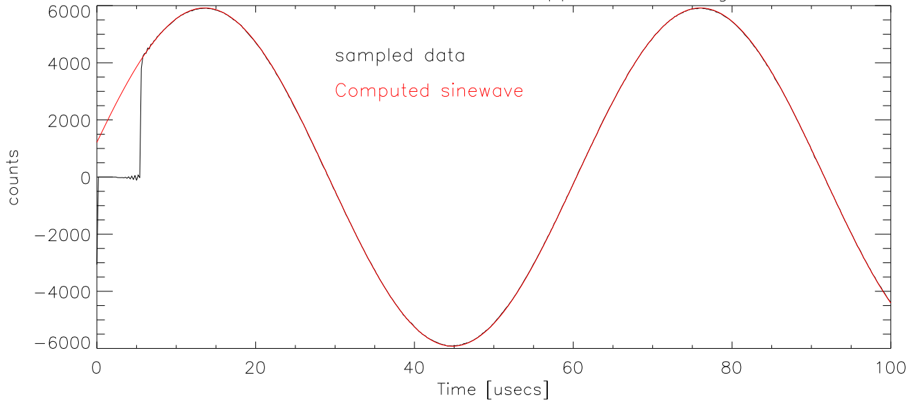
ipp 99 end of txWin, startDataWin. digitizer I
