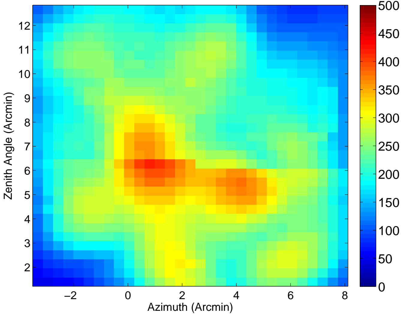
A6 Ae/Tsys Map ( z = 7.464 cm)
