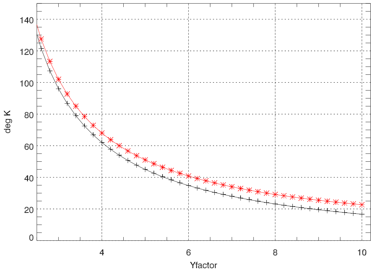
Trcv+Tspill vs Yfactor. Tsky=6K,Tmoon=210
