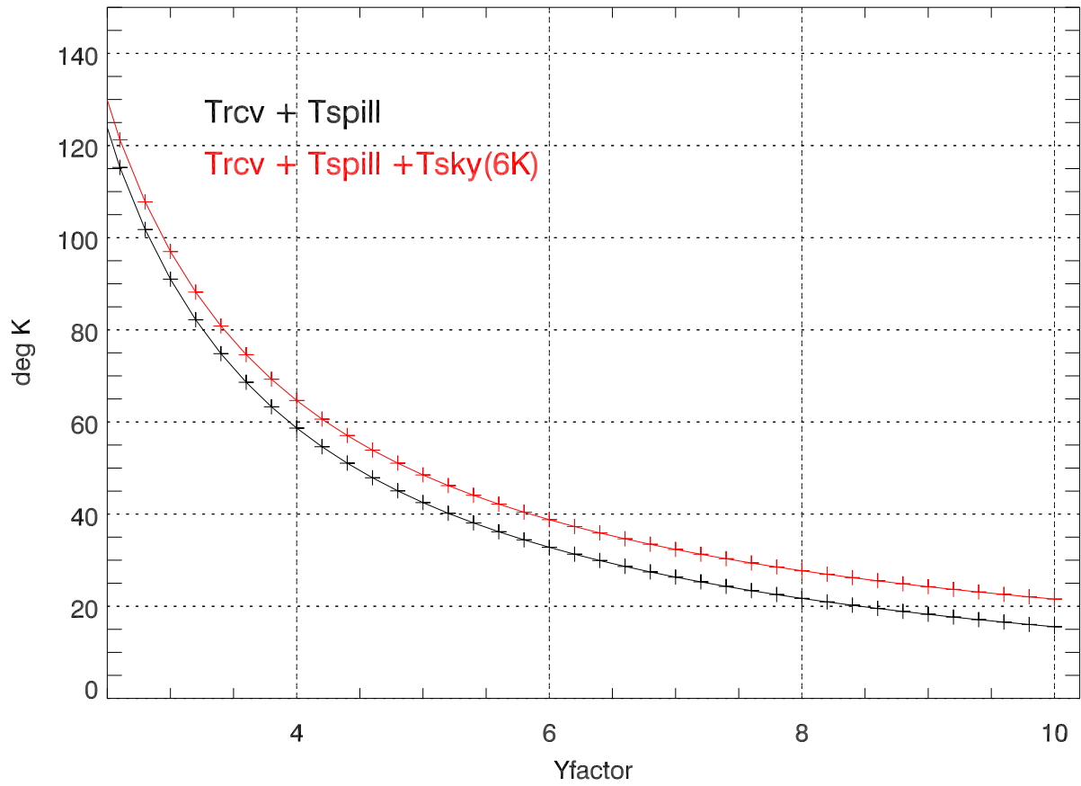
Trcv+Tspill vs Yfactor. Tsky=6K,Tmoon=200
