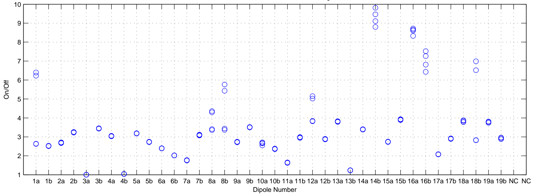
On/Off Y-Factors 1392.8711 MHz Dataset: /media/Disk0/08_02_2013_morning_moon
