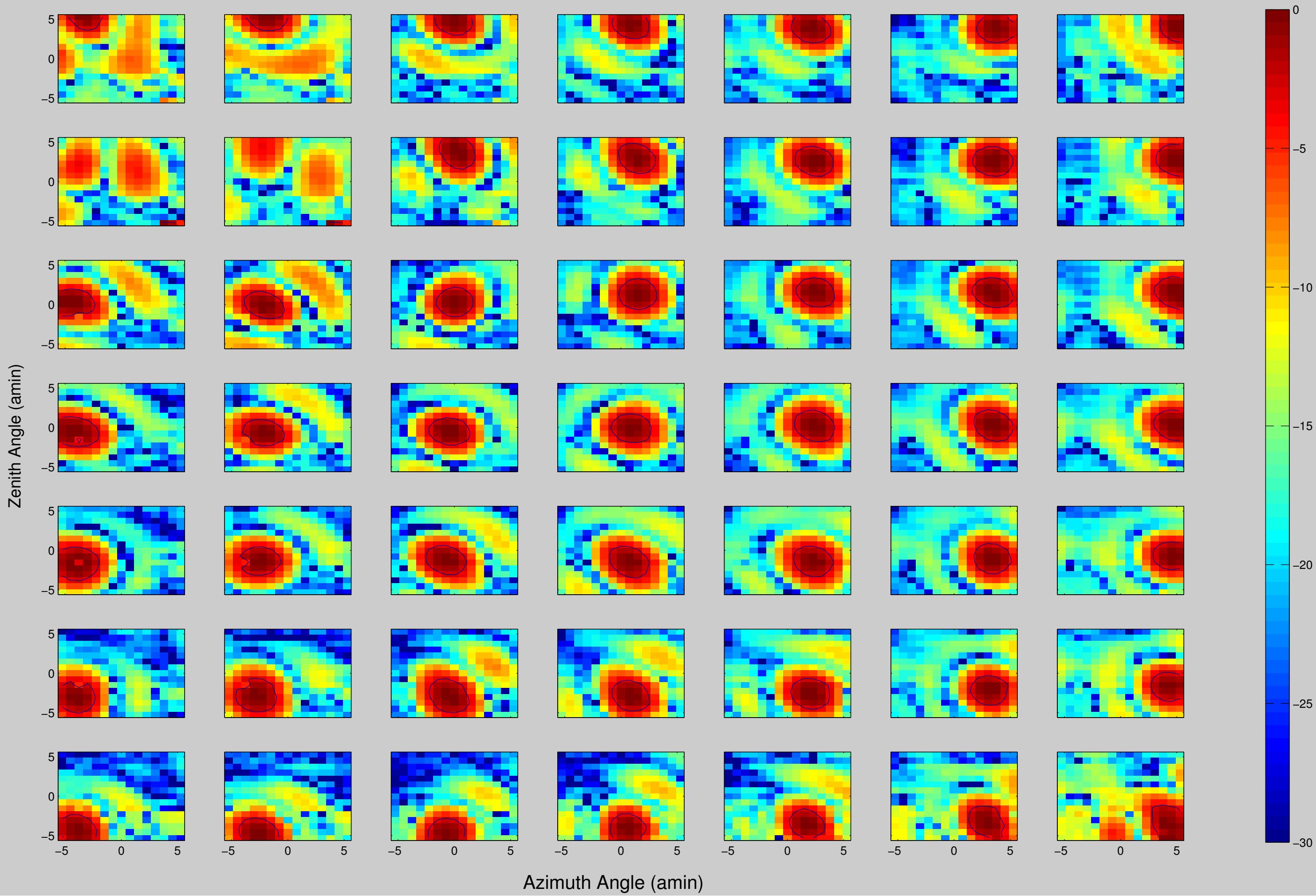
Formed Beams for Grid /media/Disk1/15x15_2013_07_23/default.mat, Frequency 1400.0977 MHz, Polarization B
