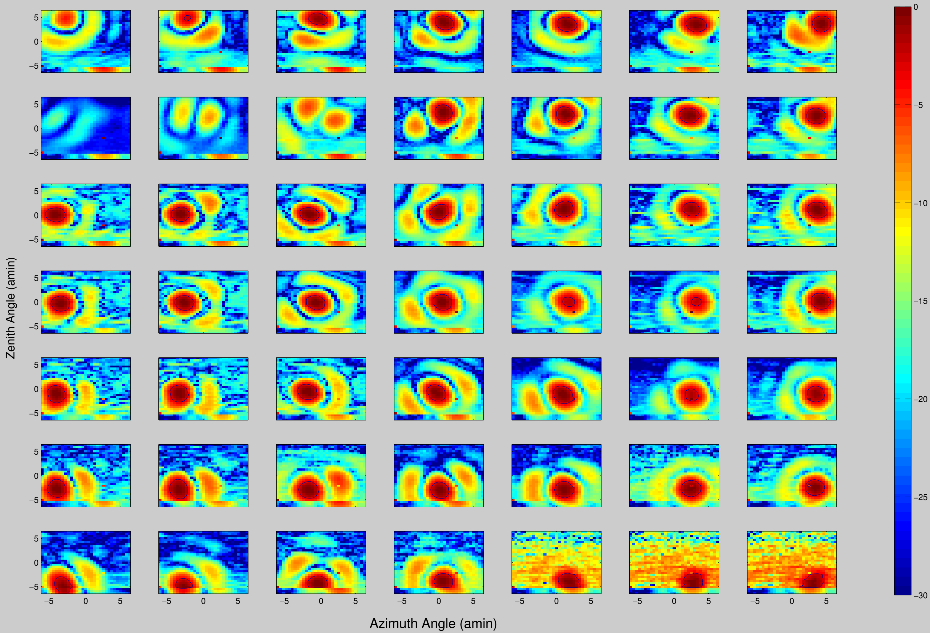
Formed Beams for Grid /media/Disk0/08_02_2013_evening_31x31/default.mat, Frequency 1664.707 MHz, Polarization B
