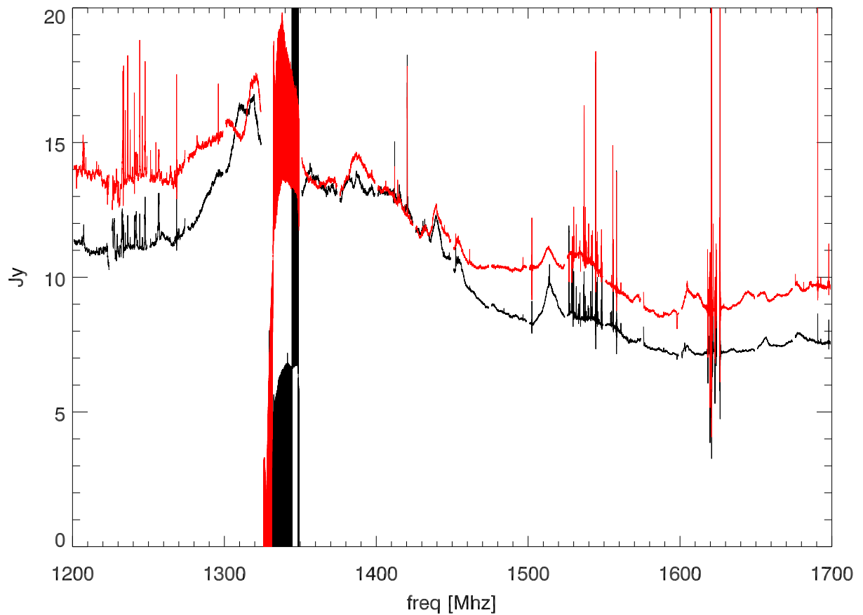
Average SEFD vs Frequency
