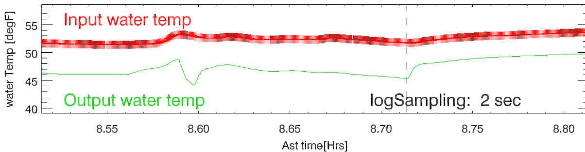
160427 bldll evaporator water temp vs time
