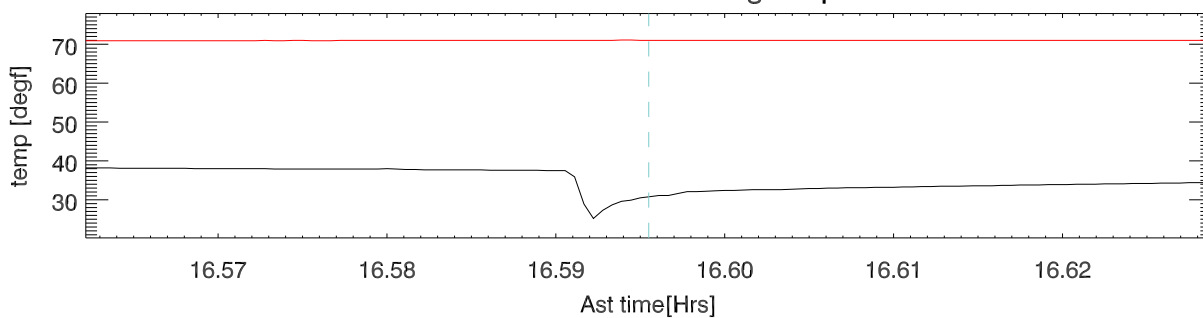
Suction saturated refriger temp
