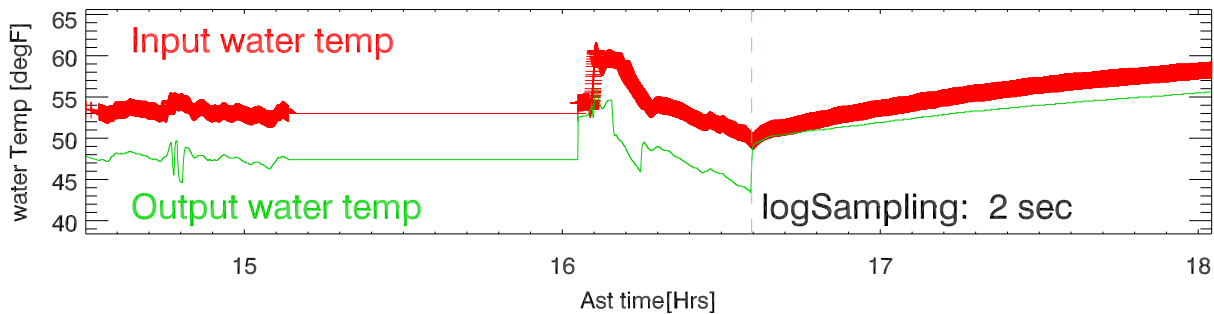
160419 bldll evaporator water temp vs time
