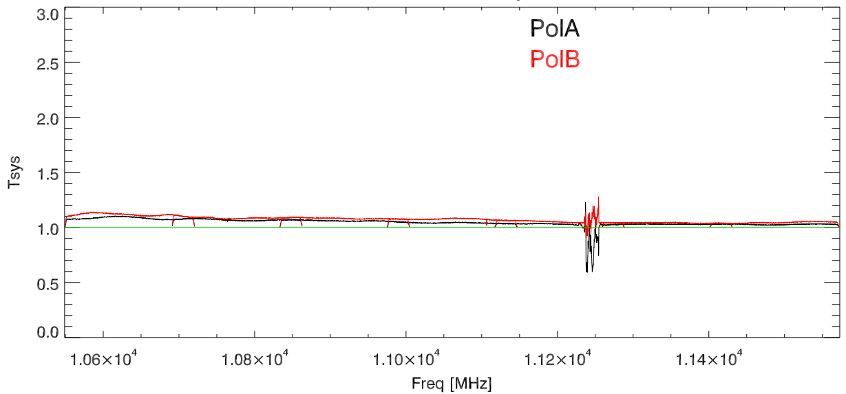
CalDeflection/Tsys
