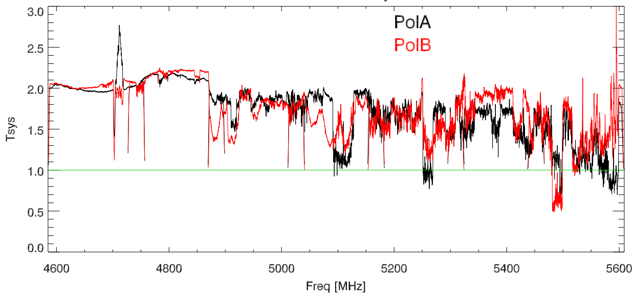
CalDeflection/Tsys
