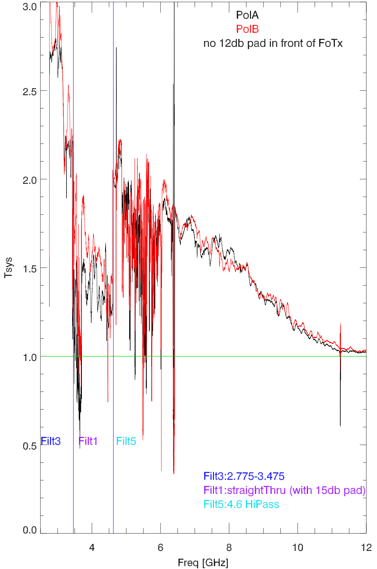
230529(Tsys+Tcal)/Tsys for all freq
