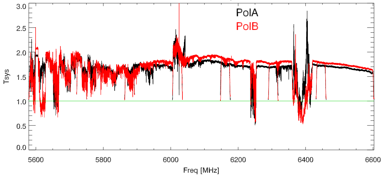
CalDeflection/Tsys
