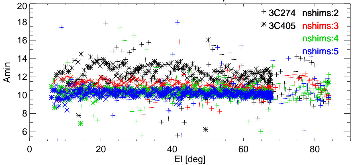
El BmWidth vs El for various shims. freq=8931 Pol:A RemoveBase.
