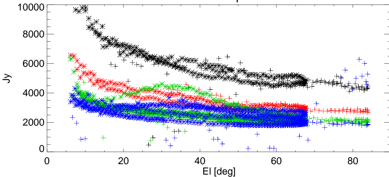
SEFD vs EI for various shims. freq=8931 Pol:B RemoveBase.
