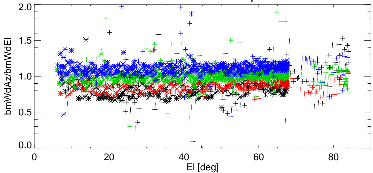
Az/EI BmWdRatio vs EI for various shims. freq=8931 Pol:B RemoveBase.
