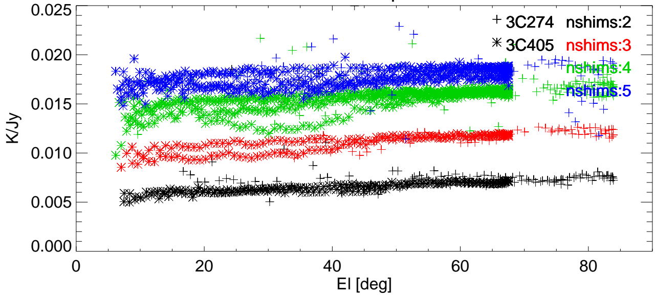
Gain vs EI for various shims. freq=8931 Pol:A RemoveBase.
