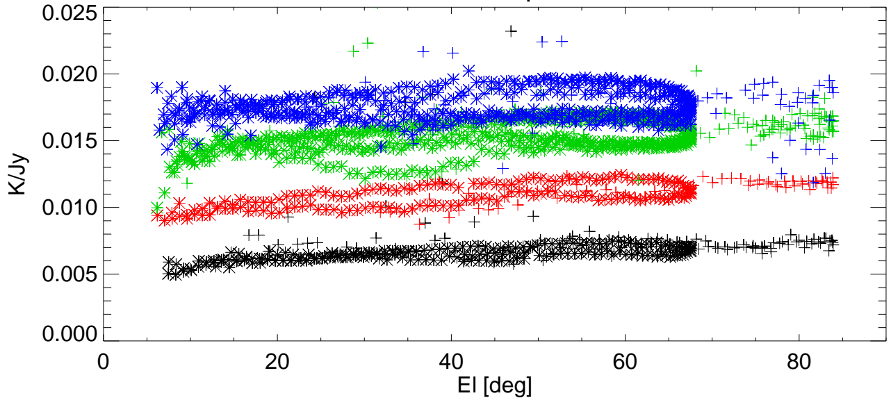
Gain vs EI for various shims. freq=8931 Pol:B RemoveBase.
