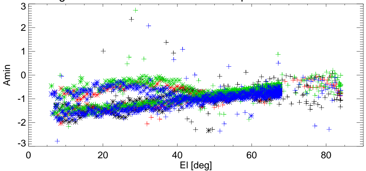
Az Pointing error vs EI for various shims. freq=8931 Pol:B RemoveBase.
