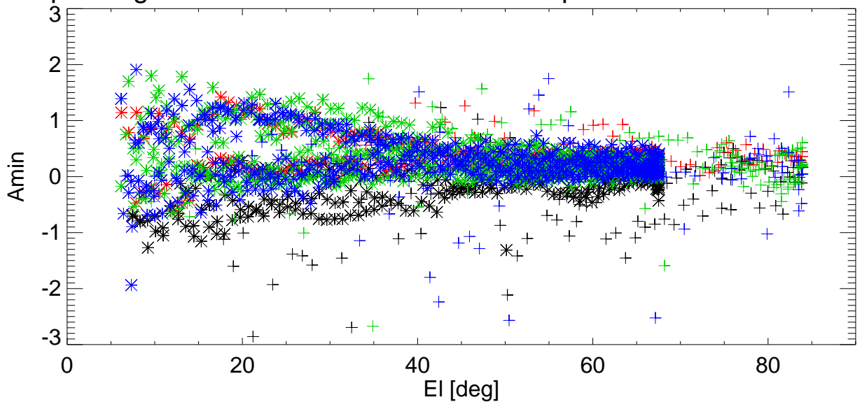
El pointing error vs El for various shims. freq=8931 Pol:B RemoveBase.
