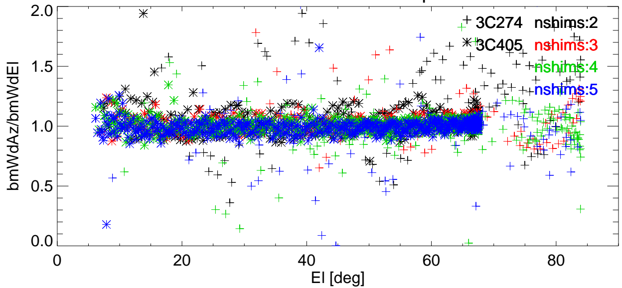
Az/EI BmWdRatio vs EI for various shims. freq=8931 Pol:A RemoveBase.
