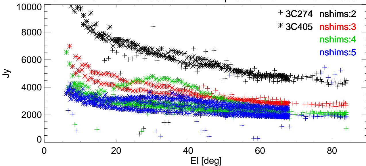
SEFD vs EI for various shims. freq=8931 Pol:A RemoveBase.
