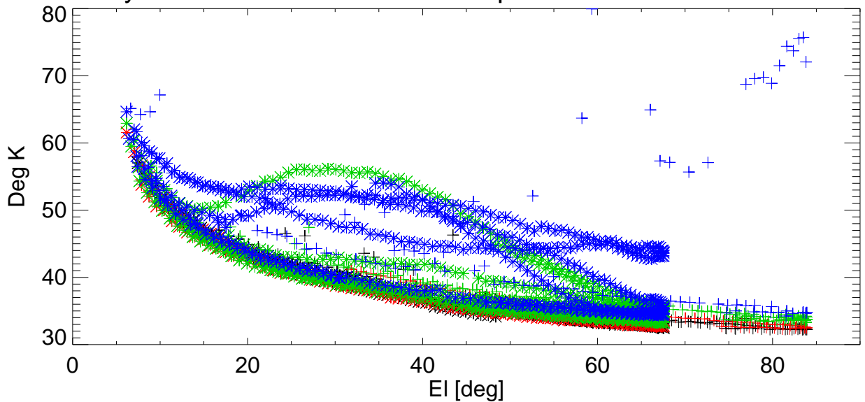
Tsys vs EI for various shims. freq=8931 Pol:B RemoveBase.
