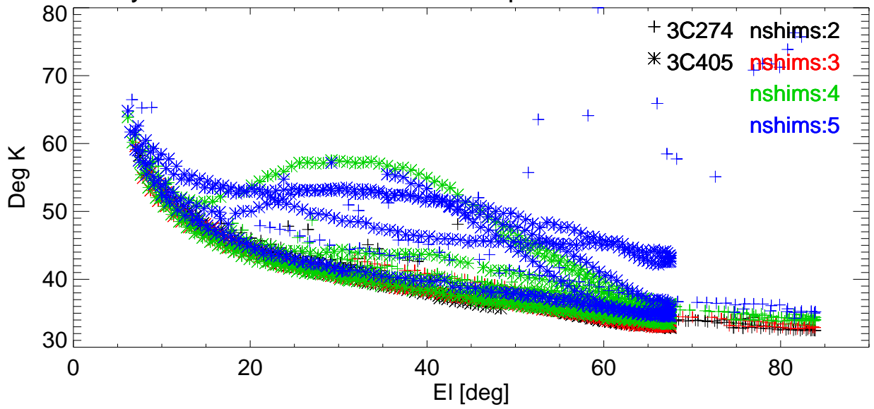
Tsys vs EI for various shims. freq=8931 Pol:A RemoveBase.
