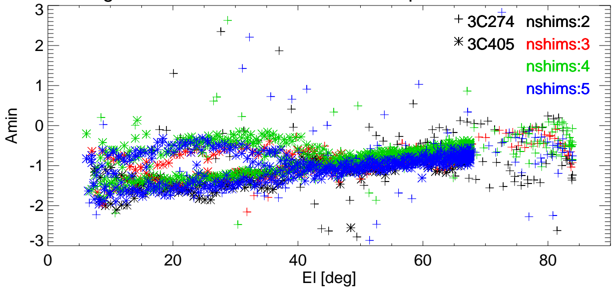
Az Pointing error vs EI for various shims. freq=8931 Pol:A RemoveBase.
