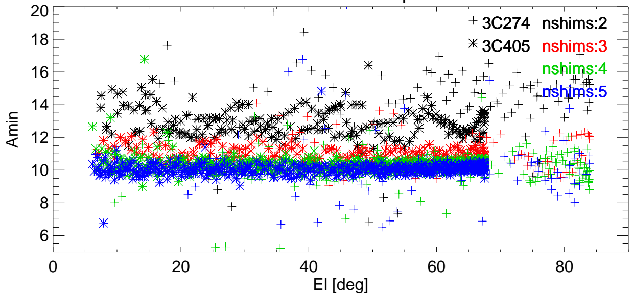
Az BmWidth vs EI for various shims. freq=8931 Pol:A RemoveBase.
