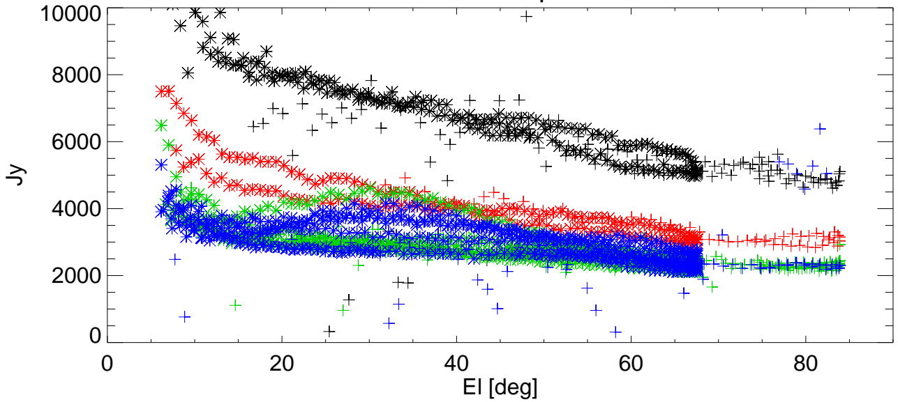
SEFD vs EI for various shims. freq=8647 Pol:B RemoveBase.
