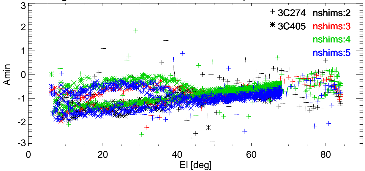
Az Pointing error vs EI for various shims. freq=8647 Pol:A RemoveBase.
