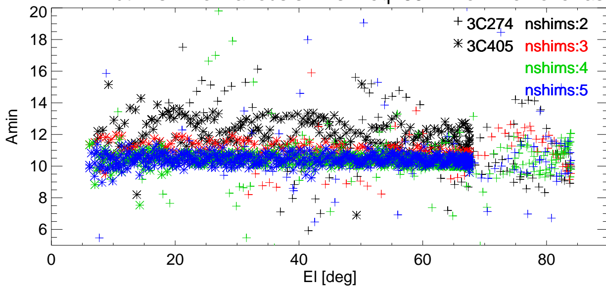
El BmWidth vs El for various shims. freq=8647 Pol:A RemoveBase.
