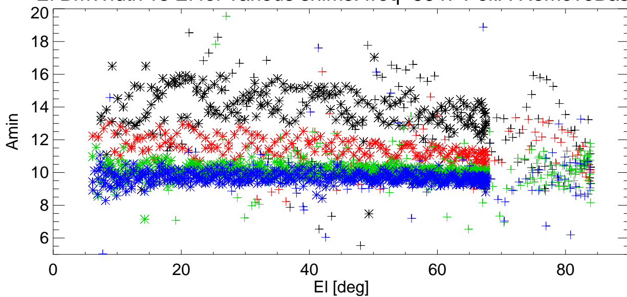
El BmWidth vs El for various shims. freq=8647 Pol:B RemoveBase.
