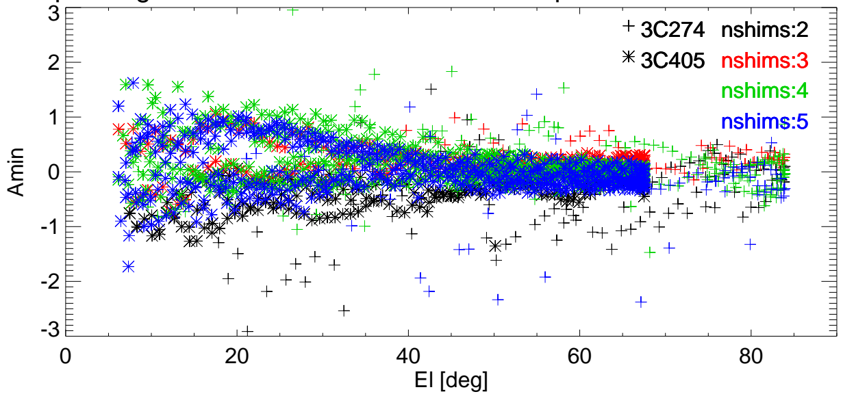
El pointing error vs El for various shims. freq=8647 Pol:A RemoveBase.
