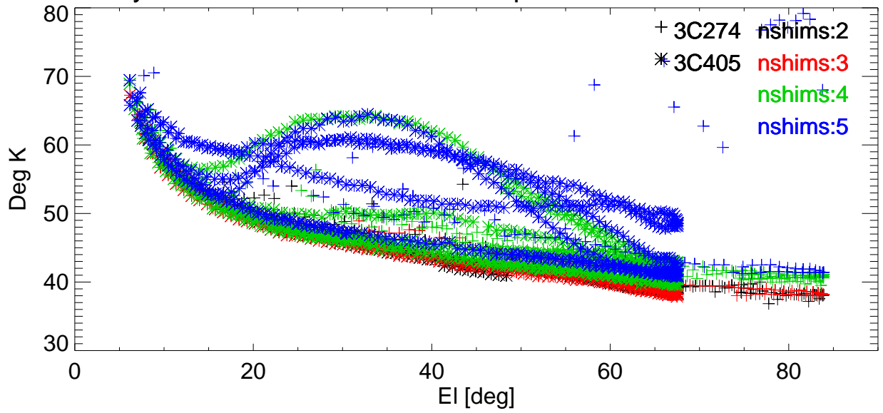
Tsys vs EI for various shims. freq=8647 Pol:A RemoveBase.
