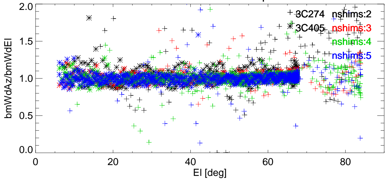
Az/EI BmWdRatio vs EI for various shims. freq=8647 Pol:A RemoveBase.
