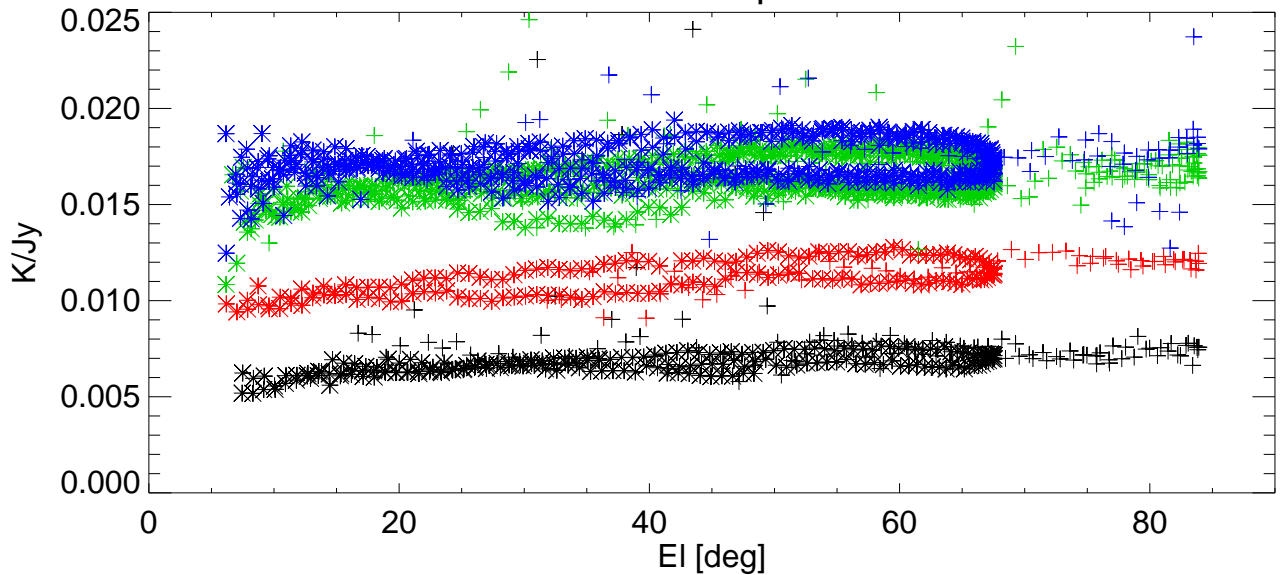
Gain vs EI for various shims. freq=8647 Pol:B RemoveBase.
