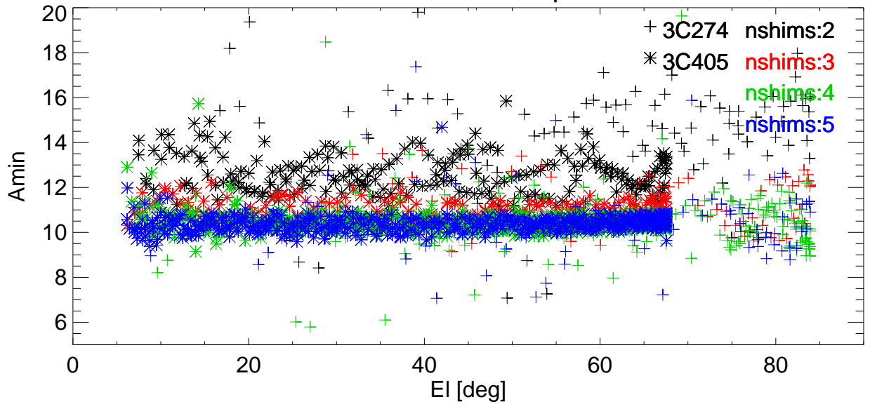
Az BmWidth vs EI for various shims. freq=8647 Pol:A RemoveBase.
