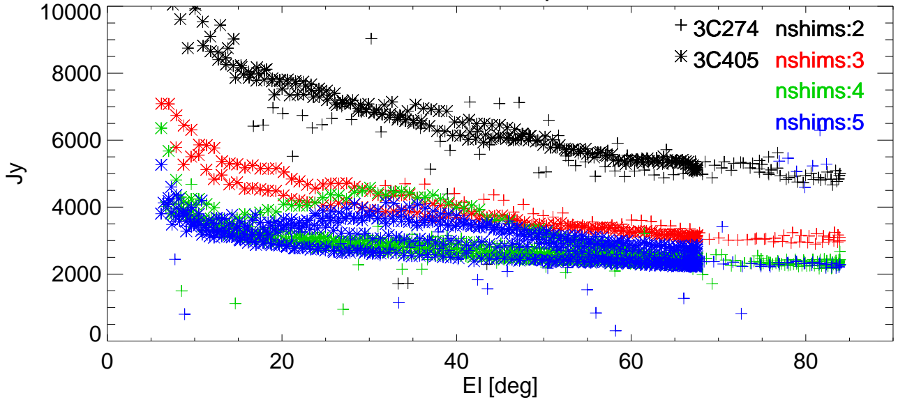
SEFD vs EI for various shims. freq=8647 Pol:A RemoveBase.
