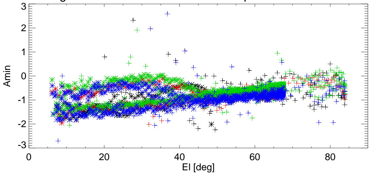
Az Pointing error vs EI for various shims. freq=8647 Pol:B RemoveBase.
