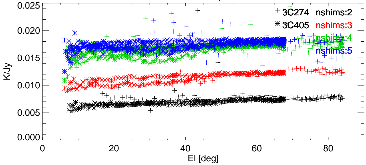
Gain vs EI for various shims. freq=8647 Pol:A RemoveBase.
