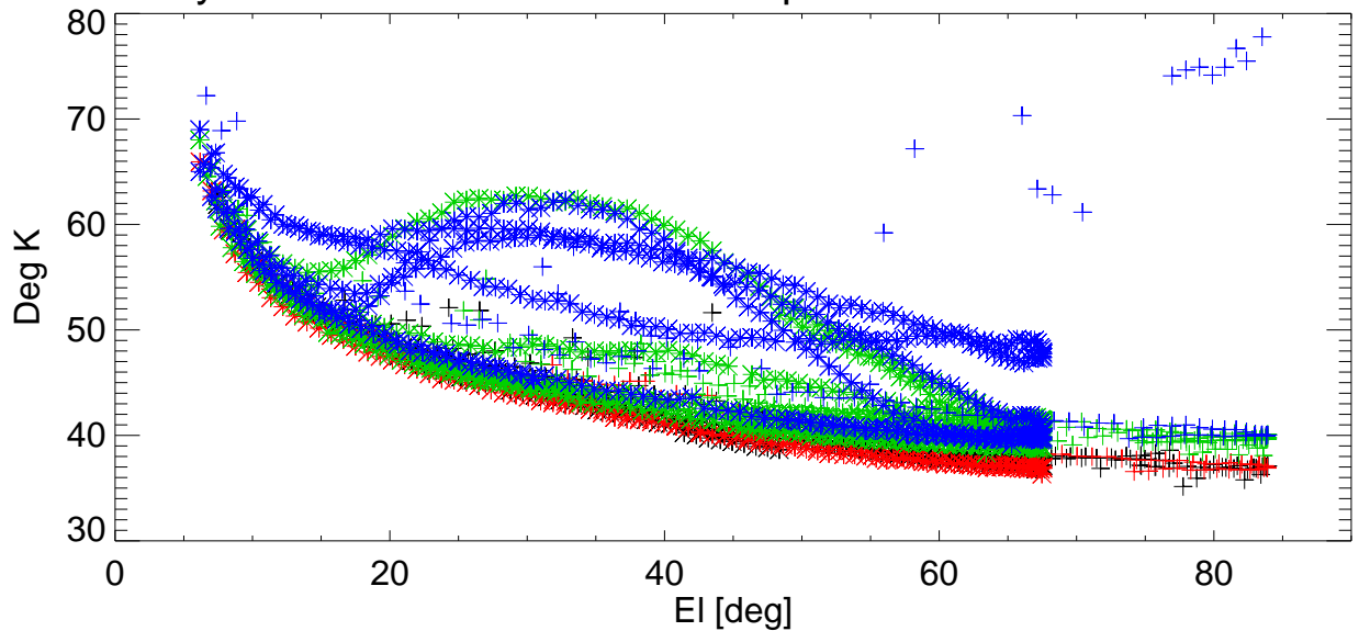
Tsys vs EI for various shims. freq=8647 Pol:B RemoveBase.
