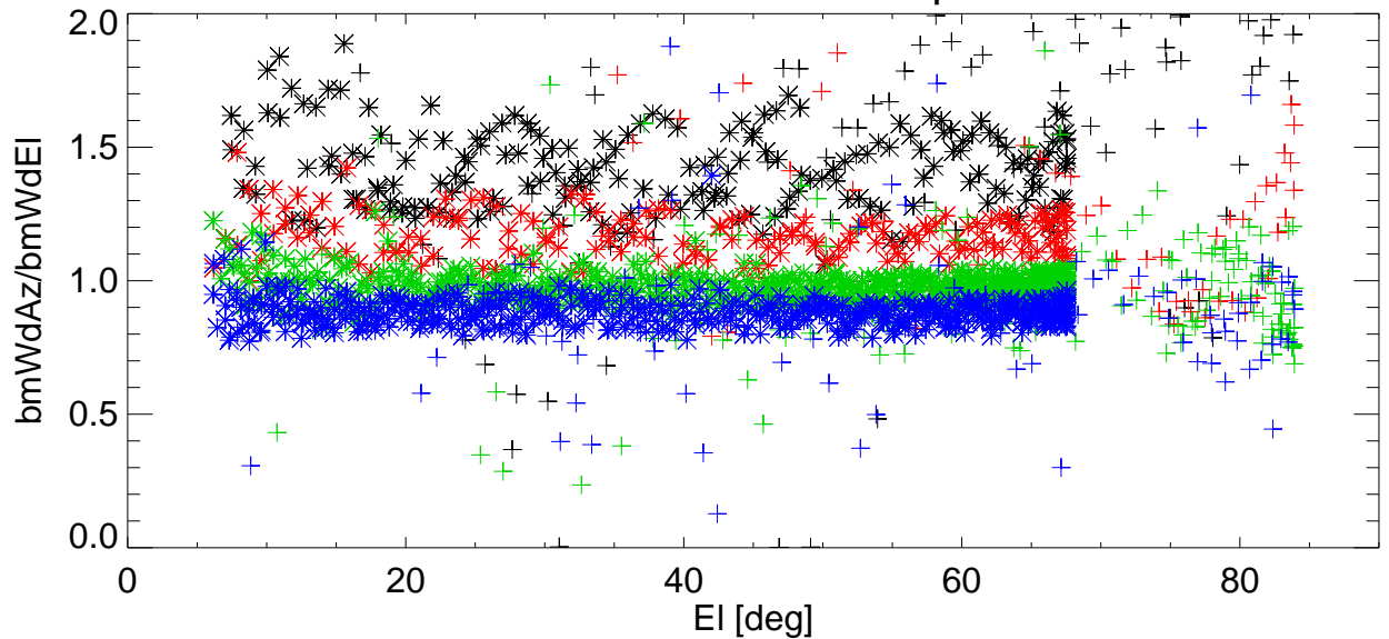
Az/EI BmWdRatio vs EI for various shims. freq=8647 Pol:B RemoveBase.
