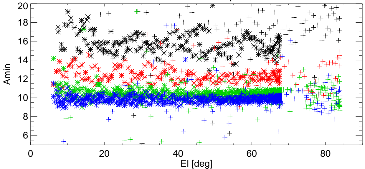
Az BmWidth vs EI for various shims. freq=8647 Pol:B RemoveBase.
