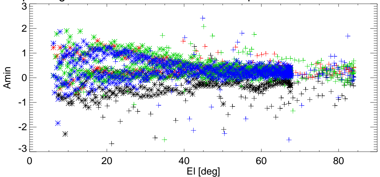
El pointing error vs El for various shims. freq=8647 Pol:B RemoveBase.
