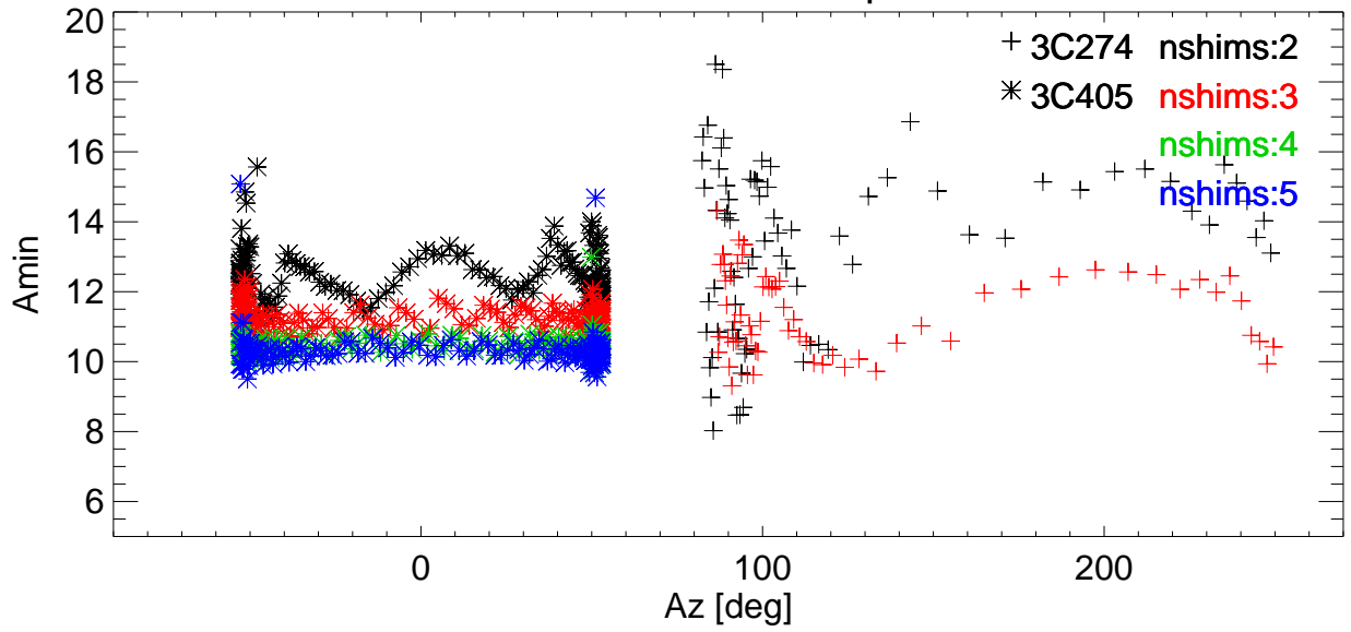
Az BmWidth vs Az for various shims. freq=8789 Pol:A RemoveBase.
