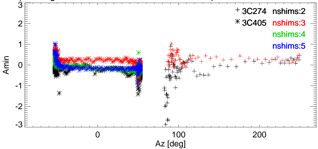
El pointing error vs Az for various shims. freq=8789 Pol:A RemoveBase.
