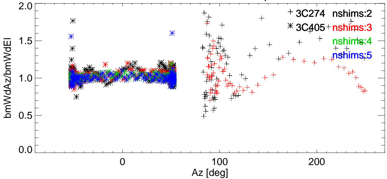
Az/EI BmWdRatio vs Az for various shims. freq=8789 Pol:A RemoveBase.
