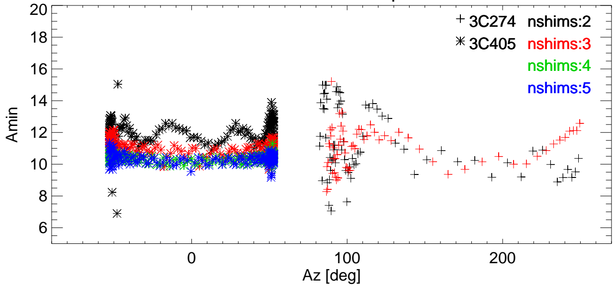
El BmWidth vs Az for various shims. freq=8789 Pol:A RemoveBase.
