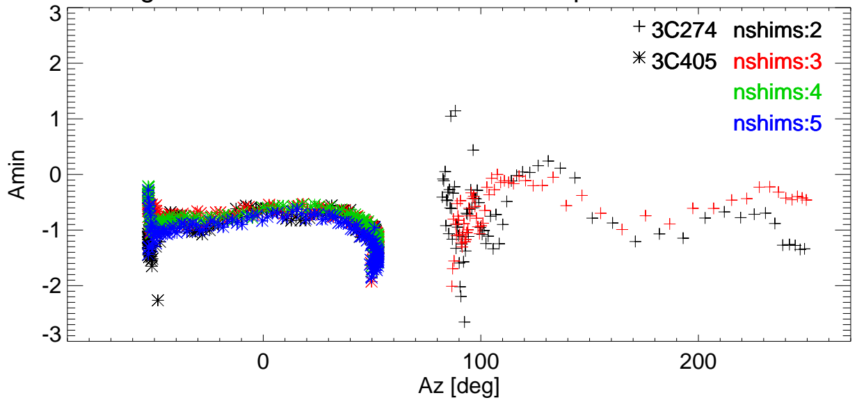
Az Pointing error vs Az for various shims. freq=8789 Pol:A RemoveBase.
