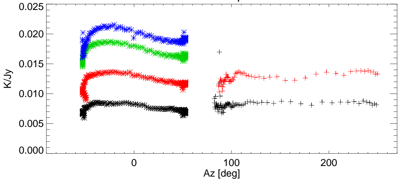
Gain vs Az for various shims. freq=8789 Pol:B RemoveBase.
