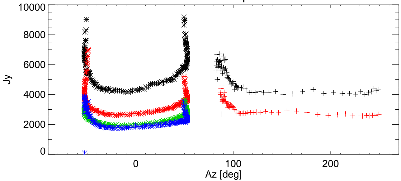
SEFD vs Az for various shims. freq=8789 Pol:B RemoveBase.
