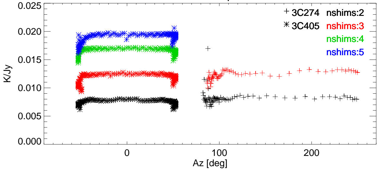
Gain vs Az for various shims. freq=8789 Pol:A RemoveBase.
