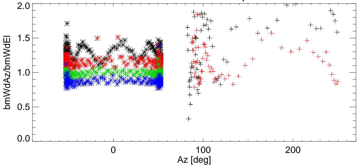
Az/EI BmWdRatio vs Az for various shims. freq=8789 Pol:B RemoveBase.
