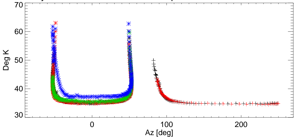
Tsys vs Az for various shims. freq=8789 Pol:B RemoveBase.
