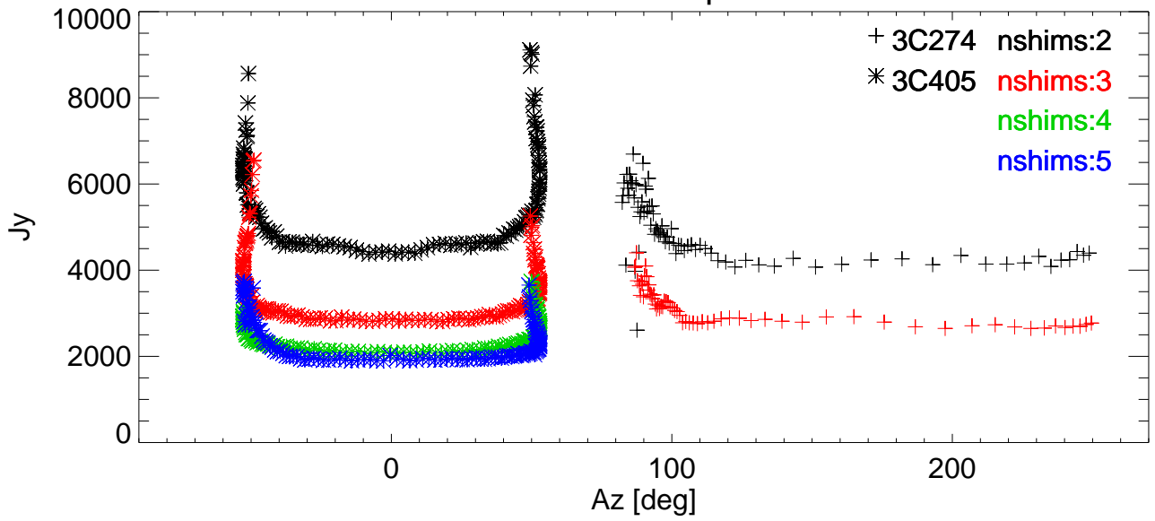
SEFD vs Az for various shims. freq=8789 Pol:A RemoveBase.
