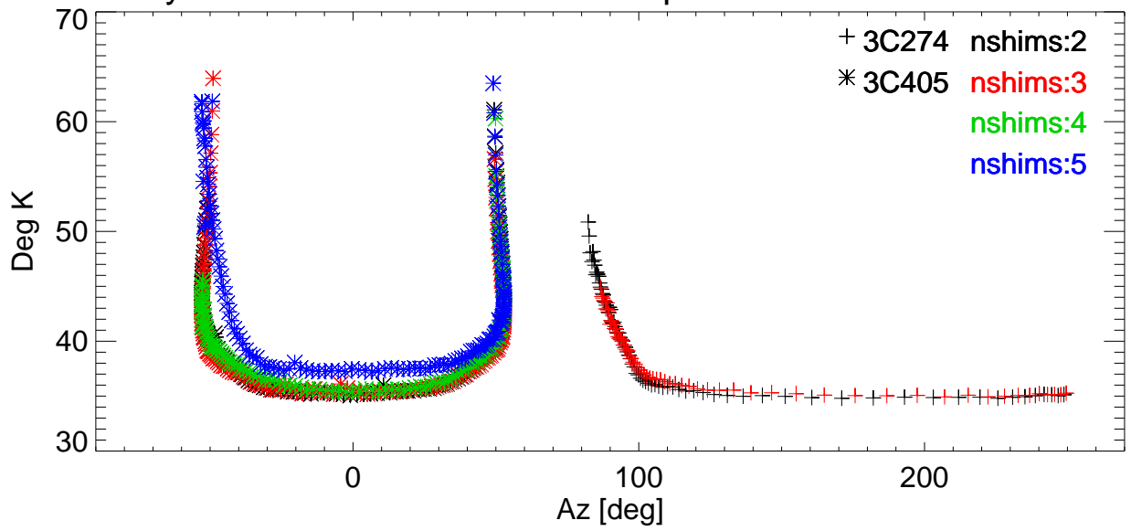
Tsys vs Az for various shims. freq=8789 Pol:A RemoveBase.
