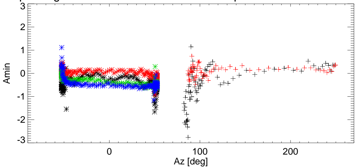
El pointing error vs Az for various shims. freq=8789 Pol:B RemoveBase.
