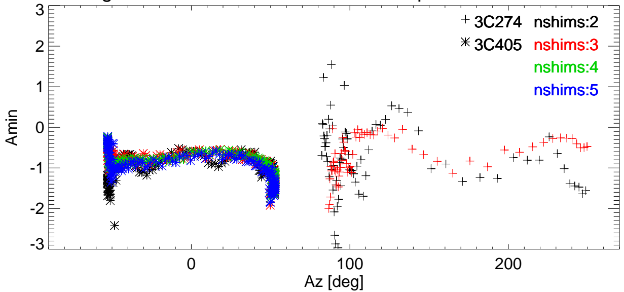
Az Pointing error vs Az for various shims. freq=8505 Pol:A RemoveBase.
