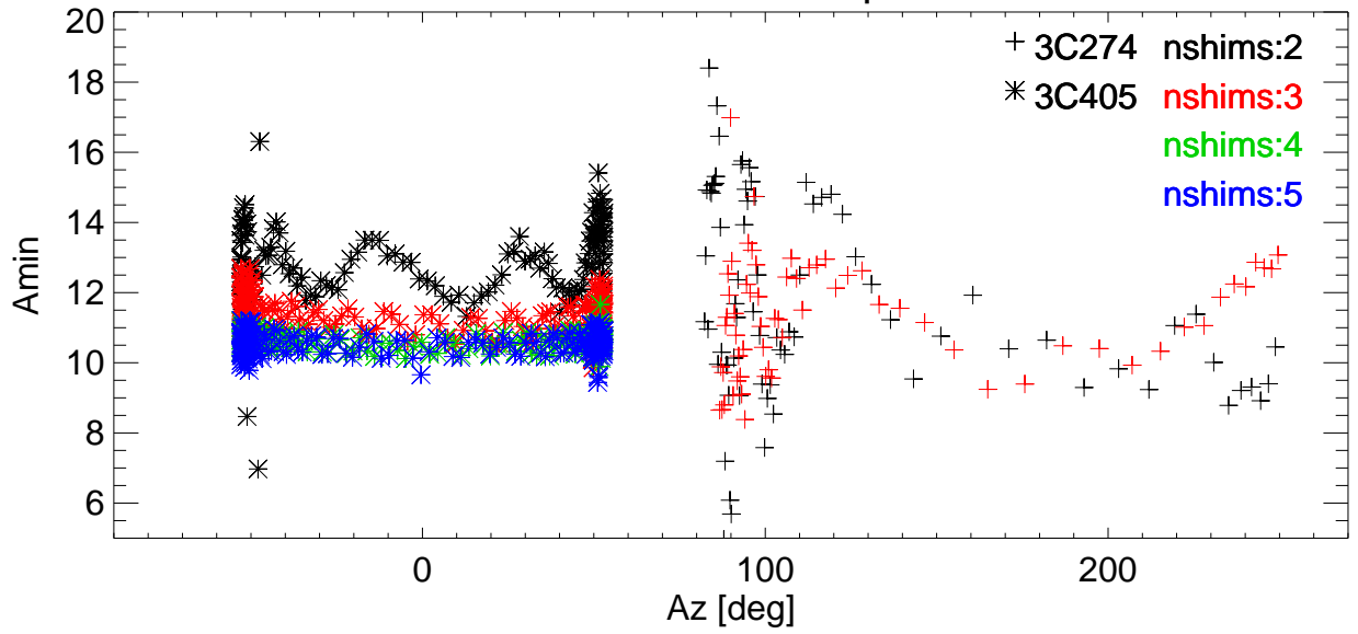
El BmWidth vs Az for various shims. freq=8505 Pol:A RemoveBase.
