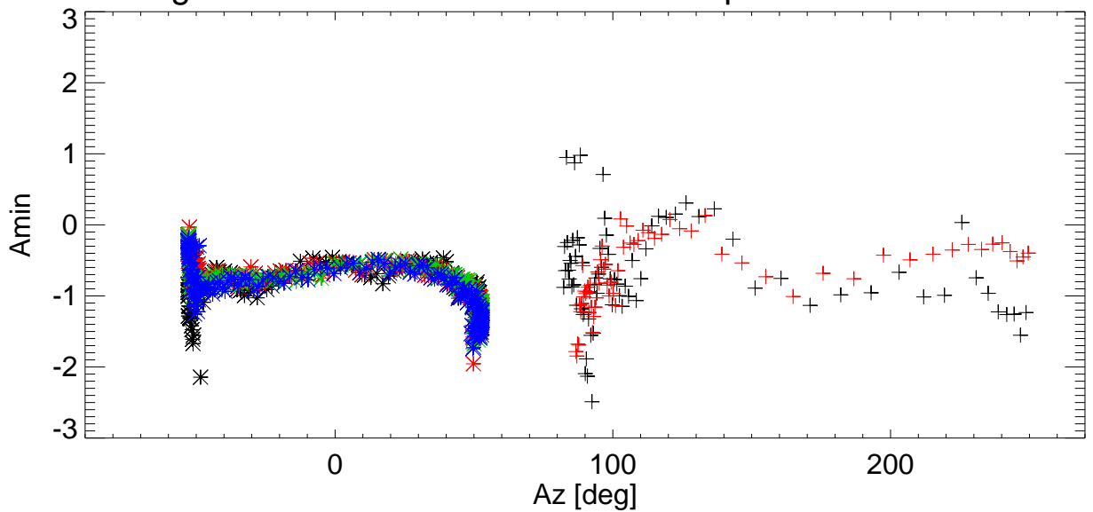
Az Pointing error vs Az for various shims. freq=8505 Pol:B RemoveBase.
