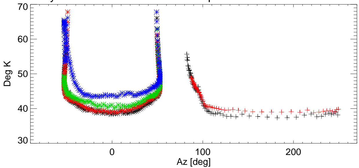
Tsys vs Az for various shims. freq=8505 Pol:B RemoveBase.
