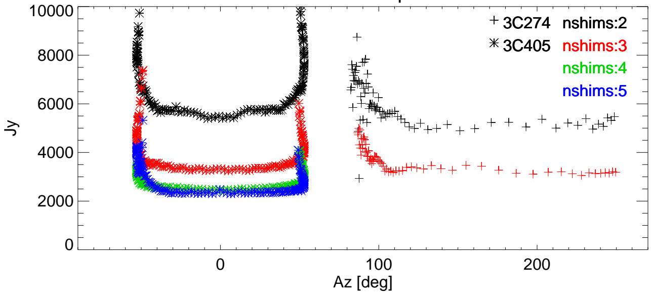
SEFD vs Az for various shims. freq=8505 Pol:A RemoveBase.
