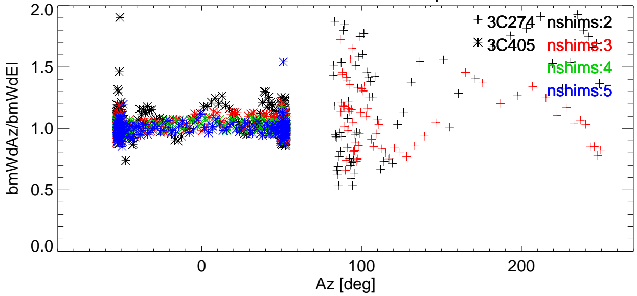
Az/EI BmWdRatio vs Az for various shims. freq=8505 Pol:A RemoveBase.
