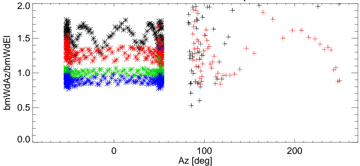
Az/EI BmWdRatio vs Az for various shims. freq=8505 Pol:B RemoveBase.
