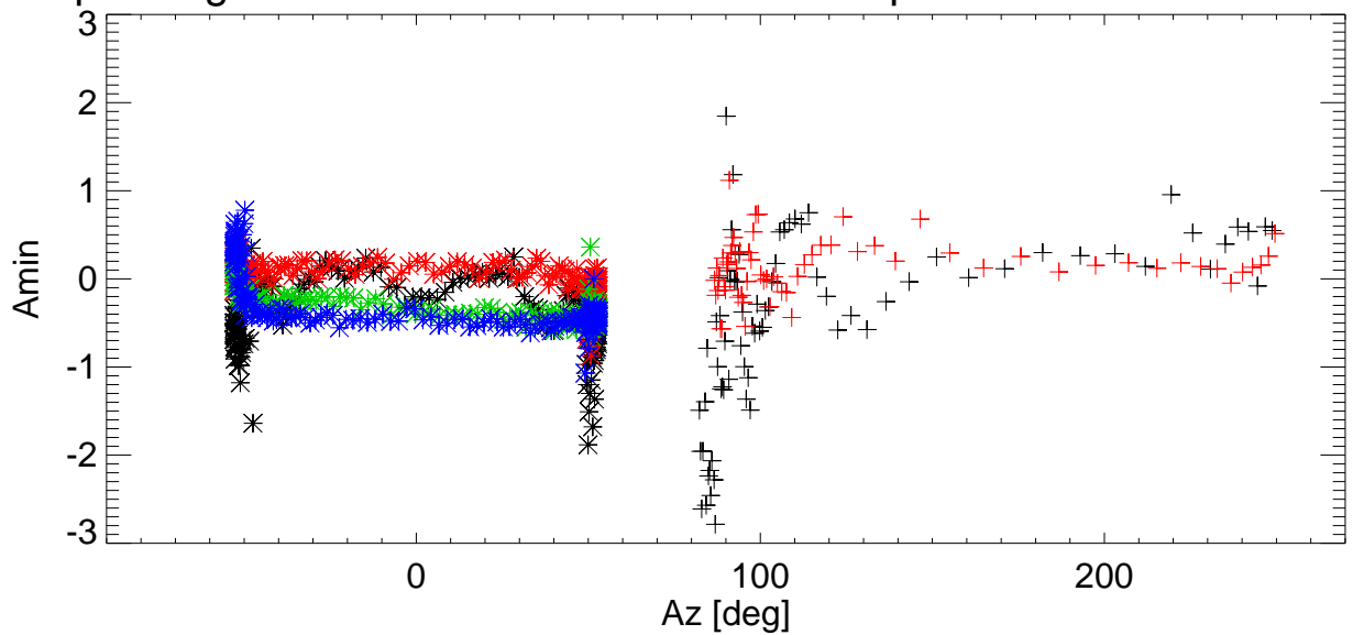
El pointing error vs Az for various shims. freq=8505 Pol:B RemoveBase.
