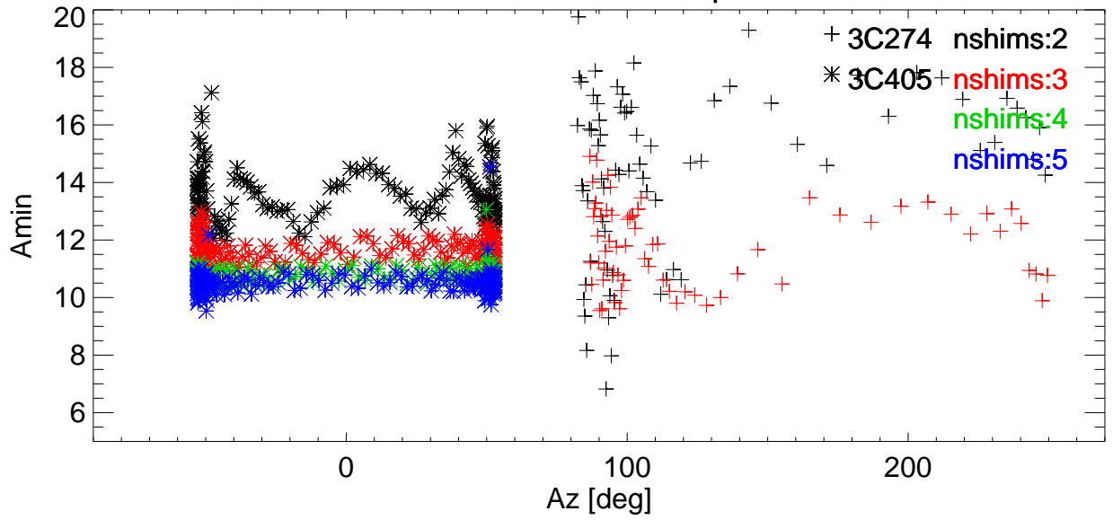
Az BmWidth vs Az for various shims. freq=8505 Pol:A RemoveBase.
