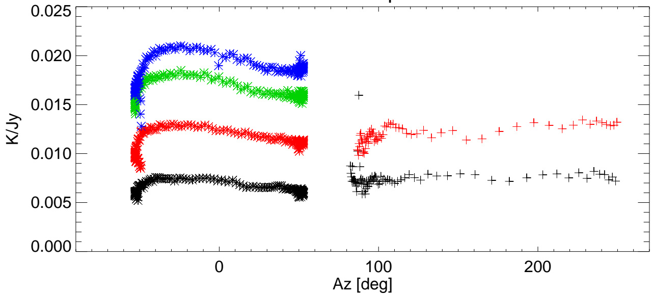
Gain vs Az for various shims. freq=8505 Pol:B RemoveBase.
