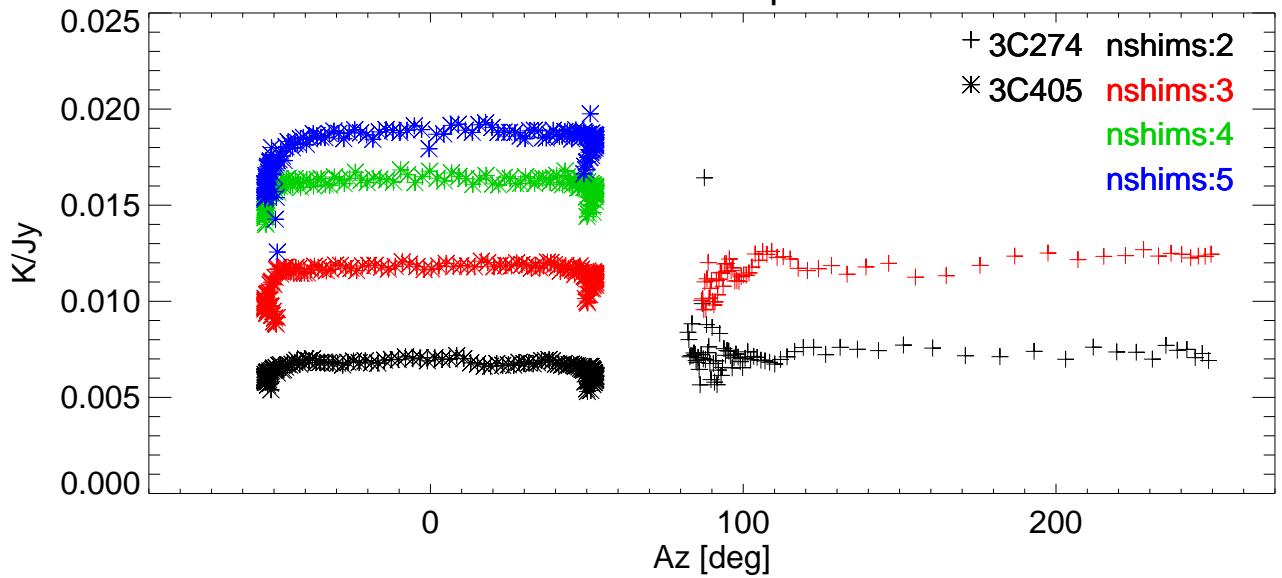
Gain vs Az for various shims. freq=8505 Pol:A RemoveBase.
