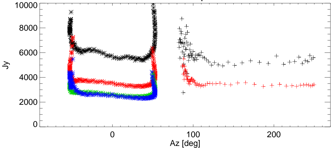
SEFD vs Az for various shims. freq=8505 Pol:B RemoveBase.
