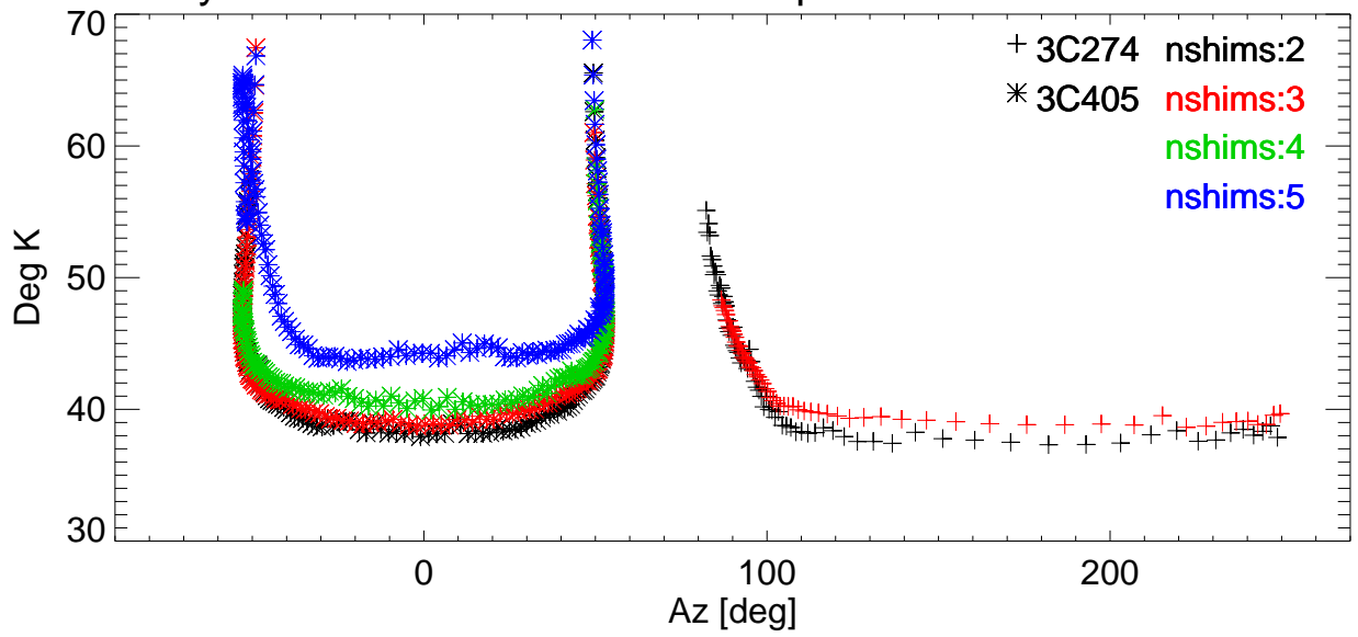
Tsys vs Az for various shims. freq=8505 Pol:A RemoveBase.
