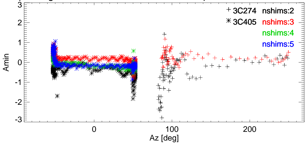
El pointing error vs Az for various shims. freq=8505 Pol:A RemoveBase.
