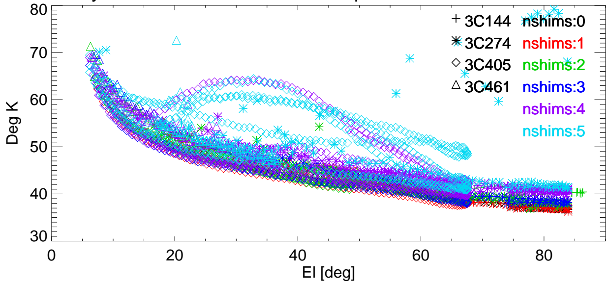
Tsys vs El for various shims. freq=8647 Pol:A RemoveBase.
