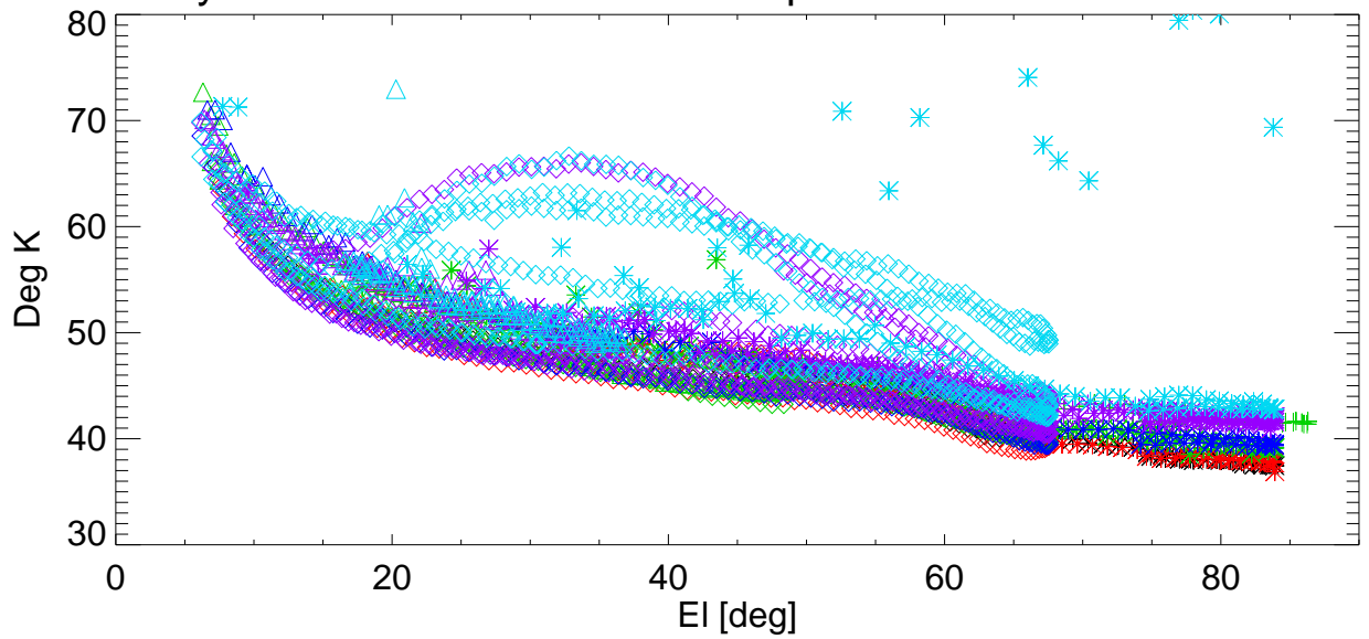
Tsys vs El for various shims. freq=8647 Pol:B RemoveBase.
