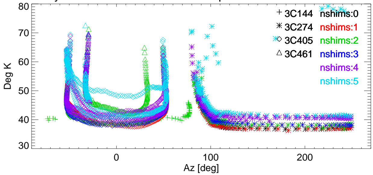
Tsys vs Az for various shims. freq=8647 Pol:A RemoveBase.
