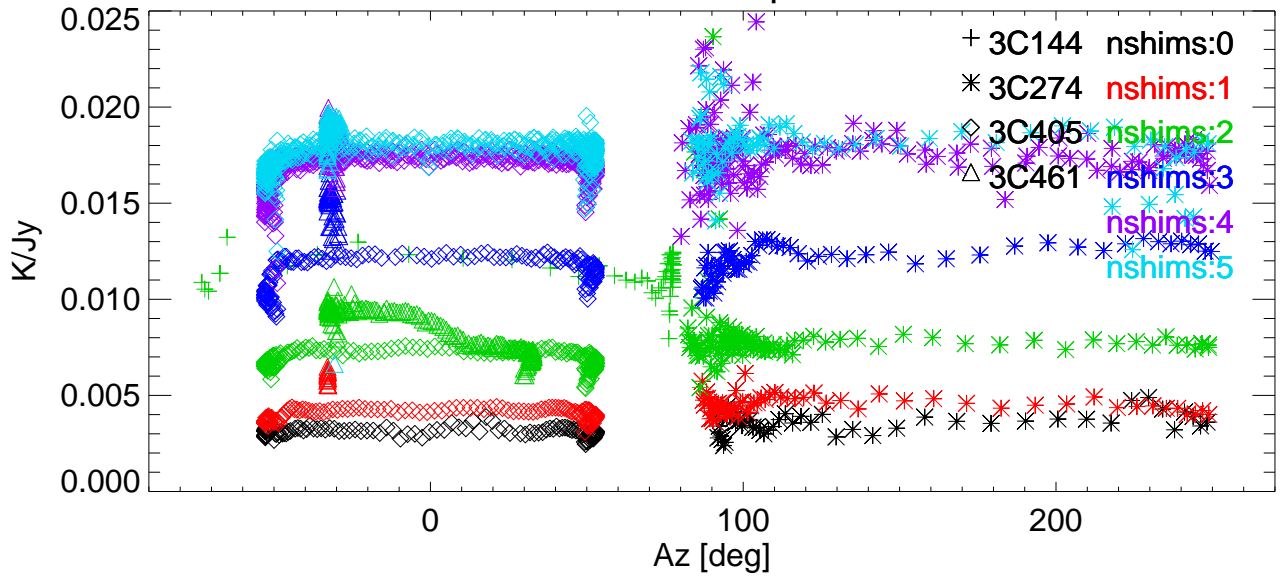
Gain vs Az for various shims. freq=8647 Pol:A RemoveBase.
