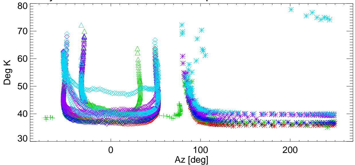
Tsys vs Az for various shims. freq=8647 Pol:B RemoveBase.
