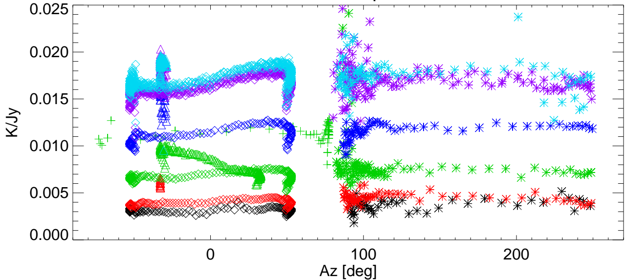
Gain vs Az for various shims. freq=8647 Pol:B RemoveBase.
