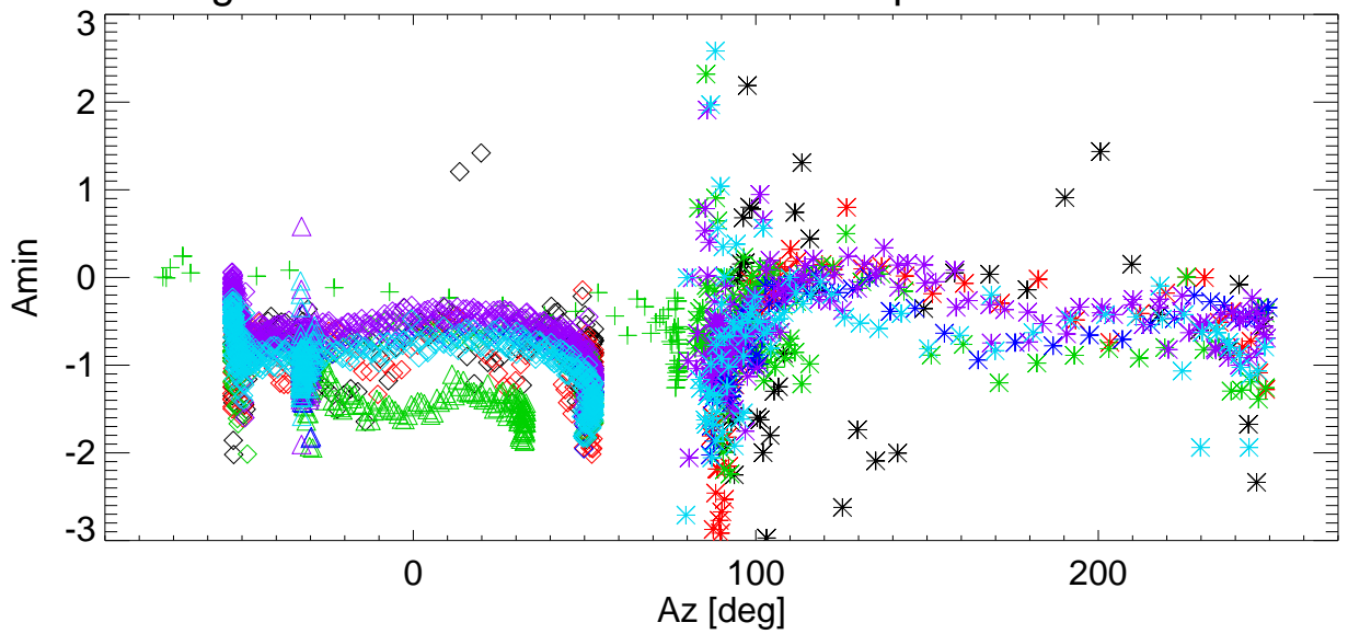
Az Pointing error vs Az for various shims. freq=8647 Pol:B RemoveBase.
