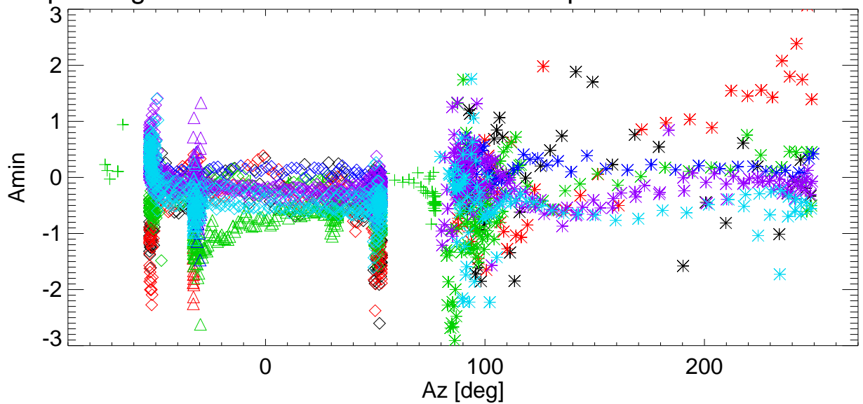
El pointing error vs Az for various shims. freq=8647 Pol:B RemoveBase.
