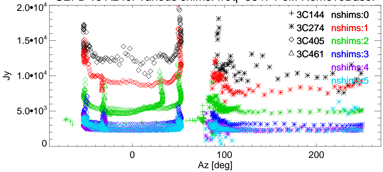
SEFD vs Az for various shims. freq=8647 Pol:A RemoveBase.
