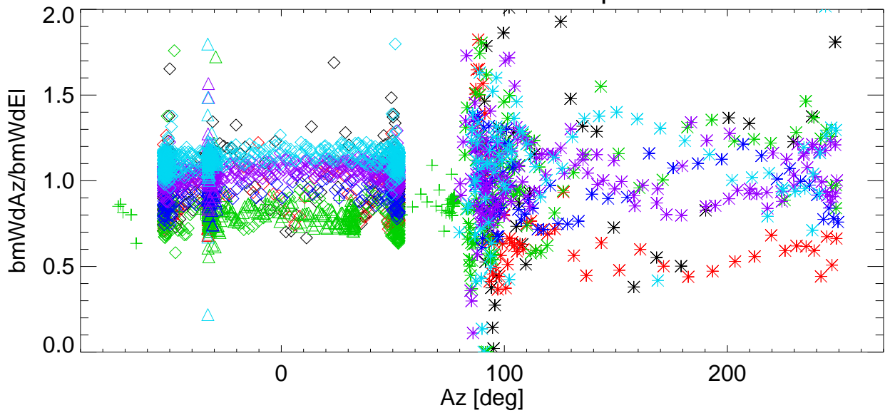
Az/EI BmWdRatio vs Az for various shims. freq=8647 Pol:B RemoveBase.
