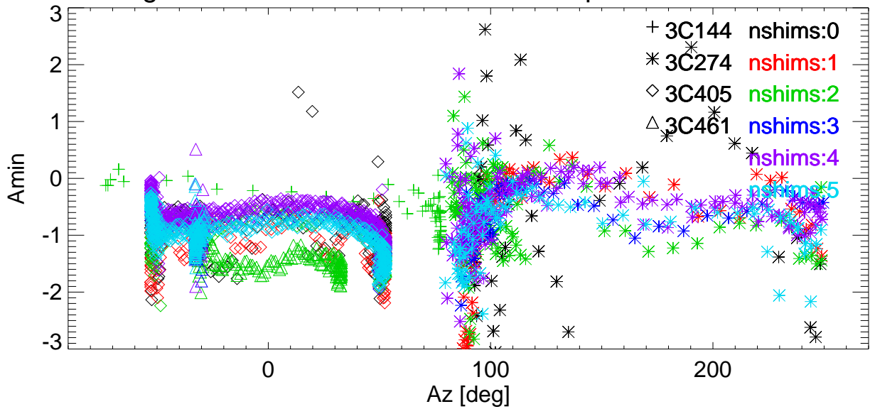
Az Pointing error vs Az for various shims. freq=8647 Pol:A RemoveBase.
