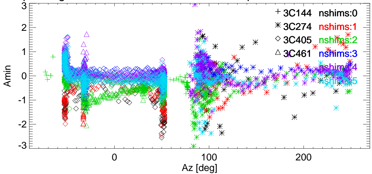
El pointing error vs Az for various shims. freq=8647 Pol:A RemoveBase.
