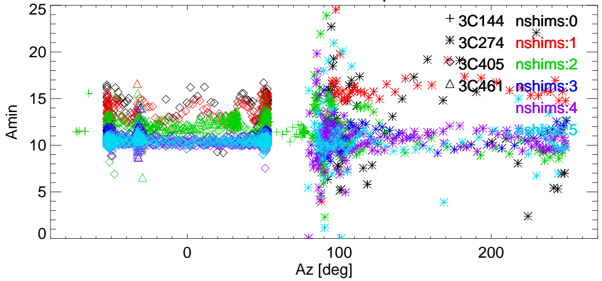
El BmWidth vs Az for various shims. freq=8647 Pol:A RemoveBase.
