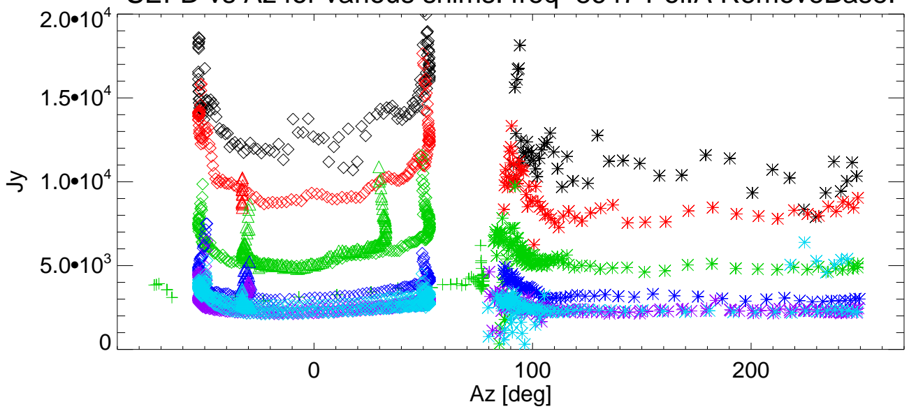
SEFD vs Az for various shims. freq=8647 Pol:B RemoveBase.
