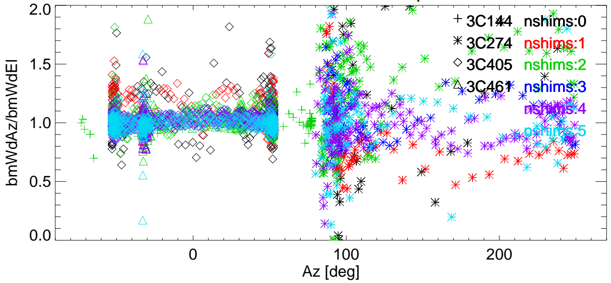
Az/EI BmWdRatio vs Az for various shims. freq=8647 Pol:A RemoveBase.
