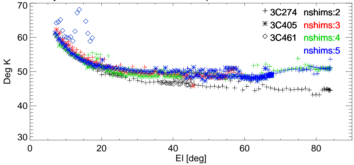
Tsys vs EI for various shims. freq=3414 Pol:A RemoveBase.
