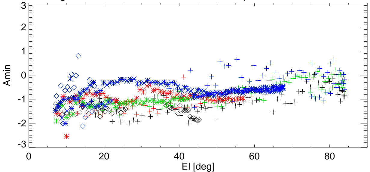
Az Pointing error vs EI for various shims. freq=3414 Pol:B RemoveBase.
