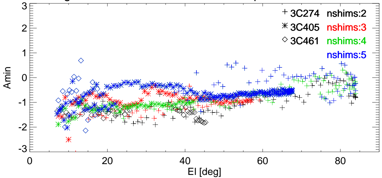
Az Pointing error vs EI for various shims. freq=3414 Pol:A RemoveBase.
