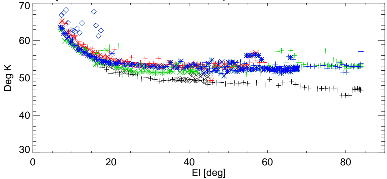
Tsys vs EI for various shims. freq=3414 Pol:B RemoveBase.
