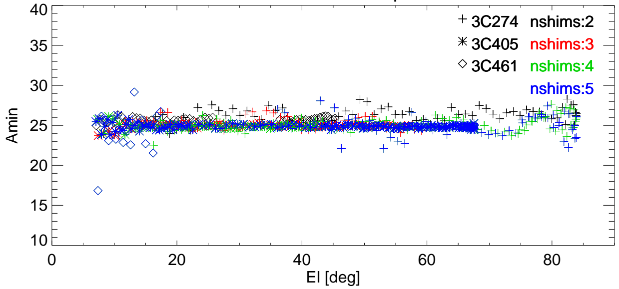
Az BmWidth vs EI for various shims. freq=3414 Pol:A RemoveBase.
