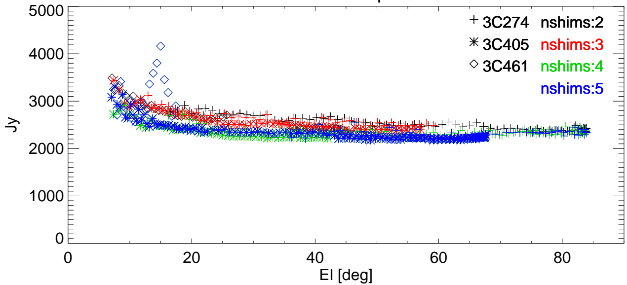
SEFD vs EI for various shims. freq=3414 Pol:A RemoveBase.
