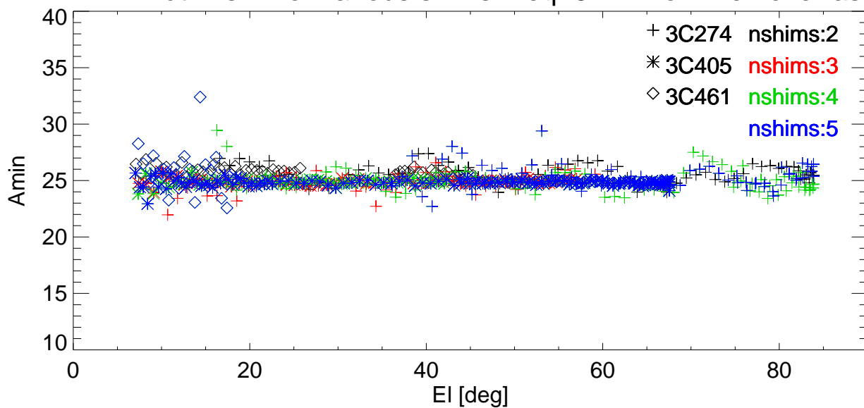
El BmWidth vs El for various shims. freq=3414 Pol:A RemoveBase.
