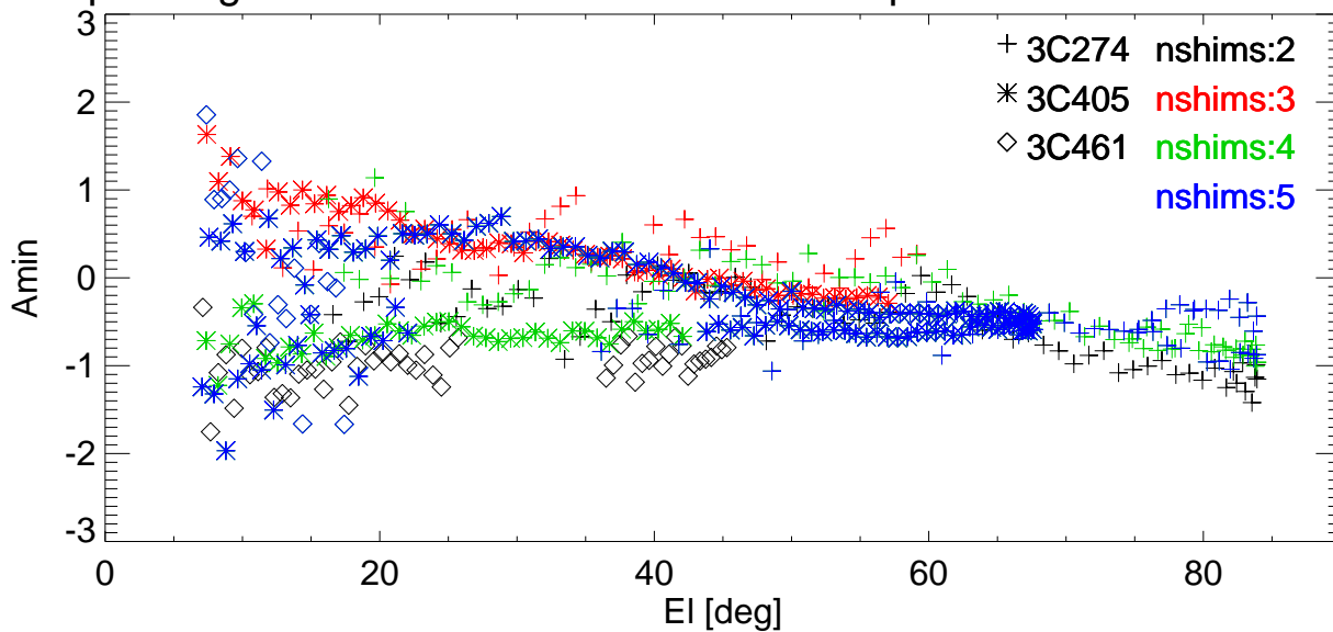
El pointing error vs El for various shims. freq=3414 Pol:A RemoveBase.
