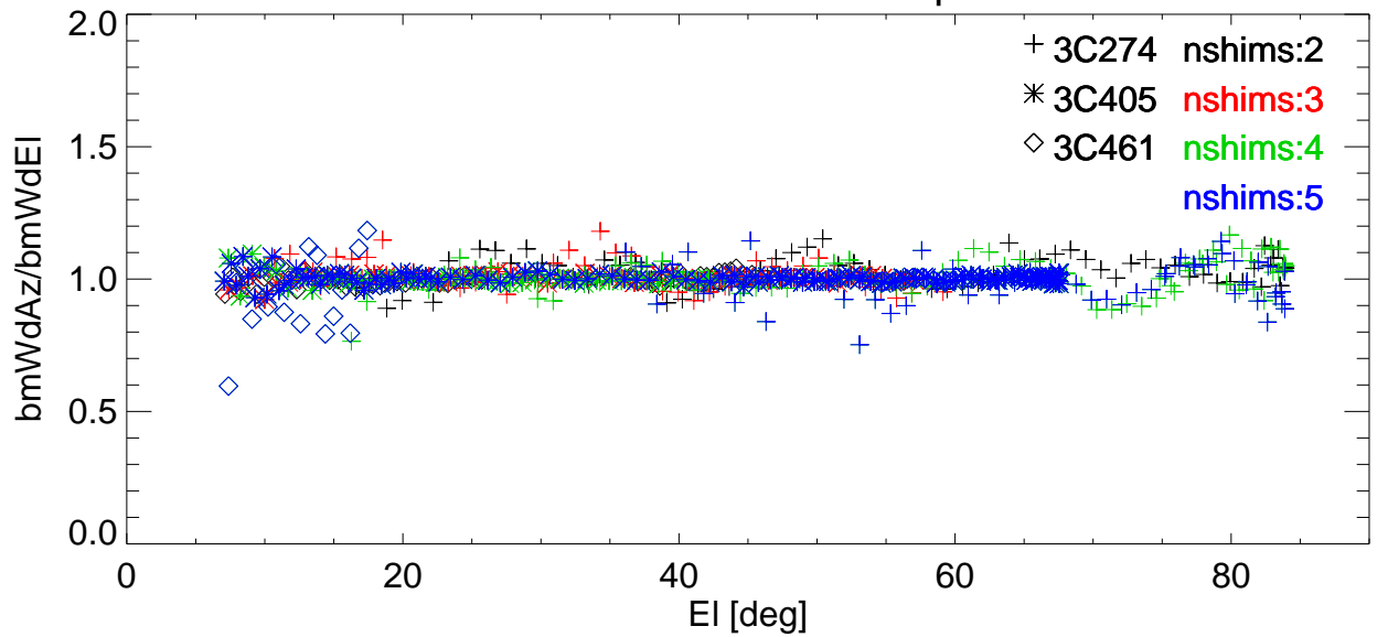
Az/EI BmWdRatio vs EI for various shims. freq=3414 Pol:A RemoveBase.
