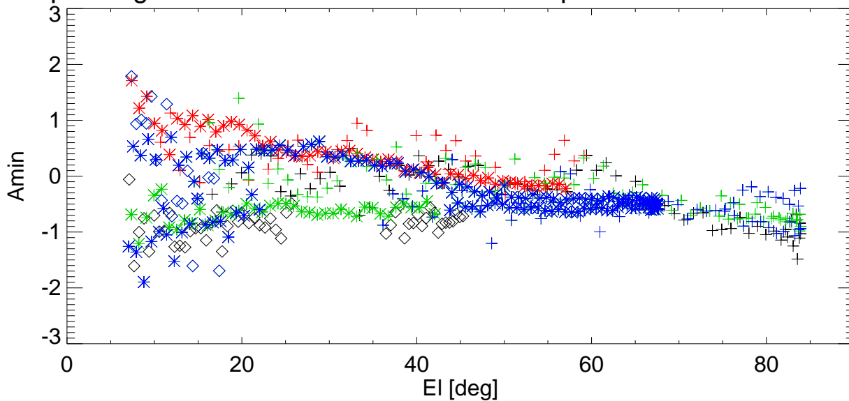
El pointing error vs El for various shims. freq=3414 Pol:B RemoveBase.
