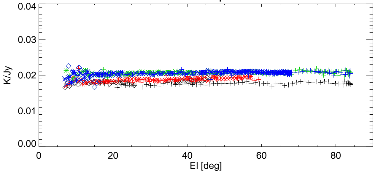
Gain vs EI for various shims. freq=3414 Pol:B RemoveBase.
