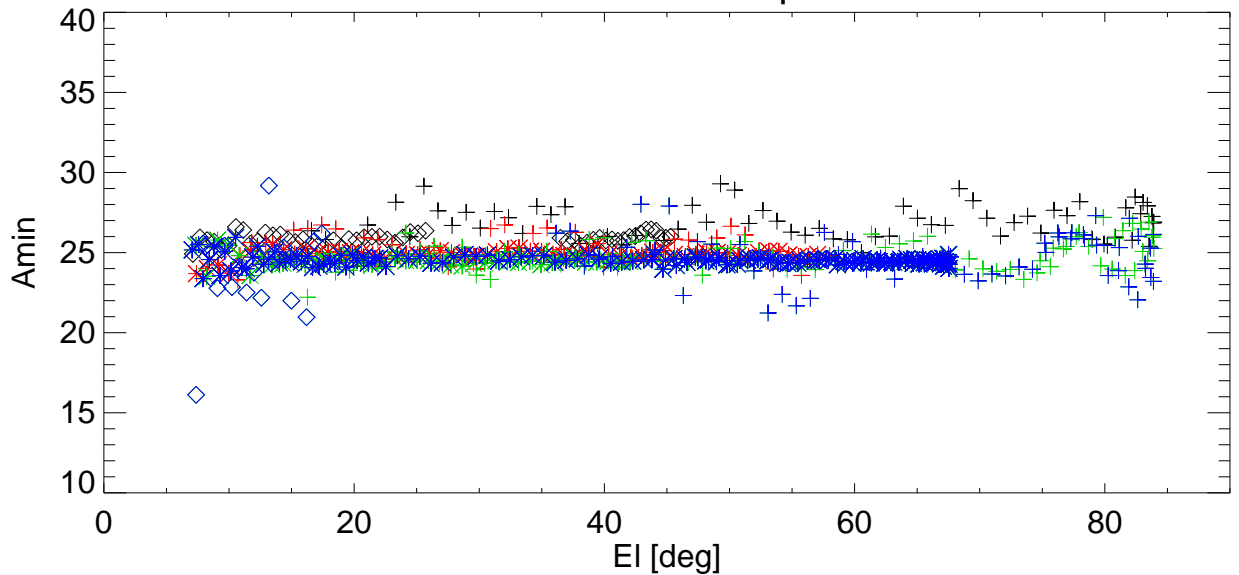
Az BmWidth vs EI for various shims. freq=3414 Pol:B RemoveBase.
