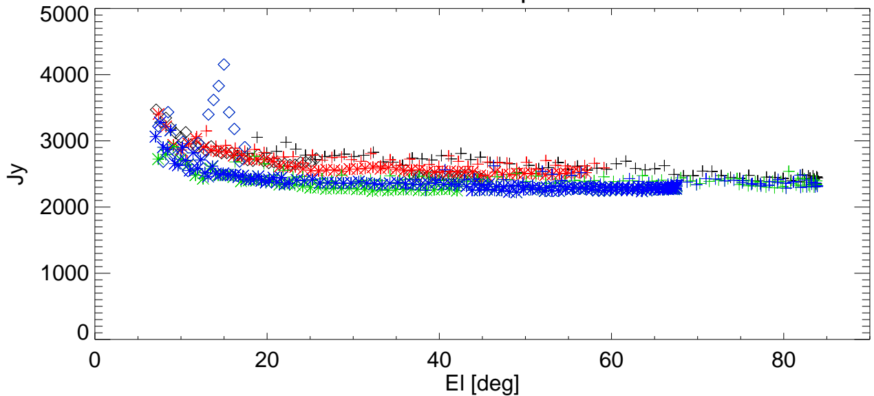
SEFD vs EI for various shims. freq=3414 Pol:B RemoveBase.
