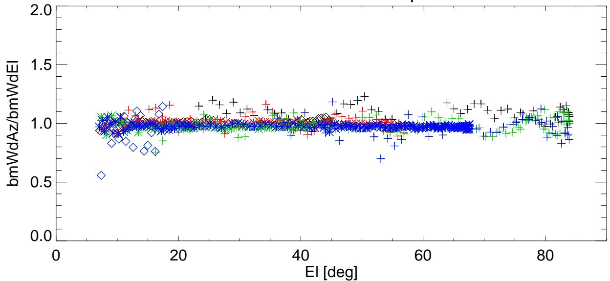
Az/EI BmWdRatio vs EI for various shims. freq=3414 Pol:B RemoveBase.
