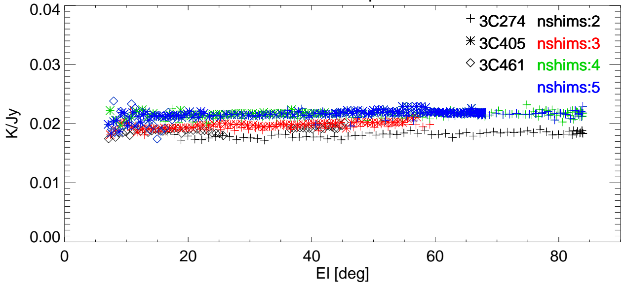
Gain vs EI for various shims. freq=3414 Pol:A RemoveBase.
