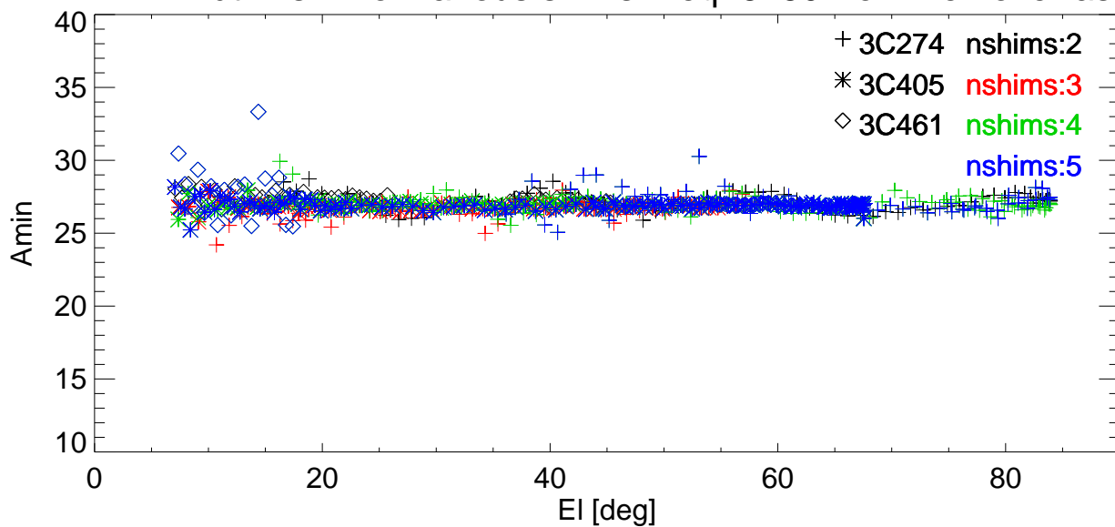
El BmWidth vs El for various shims. freq=3130 Pol:A RemoveBase.
