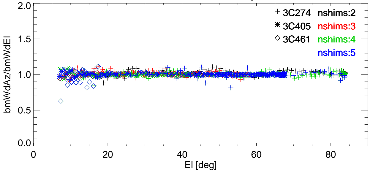
Az/EI BmWdRatio vs EI for various shims. freq=3130 Pol:A RemoveBase.
