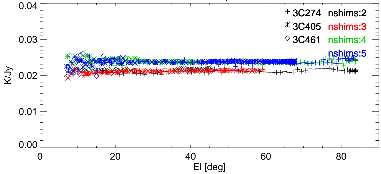
Gain vs EI for various shims. freq=3130 Pol:A RemoveBase.
