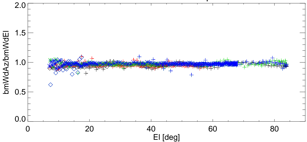
Az/EI BmWdRatio vs EI for various shims. freq=3130 Pol:B RemoveBase.
