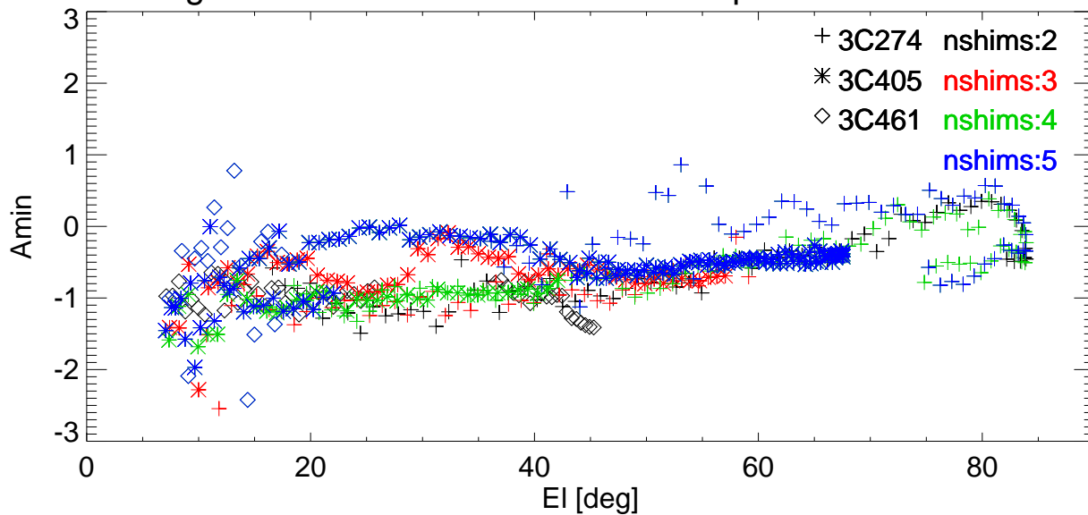
Az Pointing error vs EI for various shims. freq=3130 Pol:A RemoveBase.
