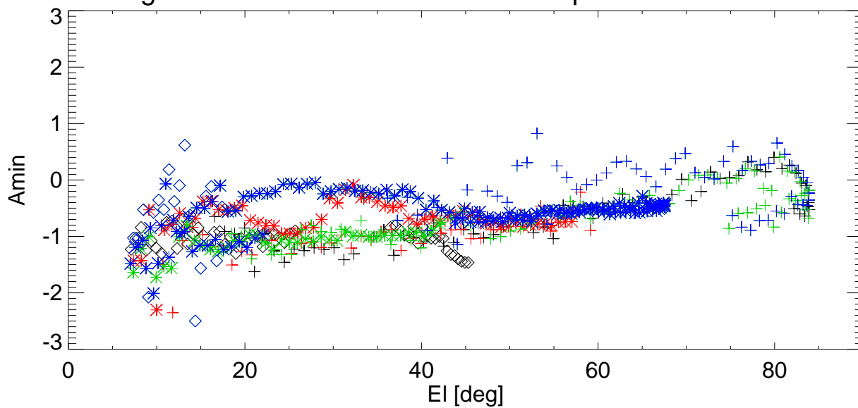
Az Pointing error vs EI for various shims. freq=3130 Pol:B RemoveBase.
