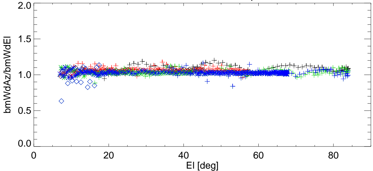
Az/EI BmWdRatio vs EI for various shims. freq=3130 Pol:B RemoveBase.
