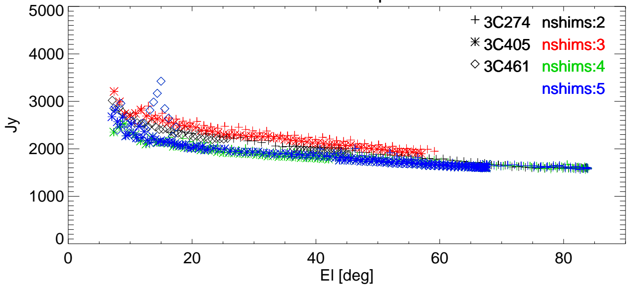
SEFD vs EI for various shims. freq=3130 Pol:A RemoveBase.
