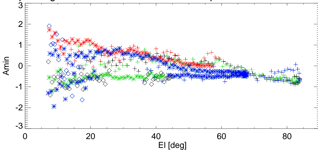
El pointing error vs El for various shims. freq=3130 Pol:B RemoveBase.
