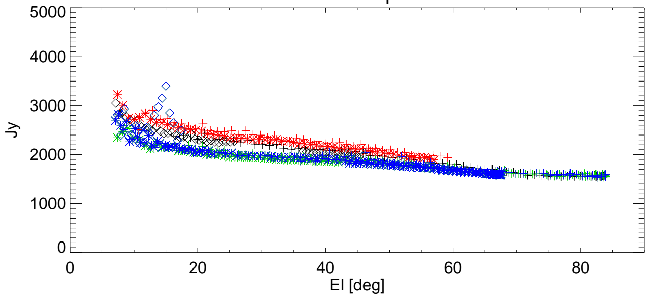
SEFD vs EI for various shims. freq=3130 Pol:B RemoveBase.
