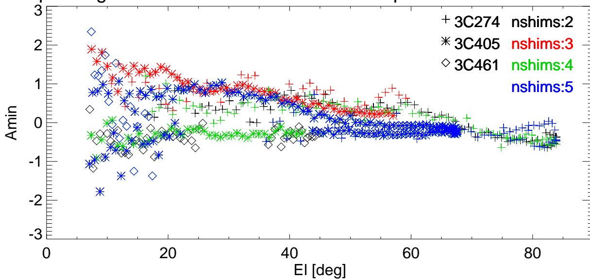
El pointing error vs El for various shims. freq=3130 Pol:A RemoveBase.
