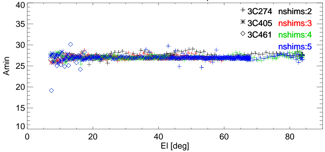
Az BmWidth vs EI for various shims. freq=3130 Pol:A RemoveBase.
