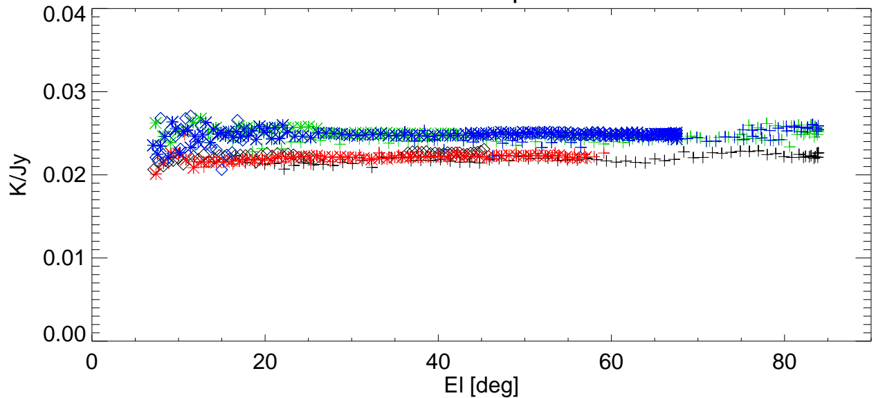
Gain vs EI for various shims. freq=3130 Pol:B RemoveBase.
