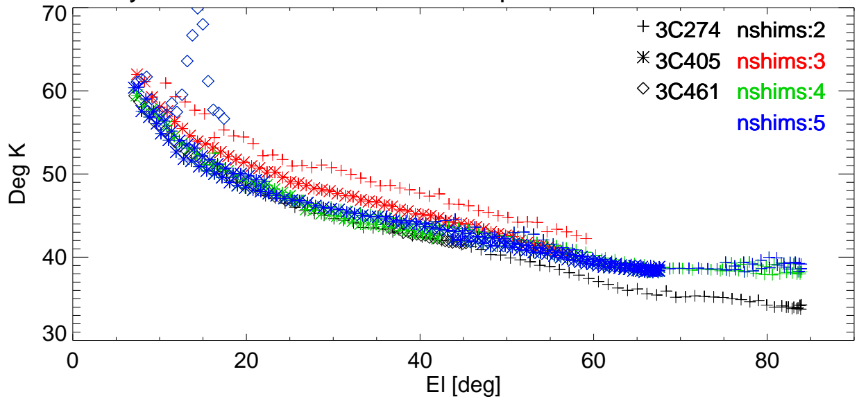
Tsys vs EI for various shims. freq=3130 Pol:A RemoveBase.
