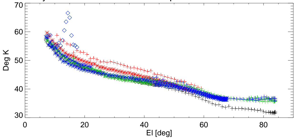
Tsys vs EI for various shims. freq=3130 Pol:B RemoveBase.
