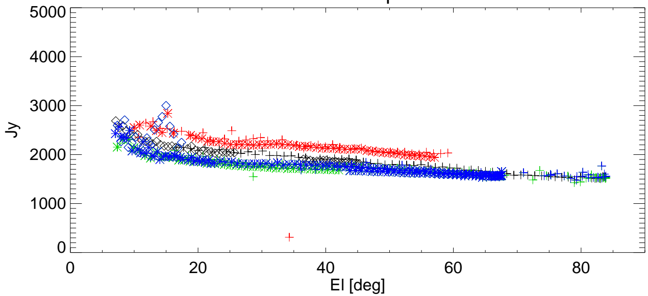
SEFD vs EI for various shims. freq=2846 Pol:B RemoveBase.
