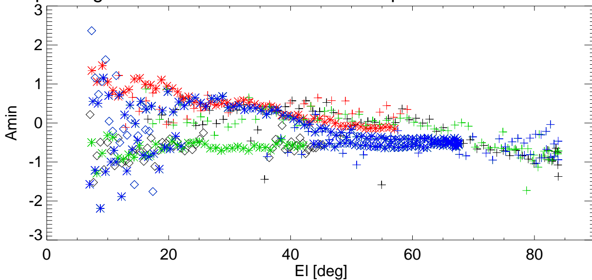
El pointing error vs El for various shims. freq=2846 Pol:B RemoveBase.
