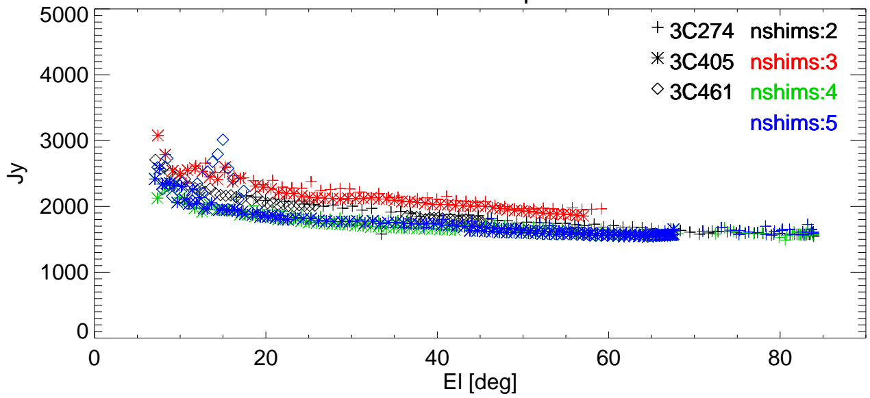
SEFD vs EI for various shims. freq=2846 Pol:A RemoveBase.
