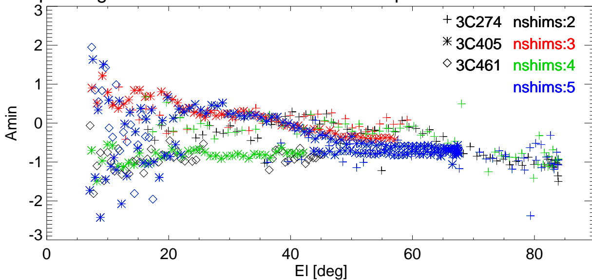
El pointing error vs El for various shims. freq=2846 Pol:A RemoveBase.
