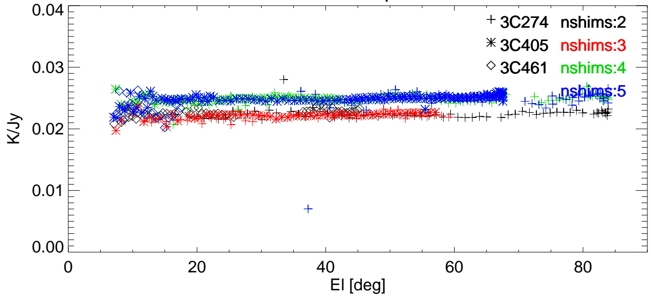
Gain vs EI for various shims. freq=2846 Pol:A RemoveBase.
