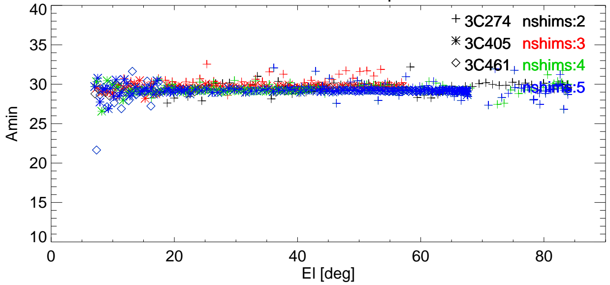
Az BmWidth vs EI for various shims. freq=2846 Pol:A RemoveBase.
