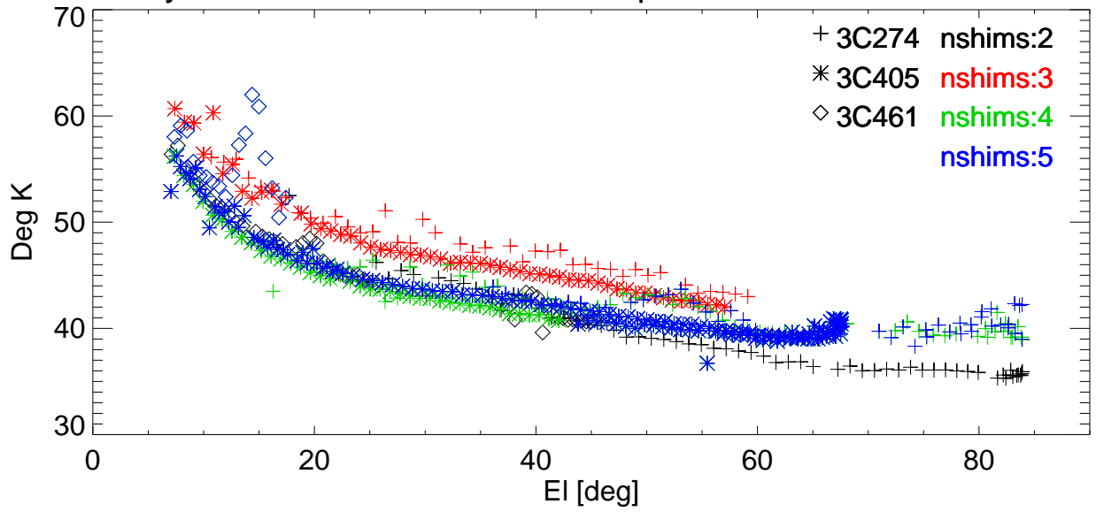
Tsys vs EI for various shims. freq=2846 Pol:A RemoveBase.
