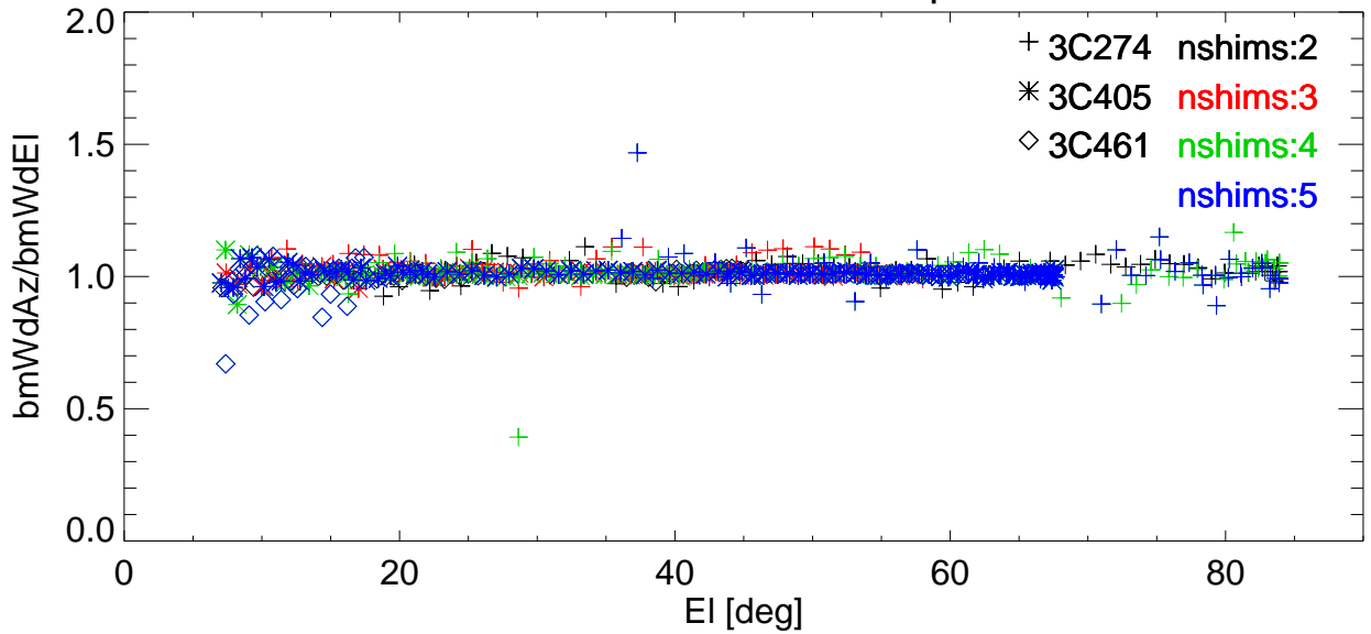
Az/EI BmWdRatio vs EI for various shims. freq=2846 Pol:A RemoveBase.
