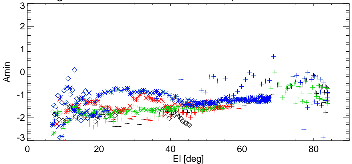
Az Pointing error vs EI for various shims. freq=2846 Pol:B RemoveBase.
