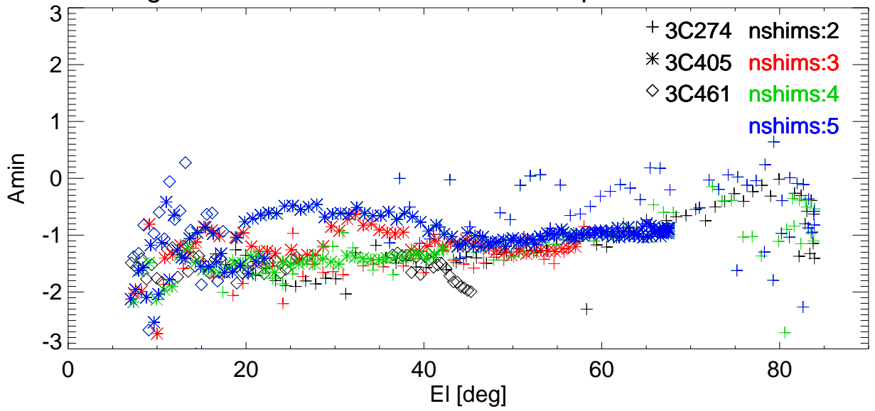
Az Pointing error vs EI for various shims. freq=2846 Pol:A RemoveBase.
