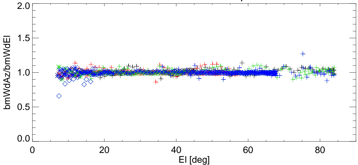
Az/EI BmWdRatio vs EI for various shims. freq=2846 Pol:B RemoveBase.
