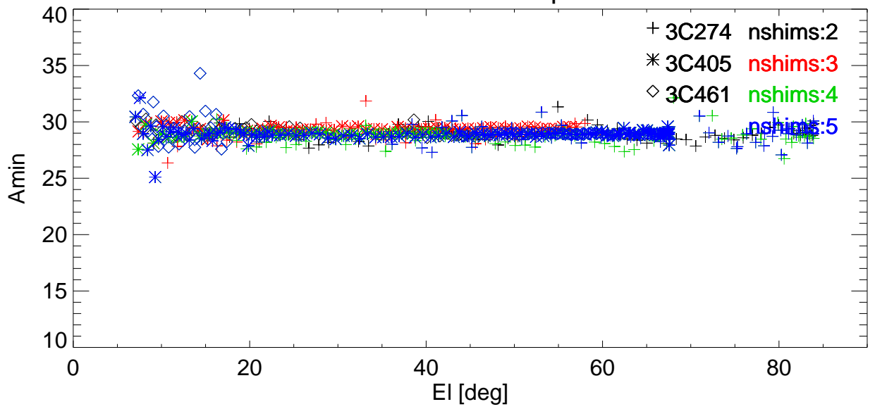
El BmWidth vs El for various shims. freq=2846 Pol:A RemoveBase.
