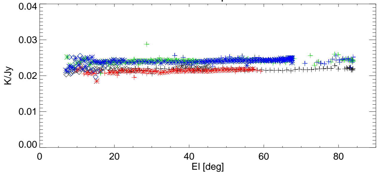
Gain vs EI for various shims. freq=2846 Pol:B RemoveBase.
