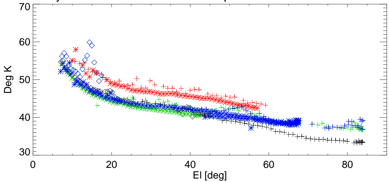
Tsys vs EI for various shims. freq=2846 Pol:B RemoveBase.
