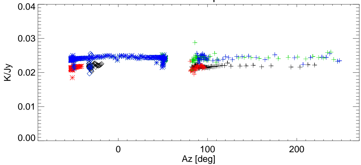
Gain vs Az for various shims. freq=2846 Pol:B RemoveBase.
