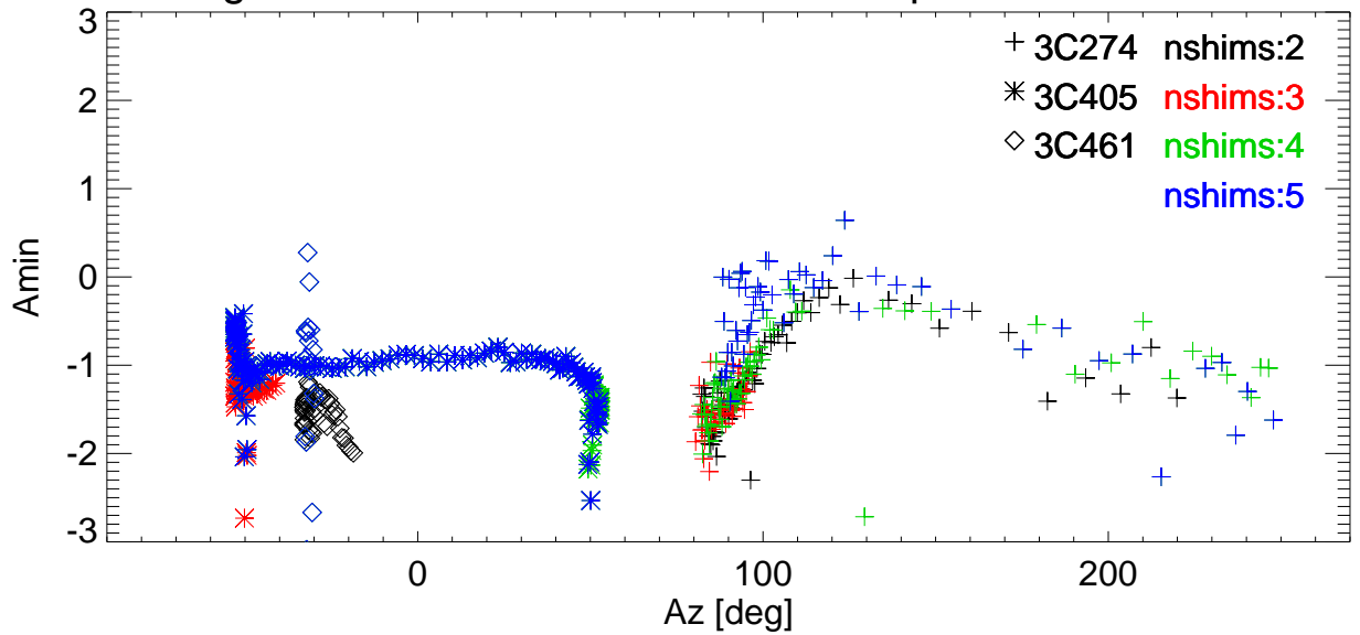
Az Pointing error vs Az for various shims. freq=2846 Pol:A RemoveBase.
