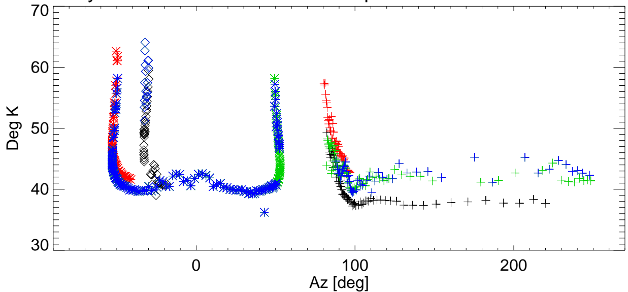
Tsys vs Az for various shims. freq=2846 Pol:B RemoveBase.
