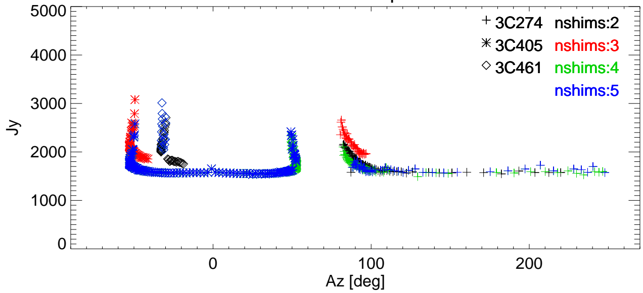
SEFD vs Az for various shims. freq=2846 Pol:A RemoveBase.
