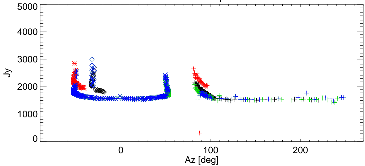
SEFD vs Az for various shims. freq=2846 Pol:B RemoveBase.
