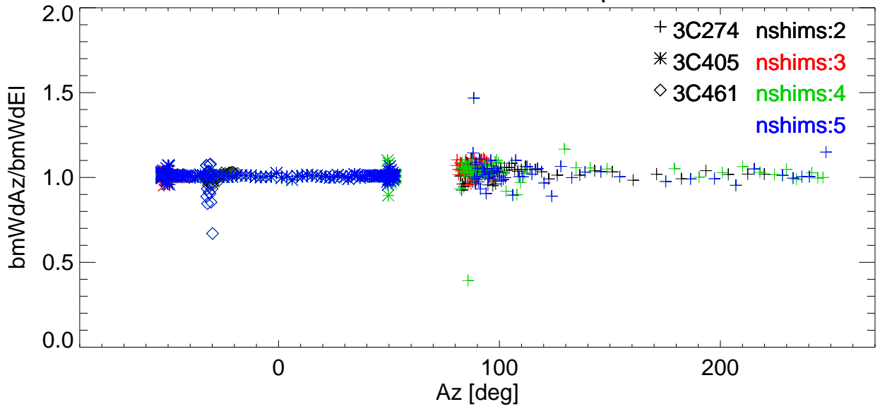
Az/EI BmWdRatio vs Az for various shims. freq=2846 Pol:A RemoveBase.
