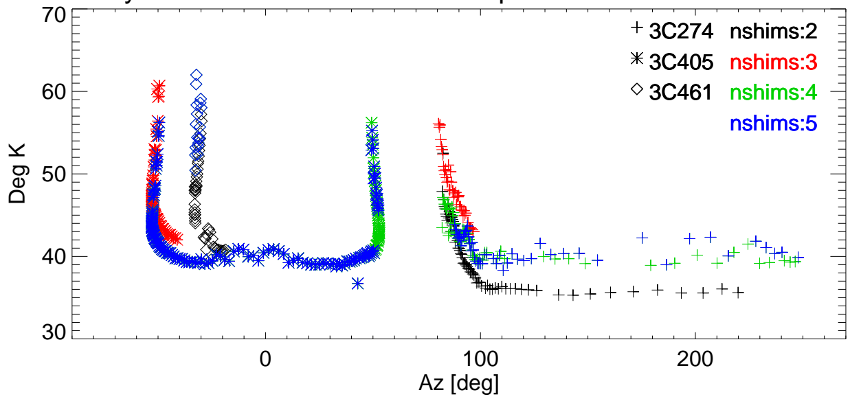
Tsys vs Az for various shims. freq=2846 Pol:A RemoveBase.
