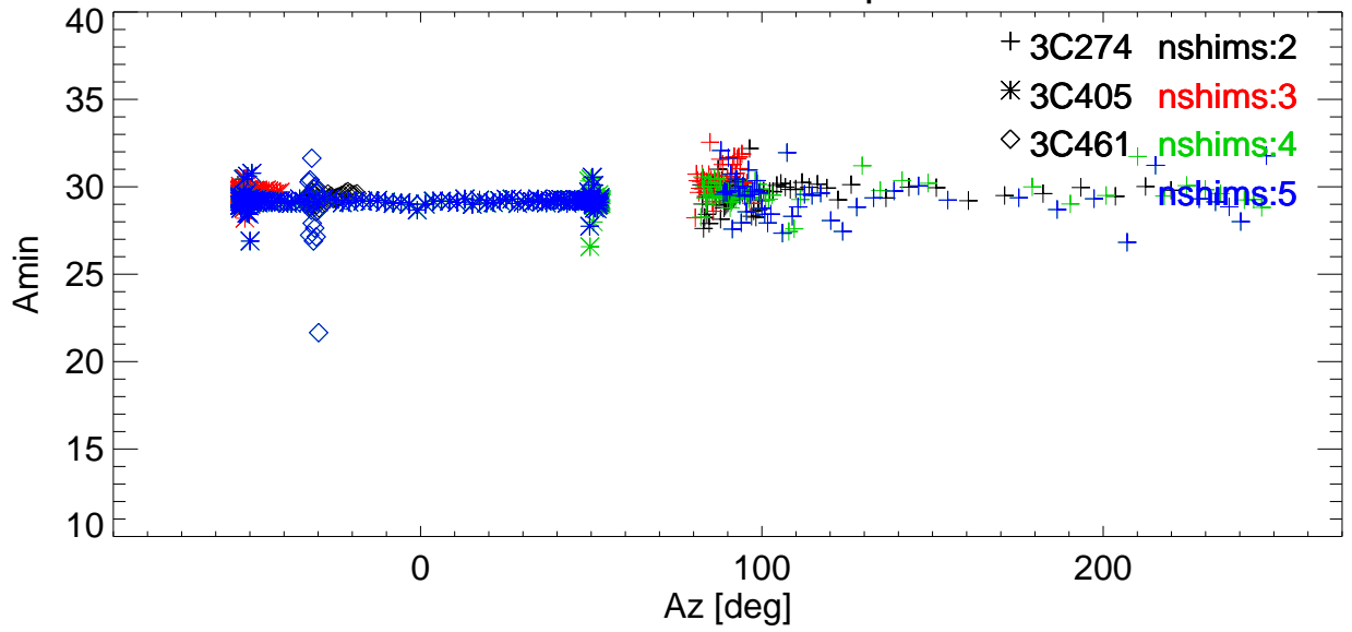
Az BmWidth vs Az for various shims. freq=2846 Pol:A RemoveBase.
