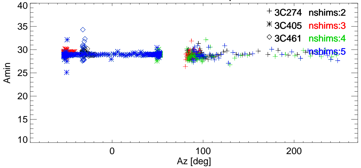
El BmWidth vs Az for various shims. freq=2846 Pol:A RemoveBase.
