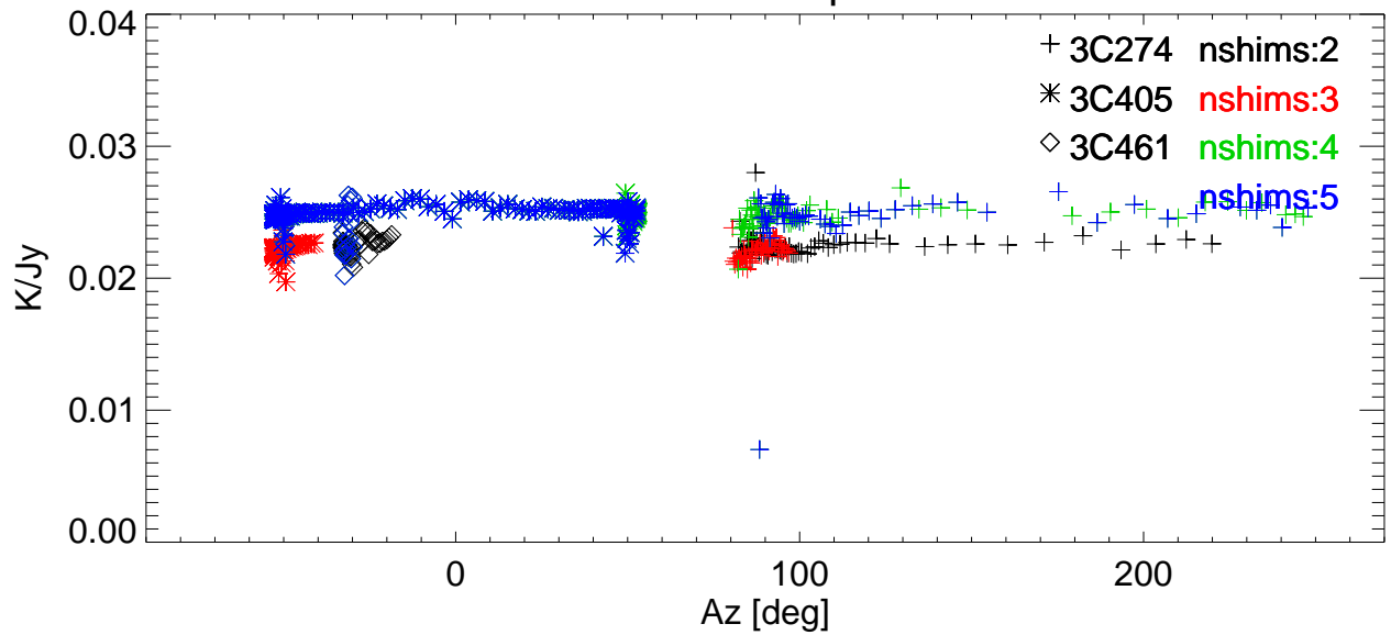
Gain vs Az for various shims. freq=2846 Pol:A RemoveBase.
