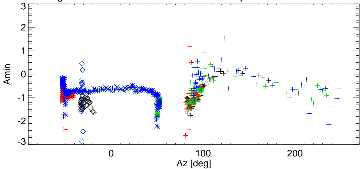
Az Pointing error vs Az for various shims. freq=2846 Pol:B RemoveBase.
