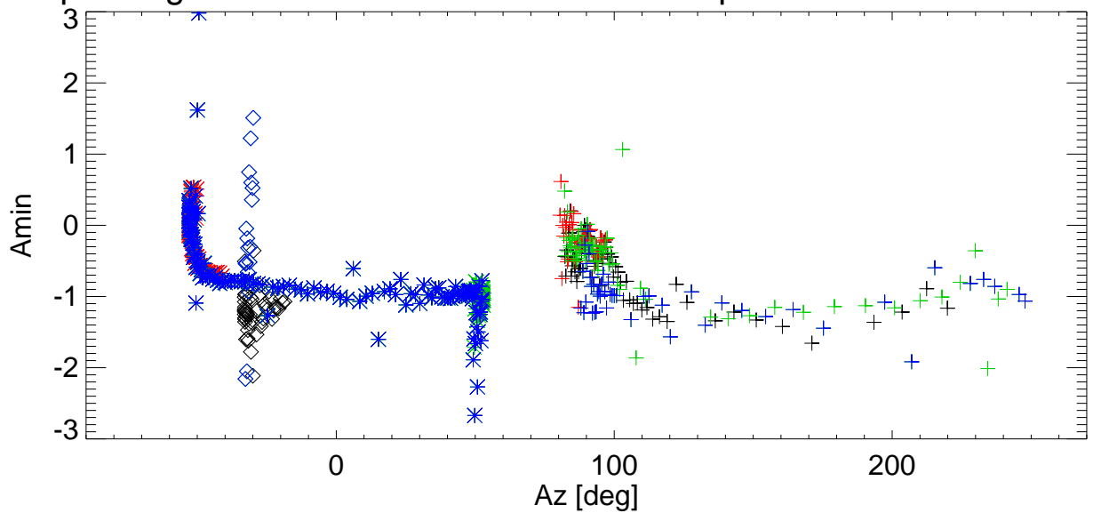
El pointing error vs Az for various shims. freq=2846 Pol:B RemoveBase.
