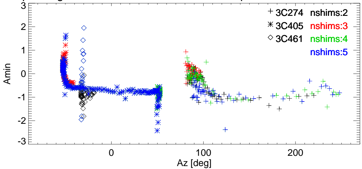
El pointing error vs Az for various shims. freq=2846 Pol:A RemoveBase.
