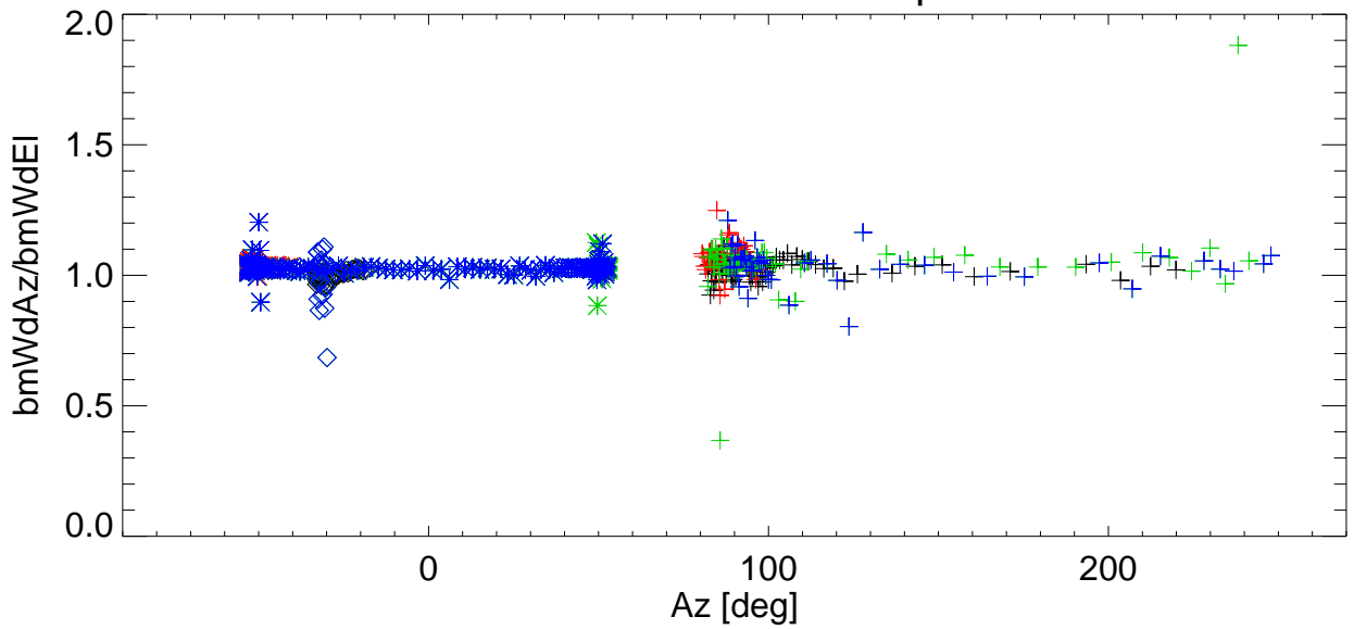
Az/EI BmWdRatio vs Az for various shims. freq=2846 Pol:B RemoveBase.
