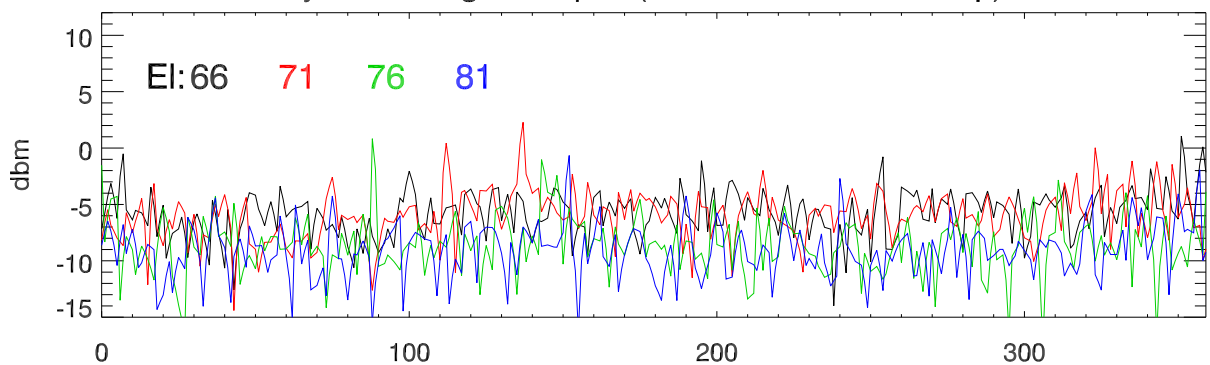
17may23 azswings total pwr (2-12GHz @ FilterBoxInp) vs az
