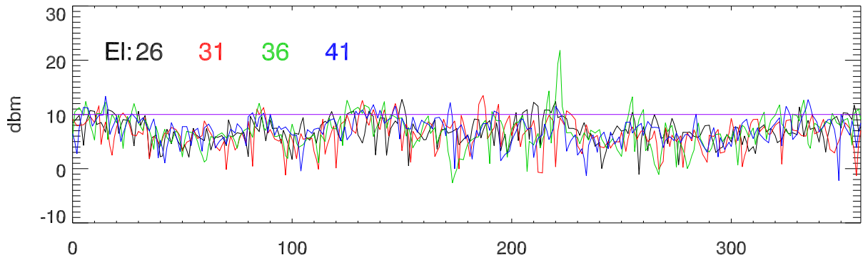
17may23 azswings total pwr (2-12GHz @ FoTxInp15db) vs az
