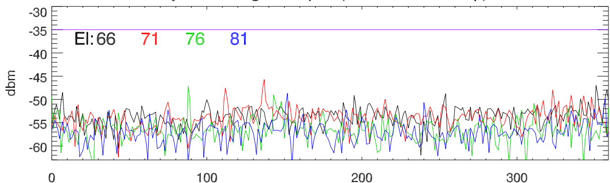
17may23 azswings total pwr (2-12GHz @ LnaInp) vs az
