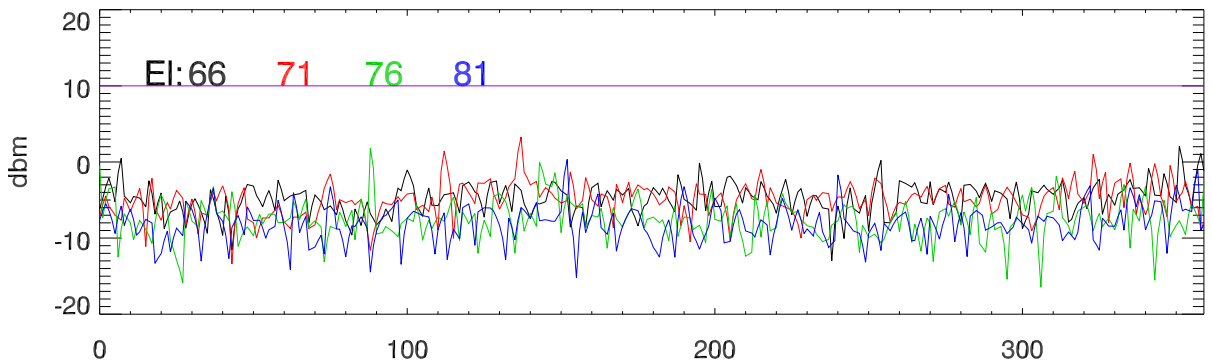
17may23 azswings total pwr (2-12GHz @ FOTxInp15+12db) vs az
