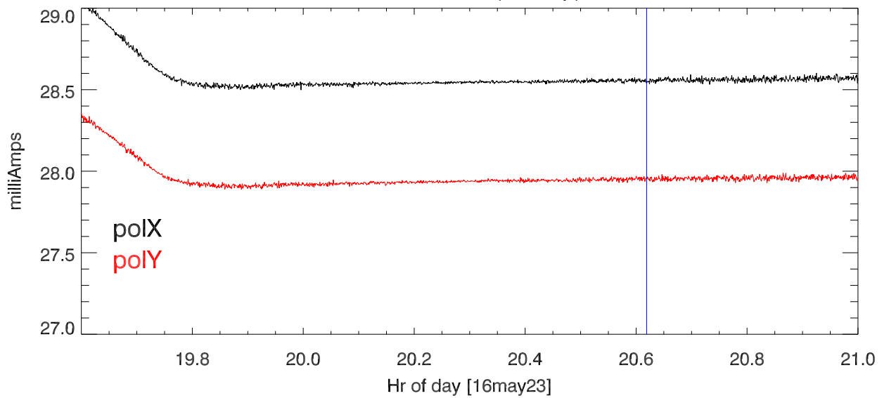
Drain current (blowup)
