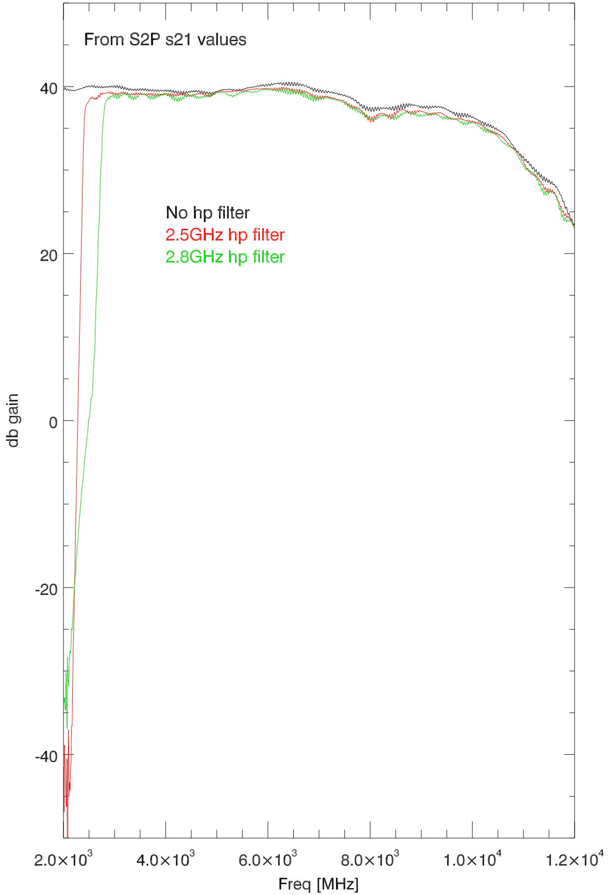
QRFH system gain (after horn) vs freq
