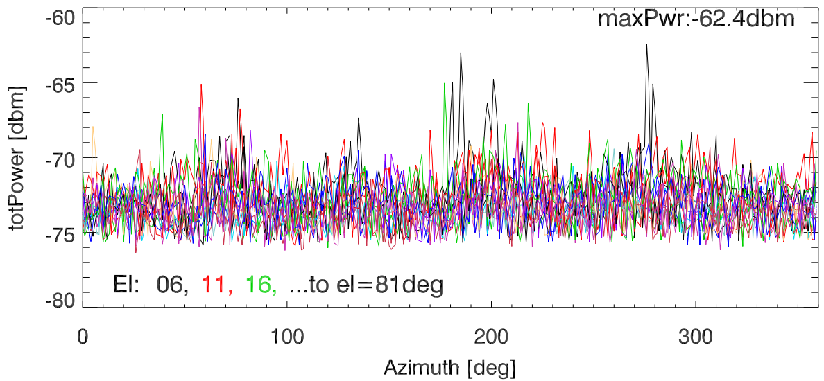
220620: 2.5 GHz HPFilter.( DriveAz @.2deg/sec, stepInEl)
