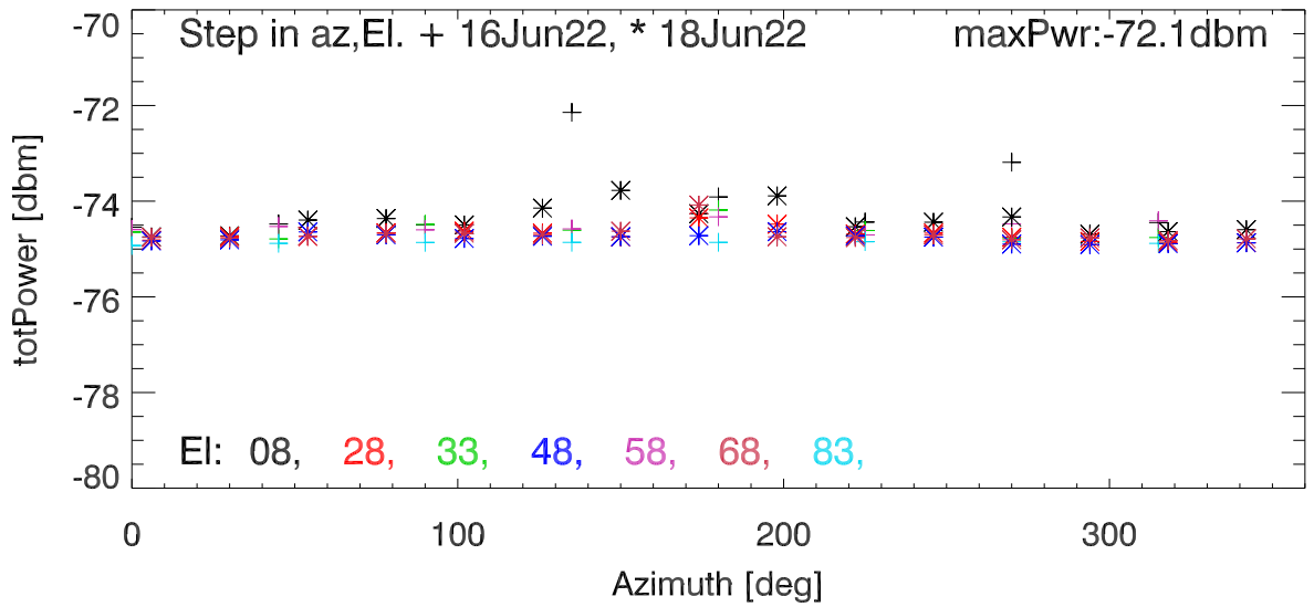
QRFH:TotPwr vs az,el. 2.8 GHz HPFilter. (Pwr at Output of Horn)
