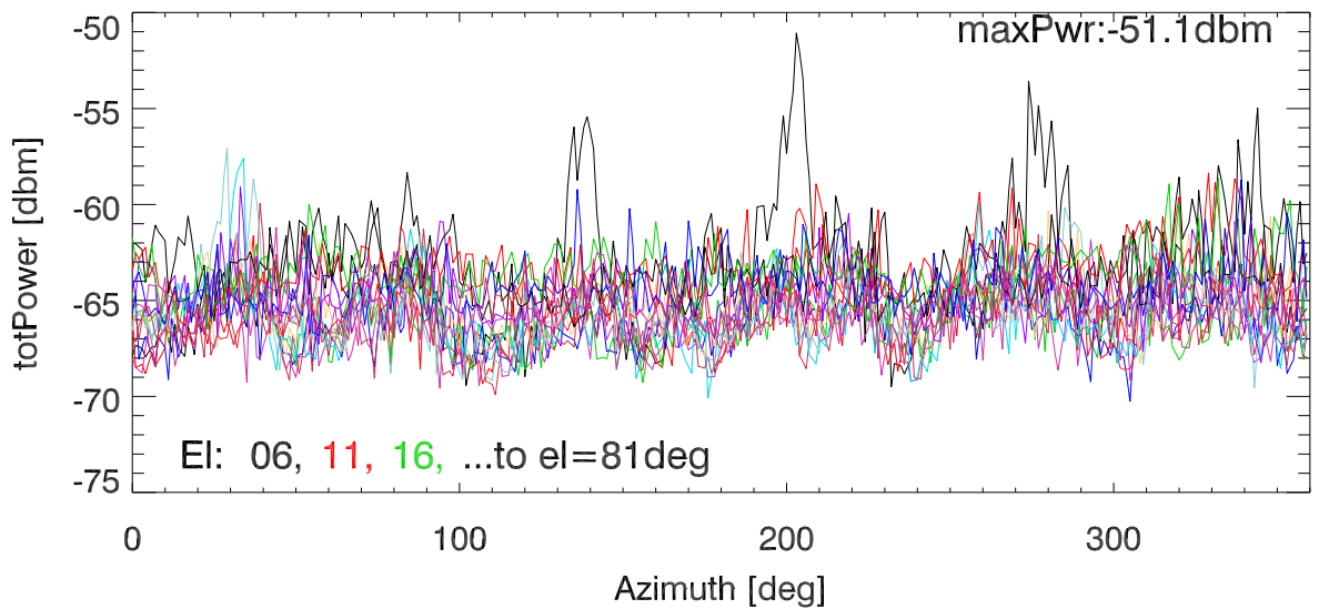
220621: No HPFilter. (DriveAz @.2deg/sec, stepInEl)
