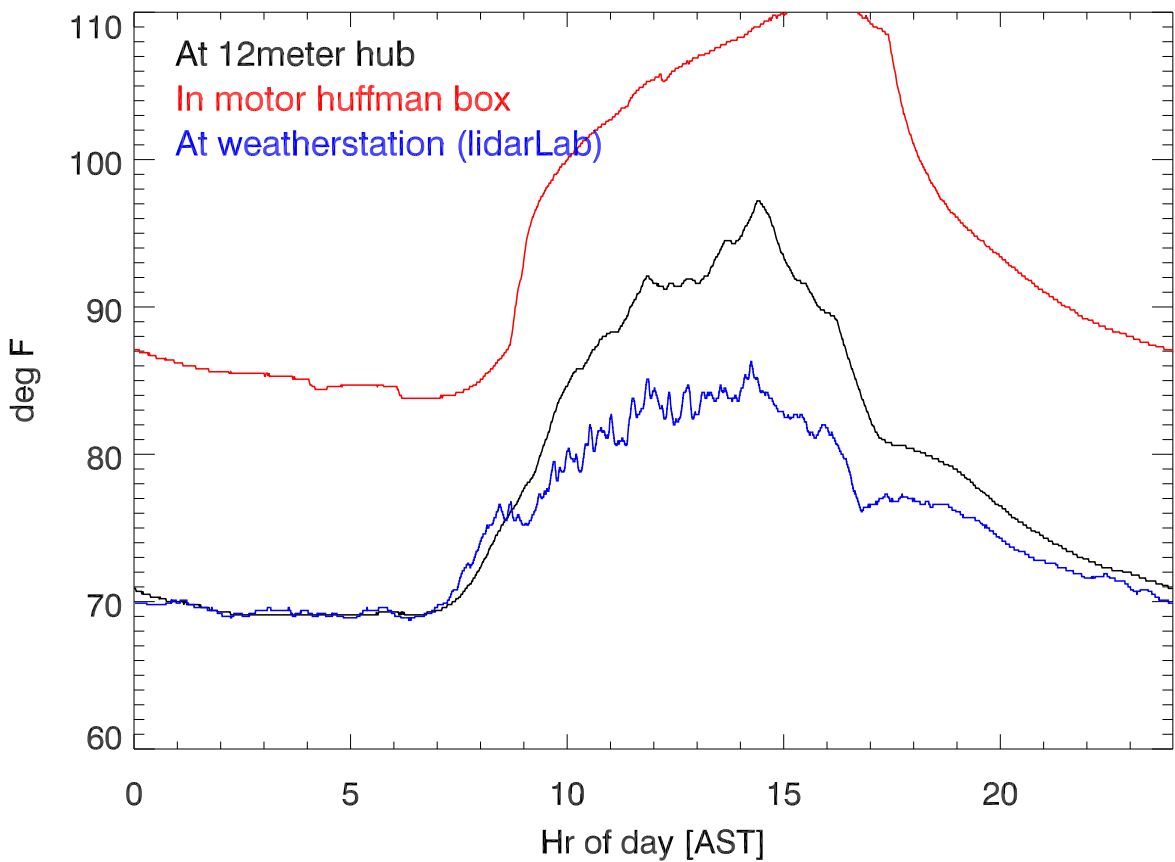
12meter and weather stations temperatures for 220418
