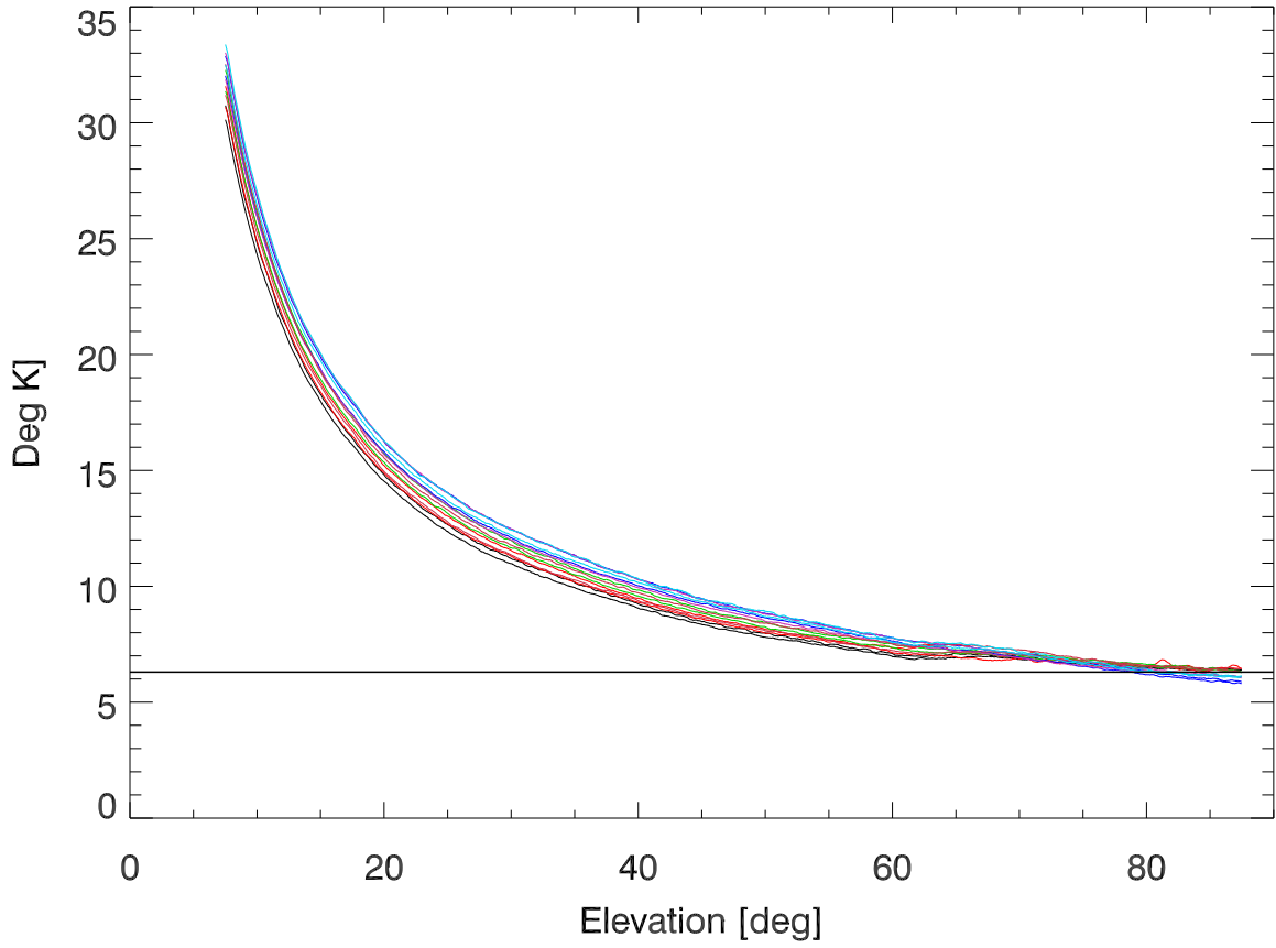
220920 (tsys - TconstFit) vs el. freqBands & PoIA,B overplotted
