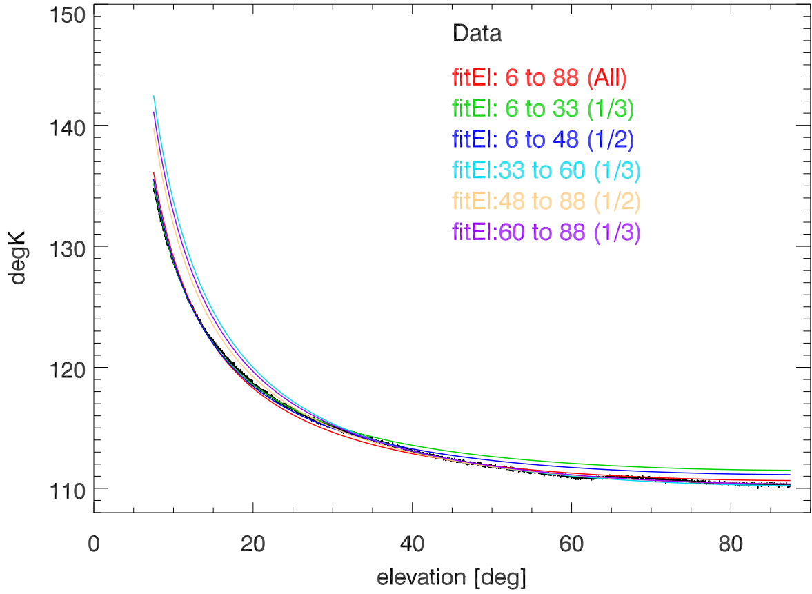
Tsys vs el using various el range fits
