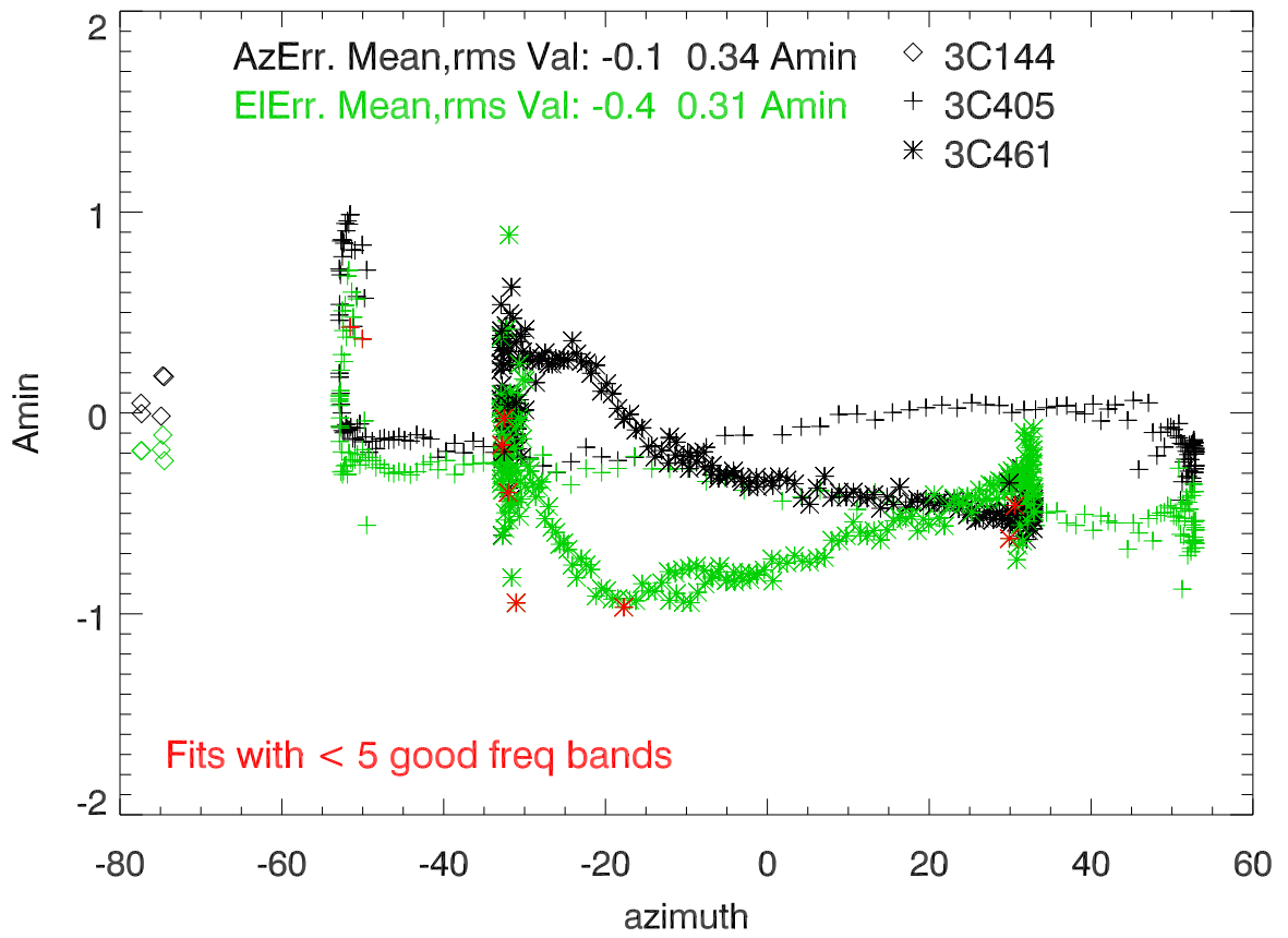
jun22 crosses.Pointing error. az,el error vs az
