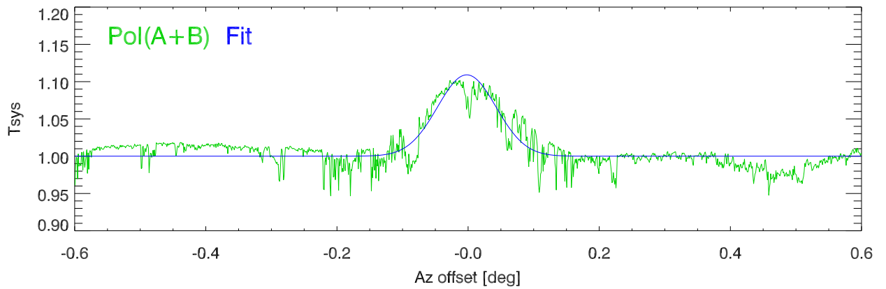
210409 Crab azStrip PoIA,B data vs offset. Pat # 6
