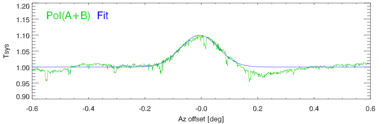
210409 Crab azStrip PoIA,B data vs offset. Pat # 4
