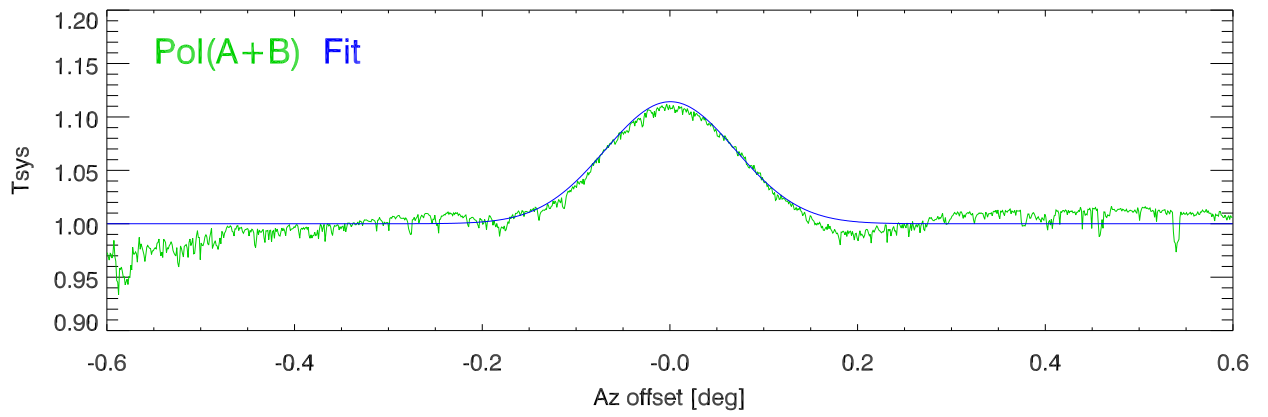
PoIA+PoIB and fit vs azoffset. Pat # 9
