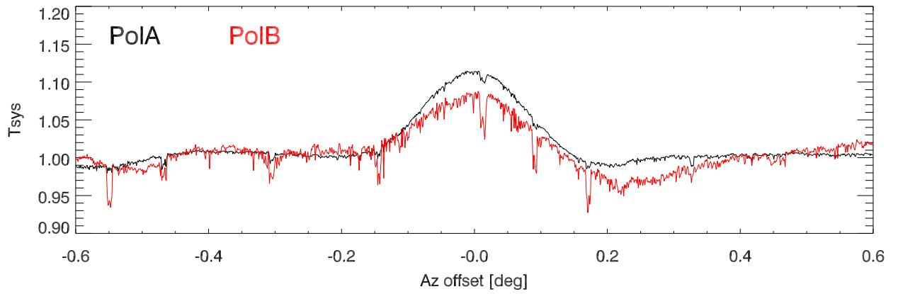
PoIA+PoIB and fit vs azoffset. Pat # 3
