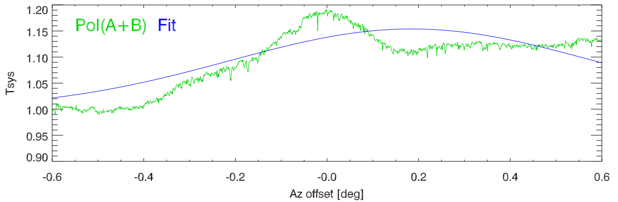
PoIA+PoIB and fit vs azoffset. Pat # 1
