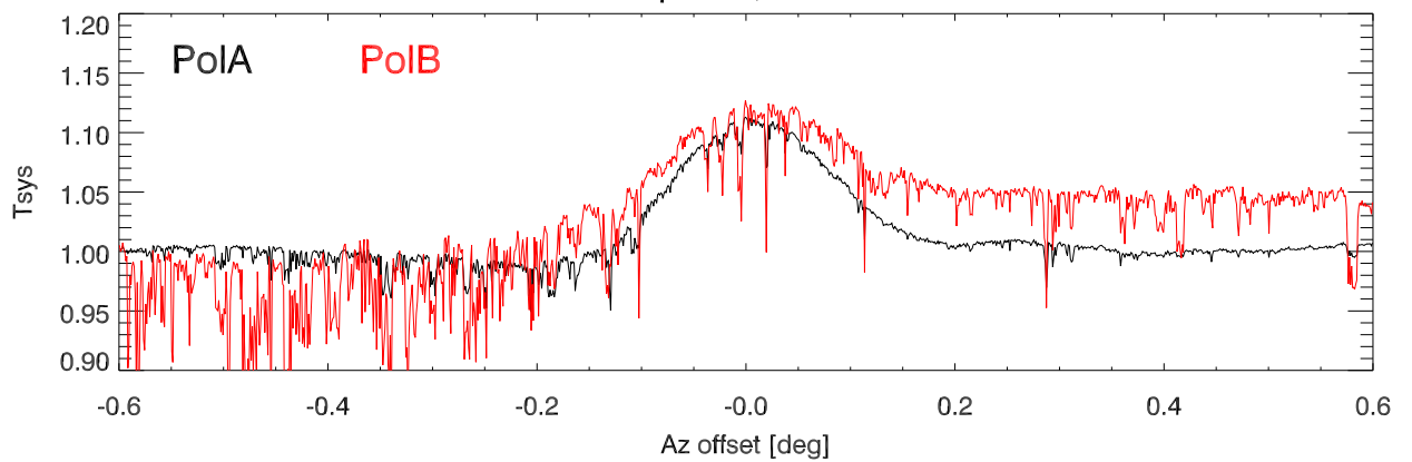
PoIA+PoIB and fit vs azoffset. Pat # 4
