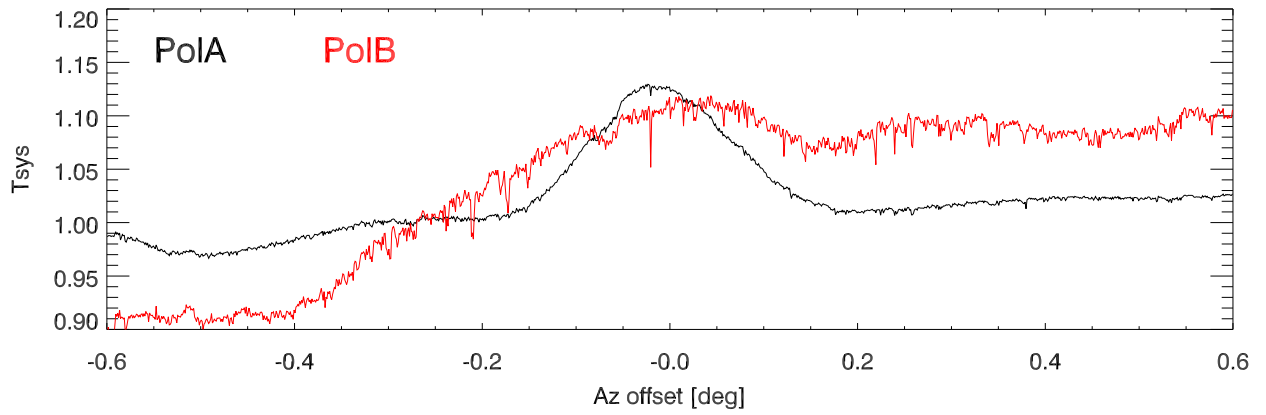
210409 Crab azStrip PoIA,B data vs offset. Pat # 1
