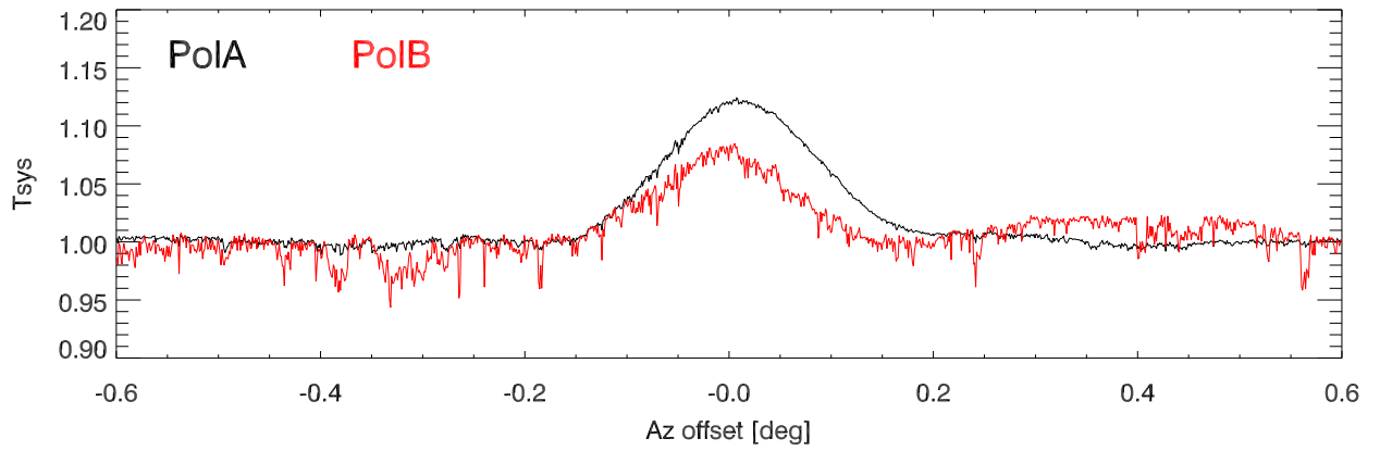
210409 Crab azStrip PoIA,B data vs offset. Pat # 7
