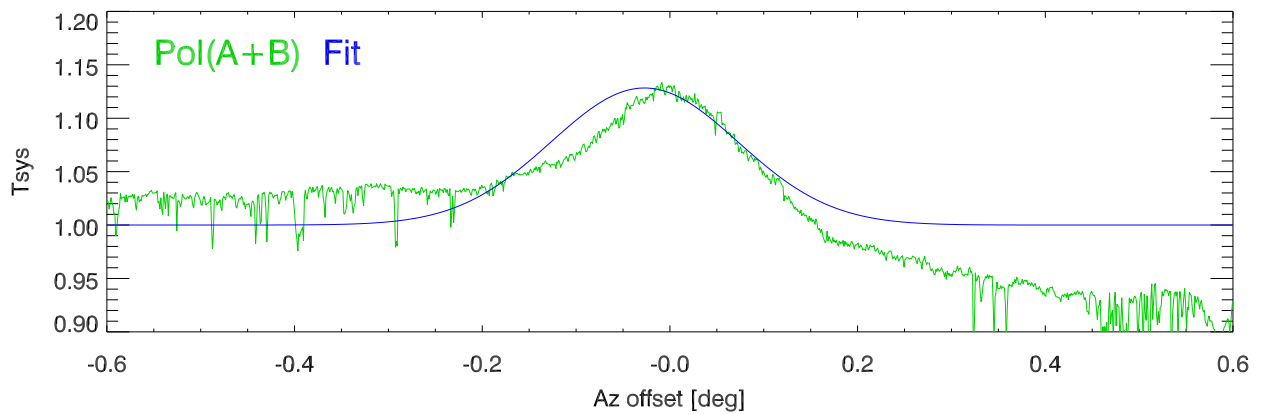
PoIA+PoIB and fit vs azoffset. Pat # 2
