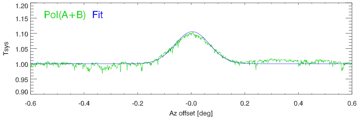
210409 Crab azStrip PoIA,B data vs offset. Pat # 8
