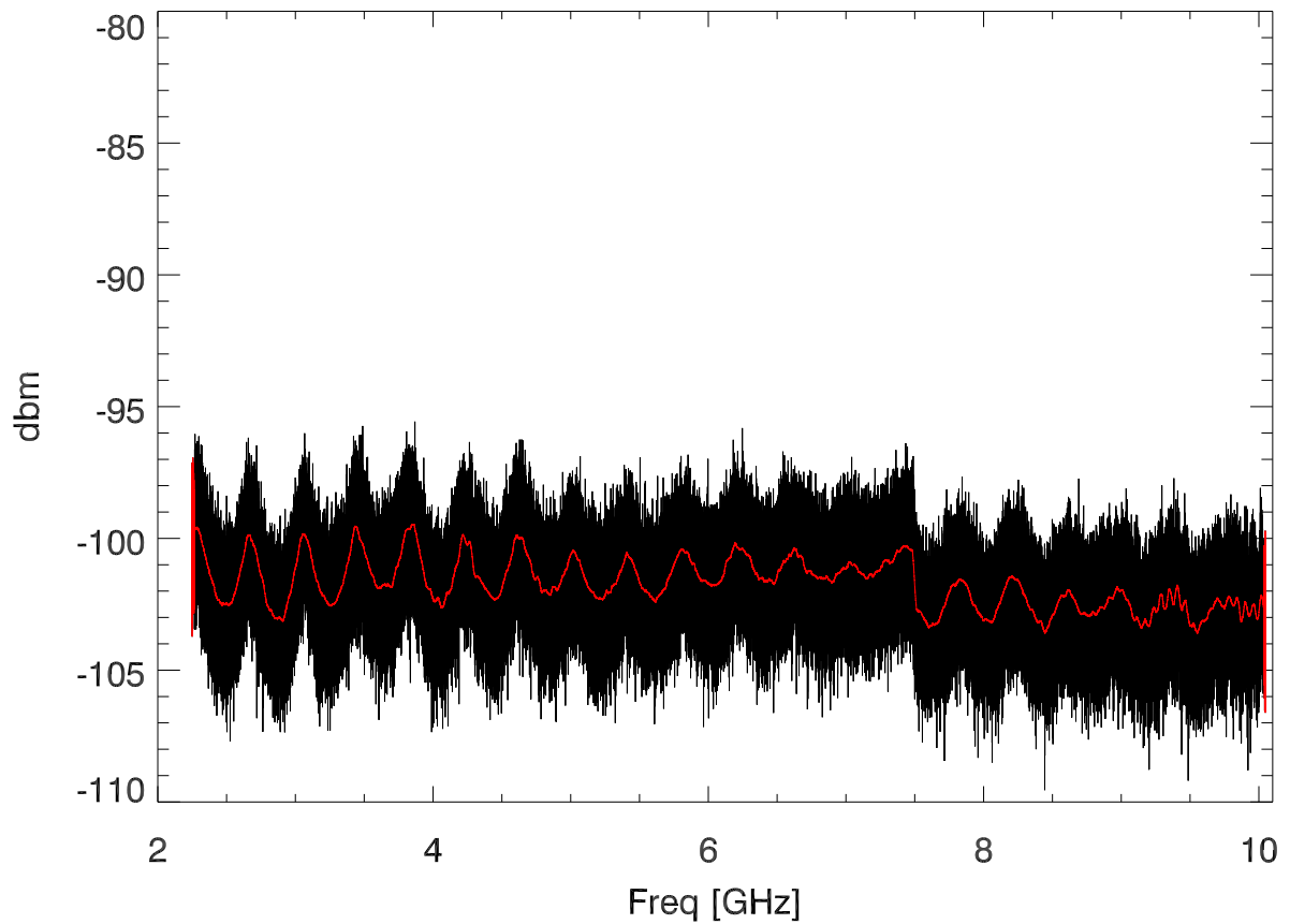
06mar23 filterbank spectra at fieldFox input. Box closed
