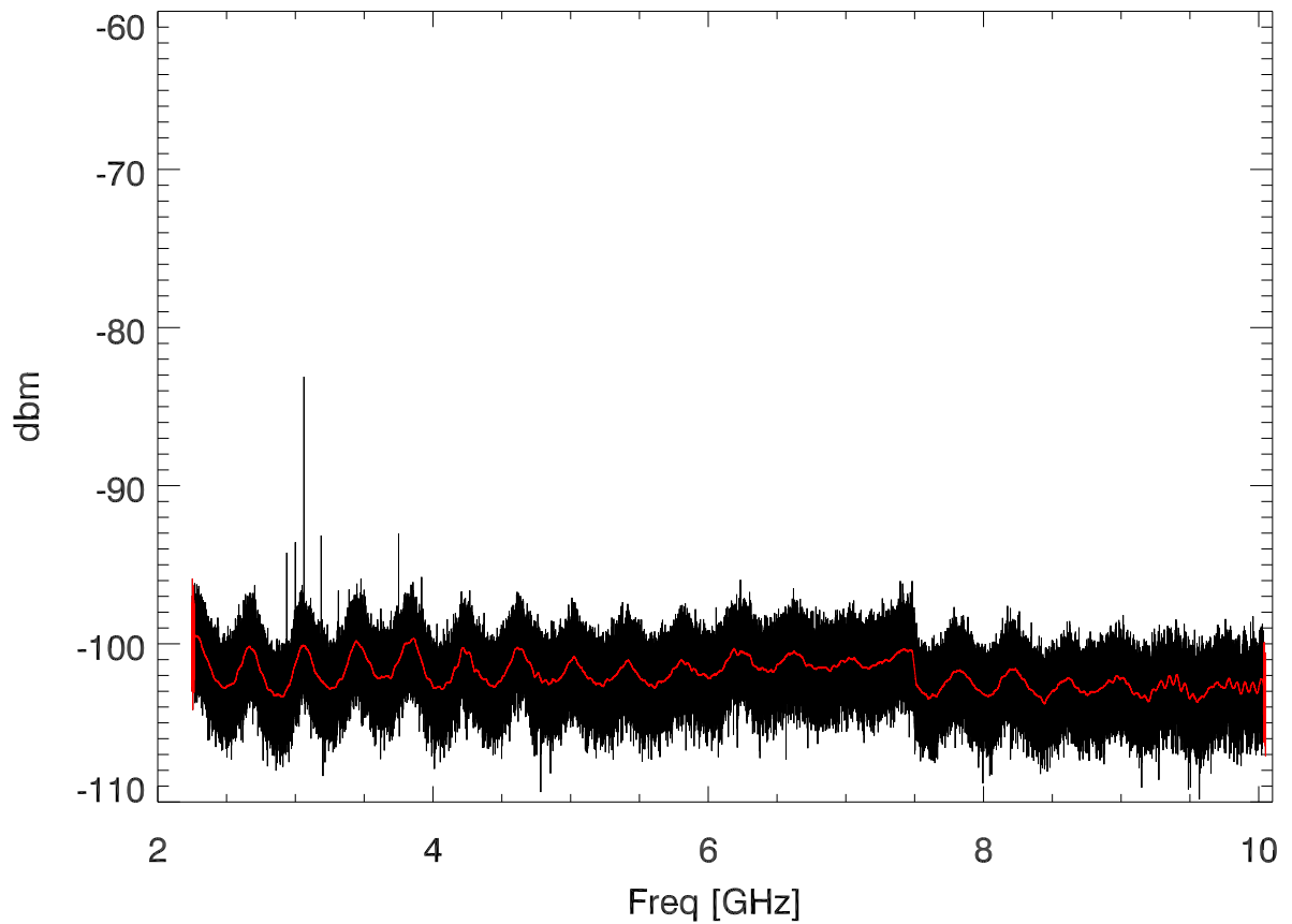
02mar23 filterbank spectra at fieldFox input. Box closed
