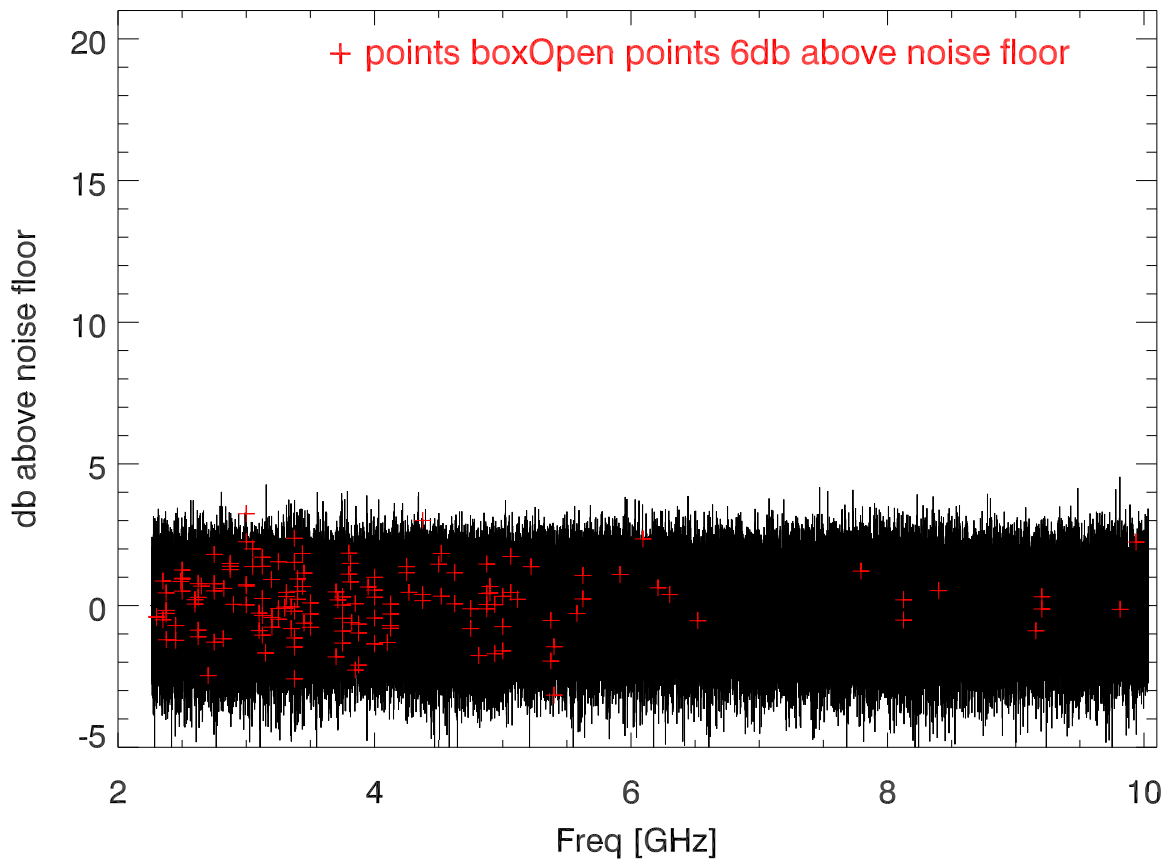
28mar23 dewMon box spectral ratio (measured/noisefloor) Box closed
