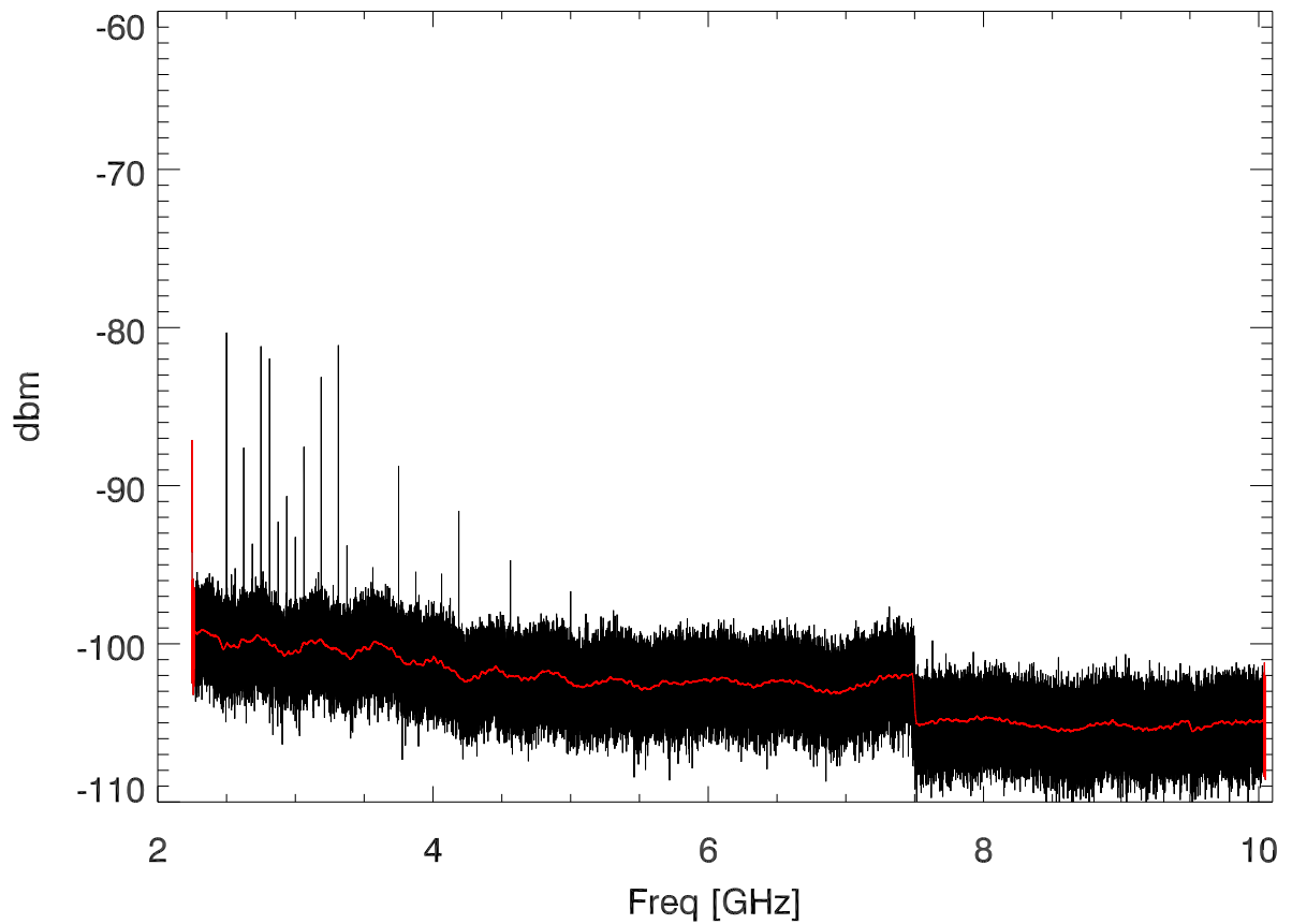
11jan23 dwMon spectra at fieldFox input. Box closed
