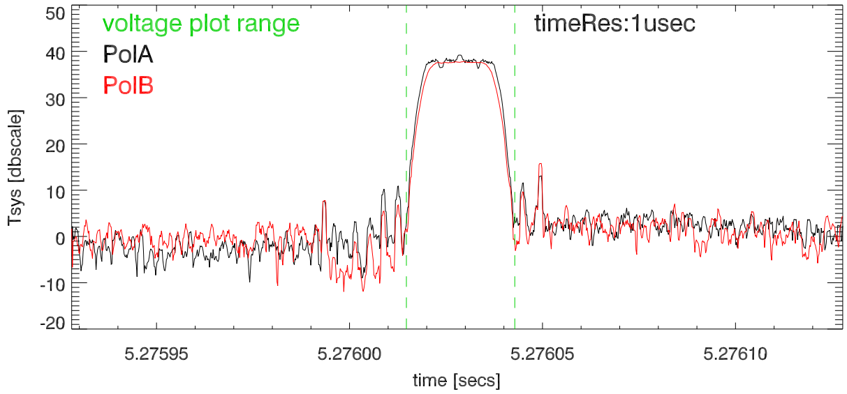
22feb23 totPwr (5mhz,cfr=8762Mhz) at rfi pk.
