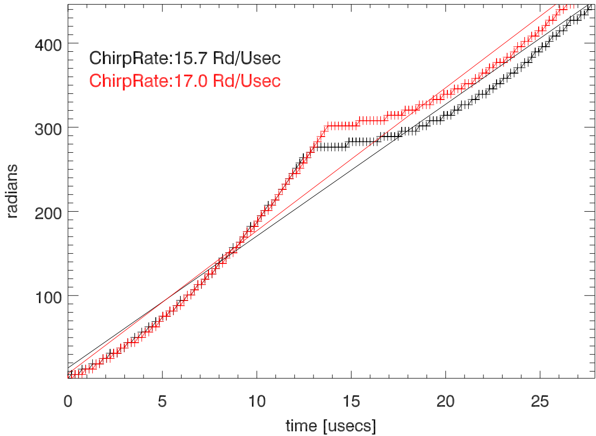
Phase vs time (and linear fits)
