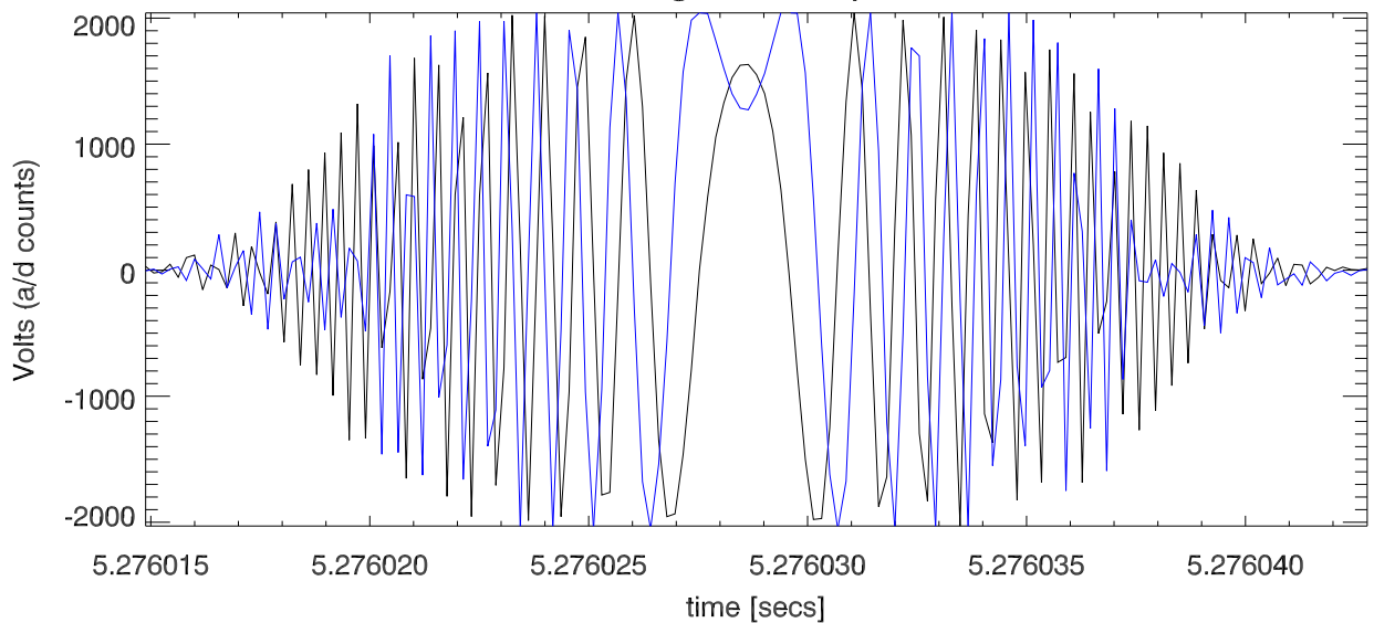
Voltage vs time. poIB
