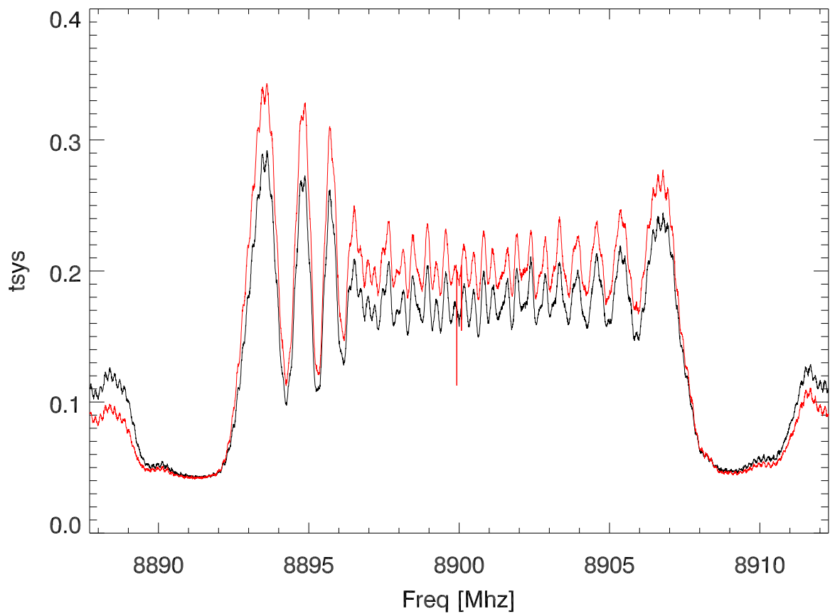
rms/mean by freq chan. 24Mhz bw, 4096 chan
