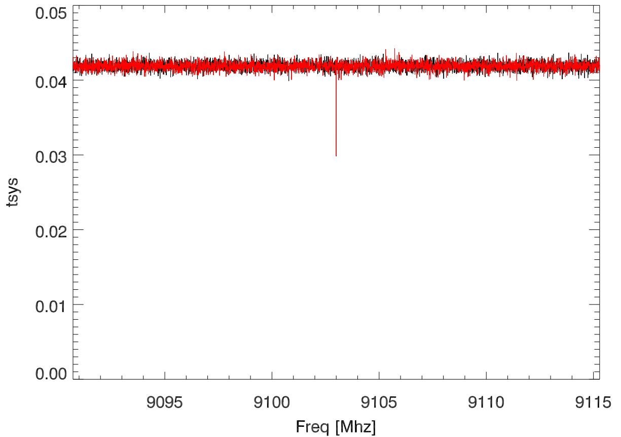
rms/mean by freq chan. 24Mhz bw, 4096 chan
