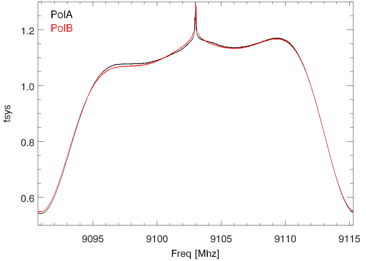
230629 spectra avg. 300 sec at 9103 Mhz. .1 sec sampling
