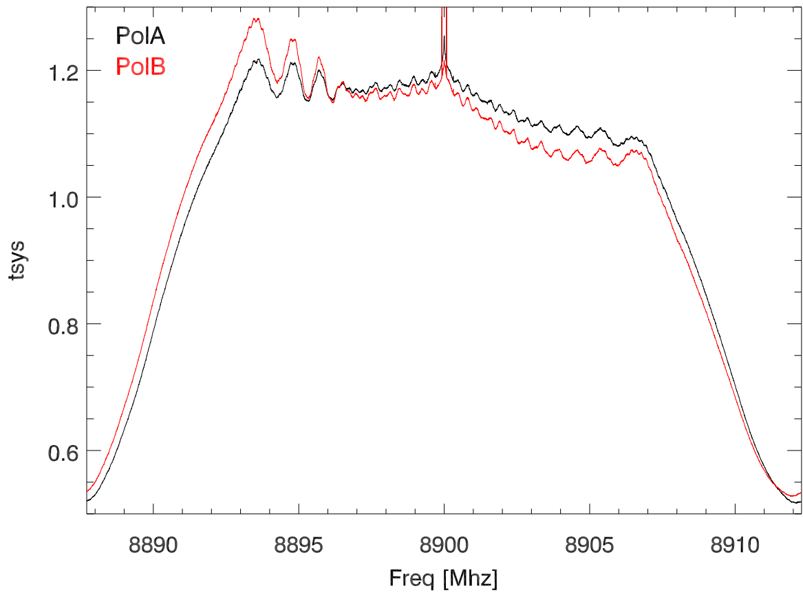
230629 spectra avg. 300 sec at 8900. Mhz. .1 sec sampling
