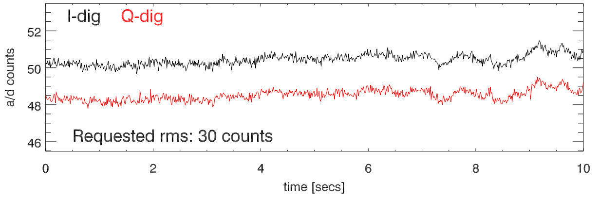
18nov22 mock voltage sampling. Voltage rms vs time. PoIA
