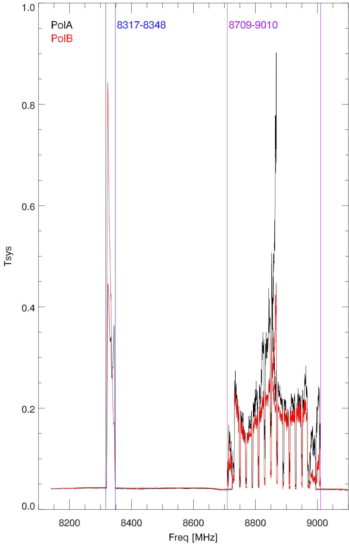
30aug22 az swing el=6. rms/mean by freq channel
