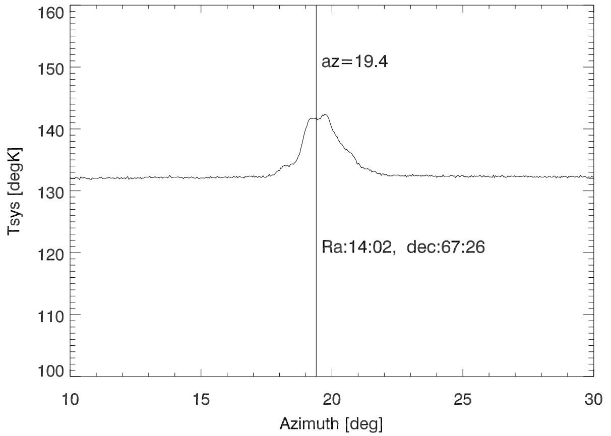
30aug22 tsys vs az blowup. el=6deg (8218Mhz Band)
