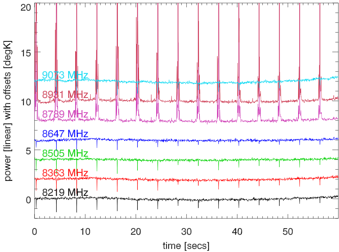
totPwr vs time for 7 freq bands (with display offsets)
