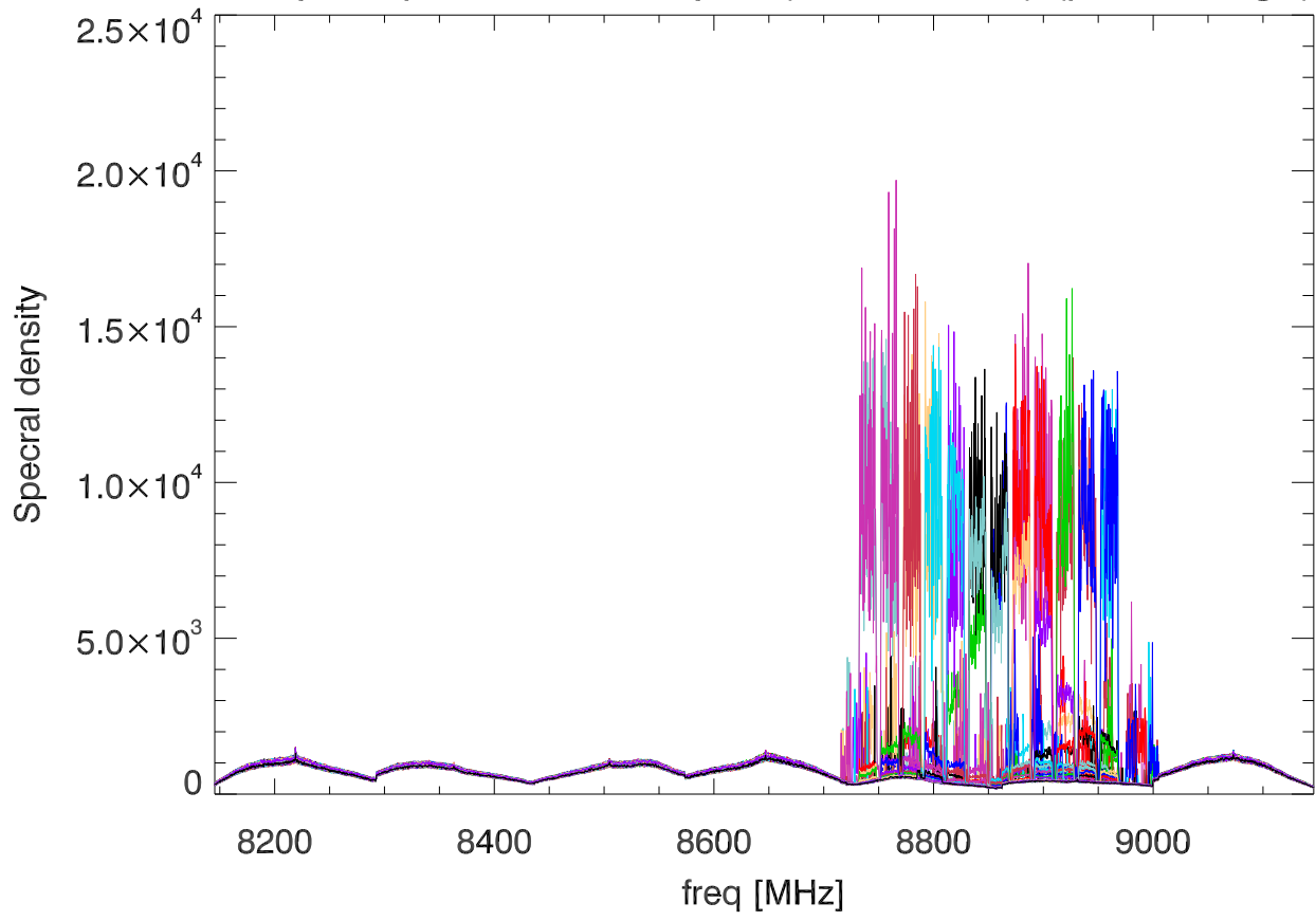
overplot spectra from strip 0. (.2 to .5 secs) (polA,B avgd)
