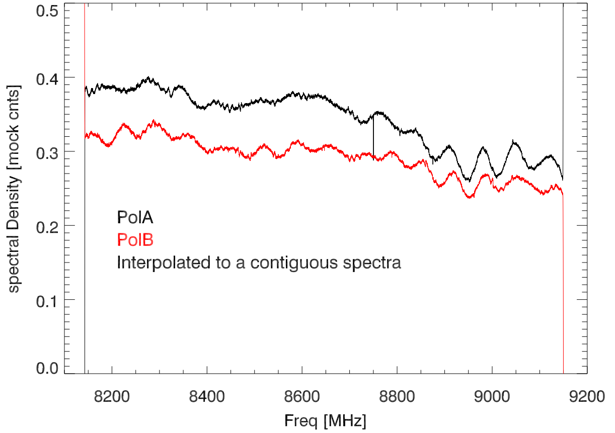
(calOn-calOff)/calOff spectra
