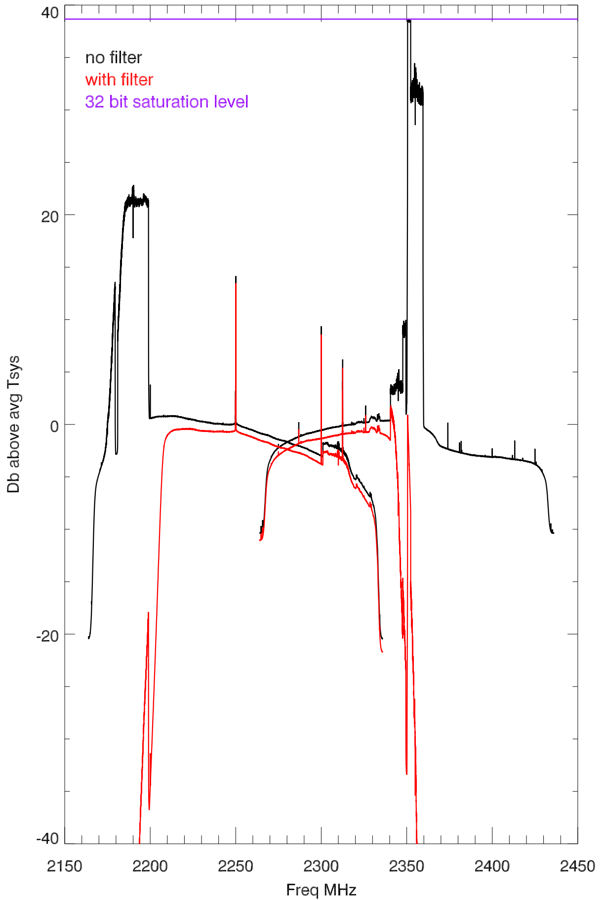
07dec21 sband spectra with mar22 filter added (in software)
