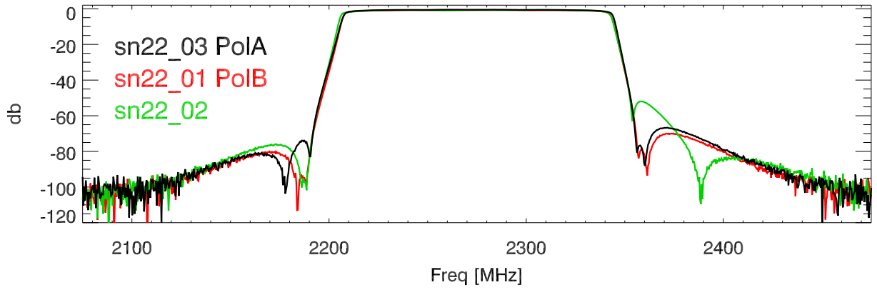
220309 S-parameters for new sband filters. S21
