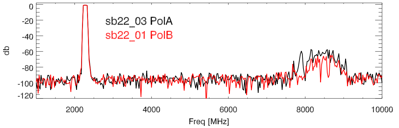
wideband S-parameters S21
